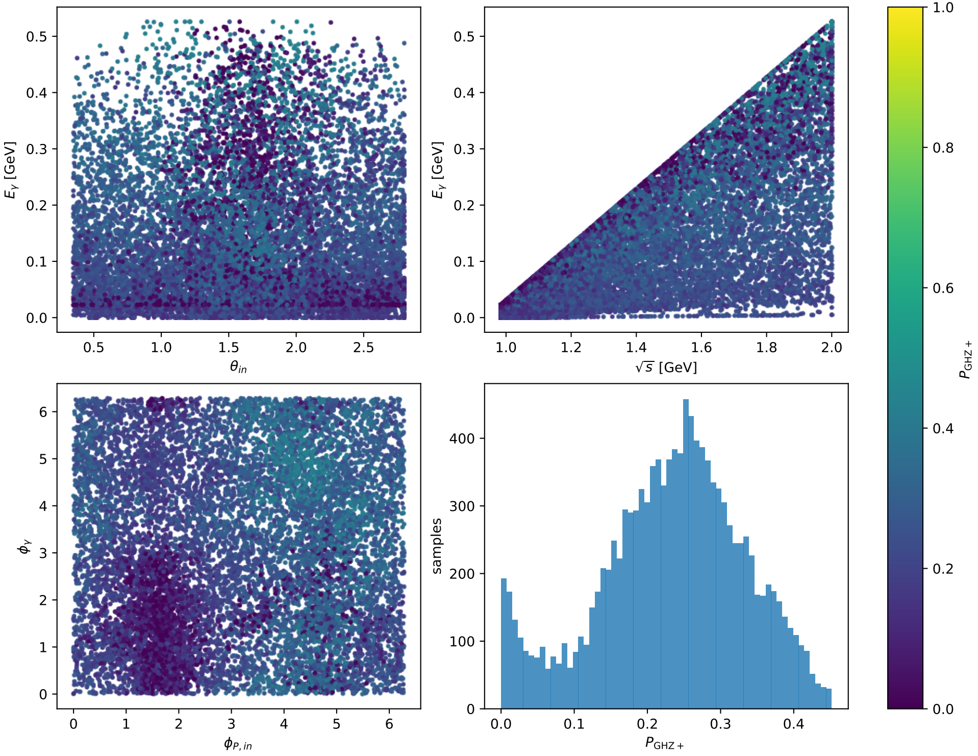
Phase-space scan: Ty proton [Ty_proton], max P_{\text{GHZ}+}=0.45193
