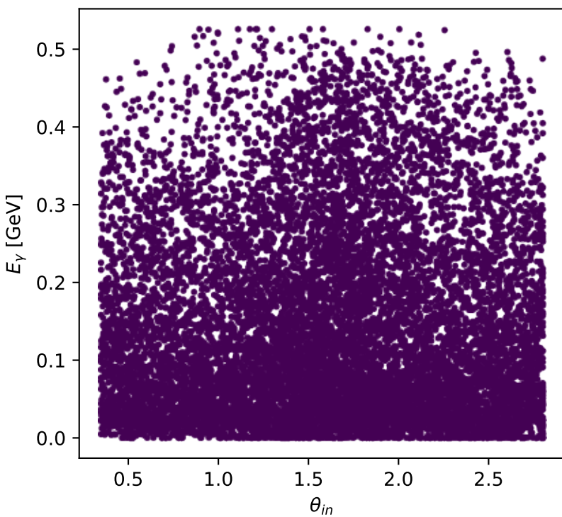
Phase-space scan: Ty proton [Ty_proton], max C_{l_0\gamma}=1.5331\text{e-13}
