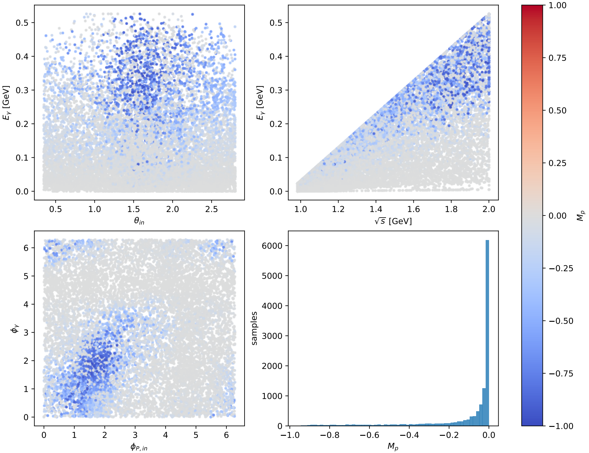
Phase-space scan: Ty proton [Ty_proton], max M_p = -3.2919\text{e-}11
