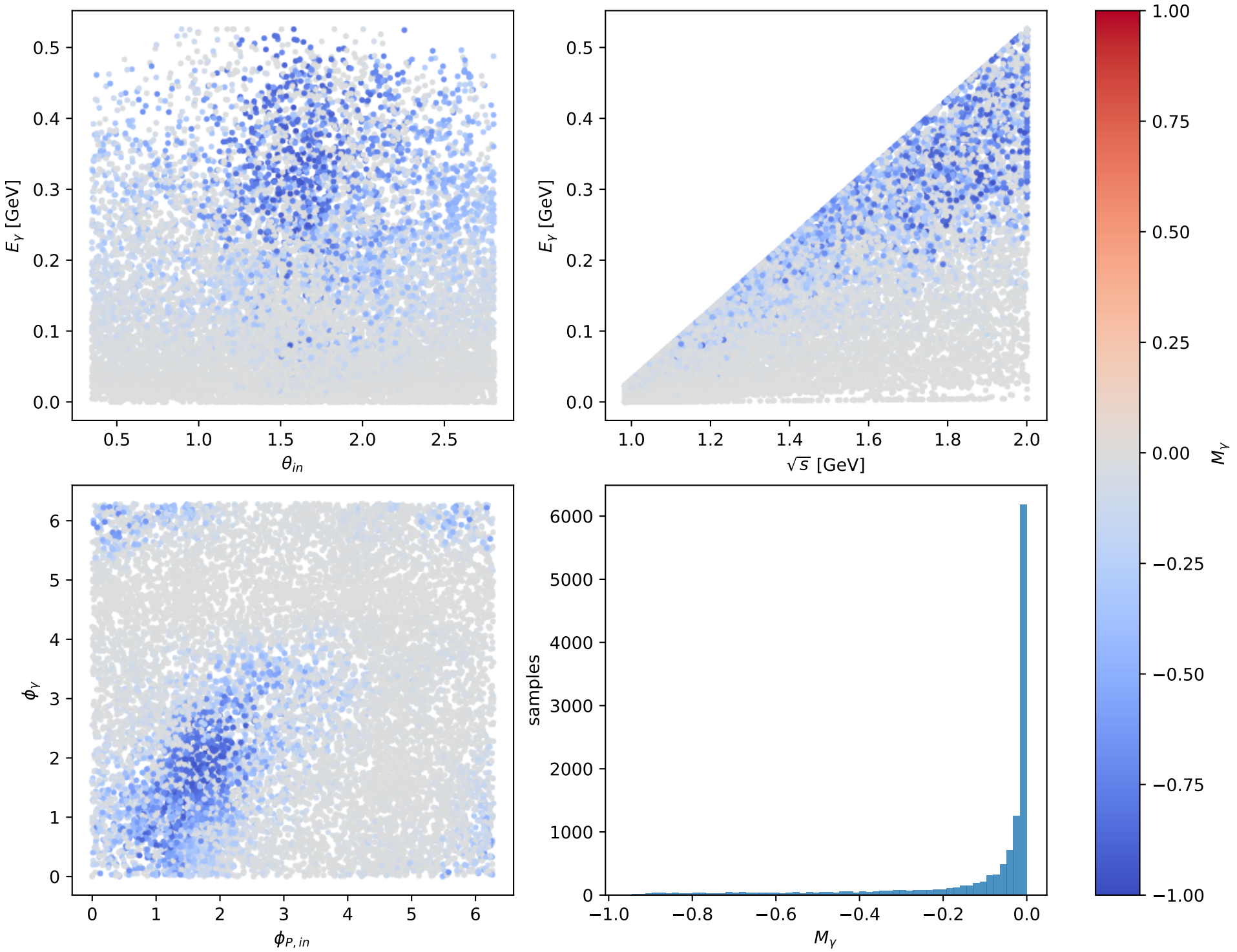
Phase-space scan: Ty proton [Ty_proton], max M_\gamma = -3.2919\text{e-}11
