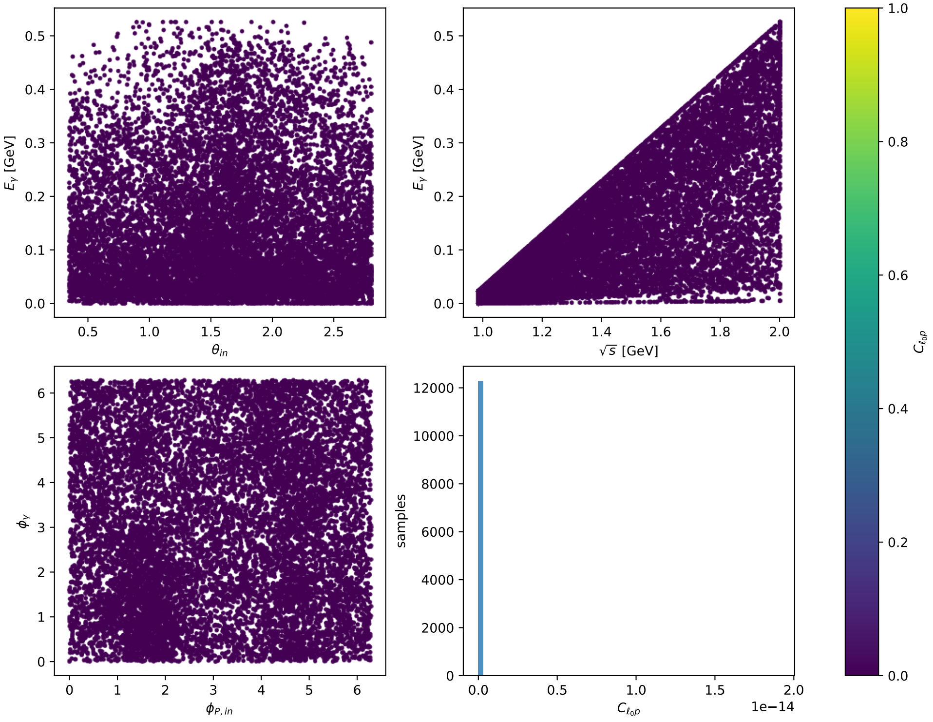
Phase-space scan: Ty proton [Ty_proton], max C_{\ell_0 p}=1.9096\text{e-14}
