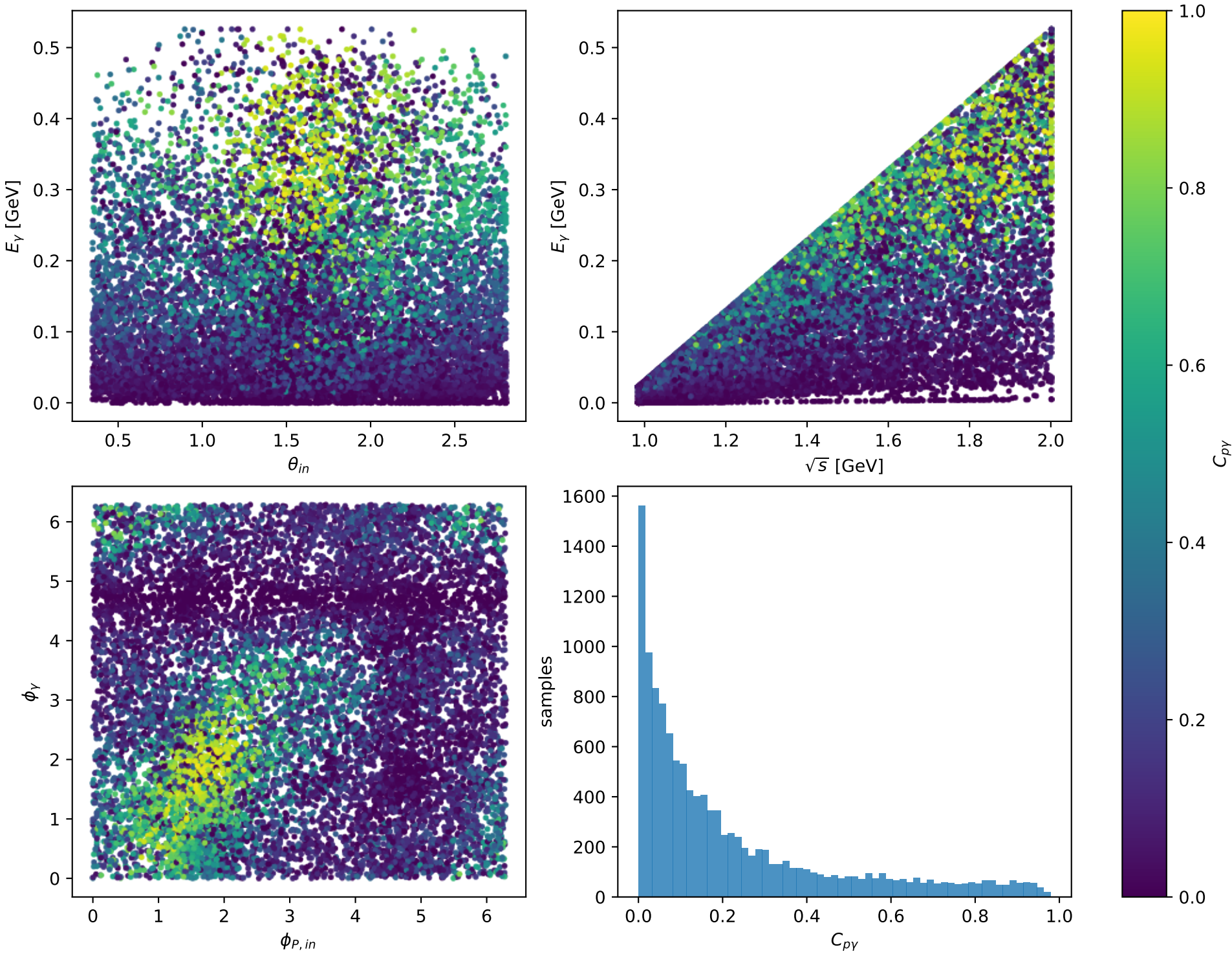
Phase-space scan: Ty proton [Ty_proton], max C_{p\gamma}=0.97971
