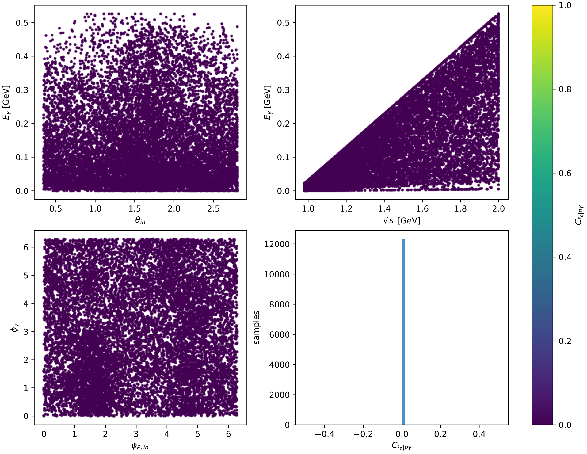
Phase-space scan: Ty proton[Ty_proton], max C_{\ell_0|p\gamma}=0
