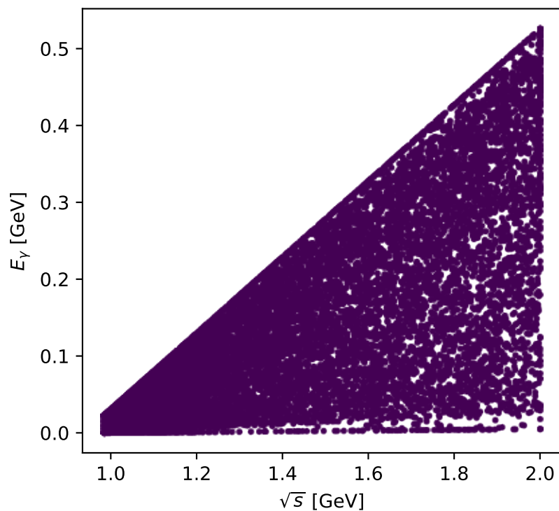
Phase-space scan: Ty proton [Ty_proton], max C_{l_0\gamma}=1.5331\text{e-13}
