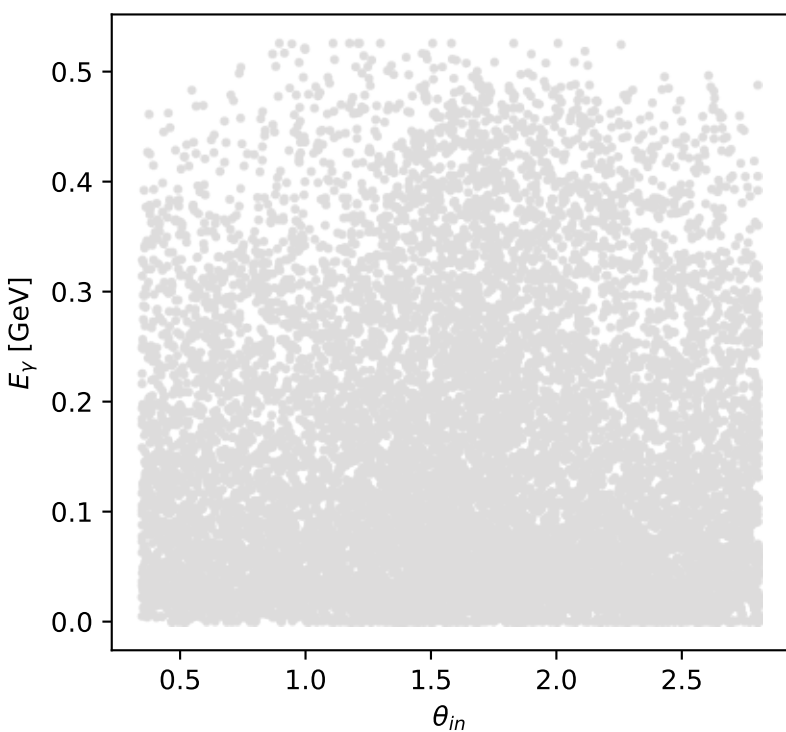
Phase-space scan: Ty proton [Ty_proton], max M_{\ell_0} = -0
