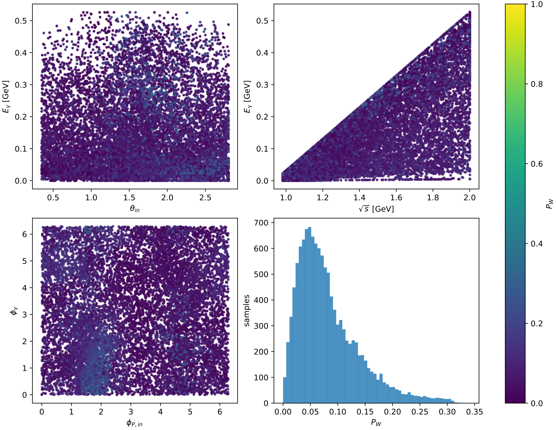
Phase-space scan: Ty proton [Ty_proton], max P_W=0.34098
