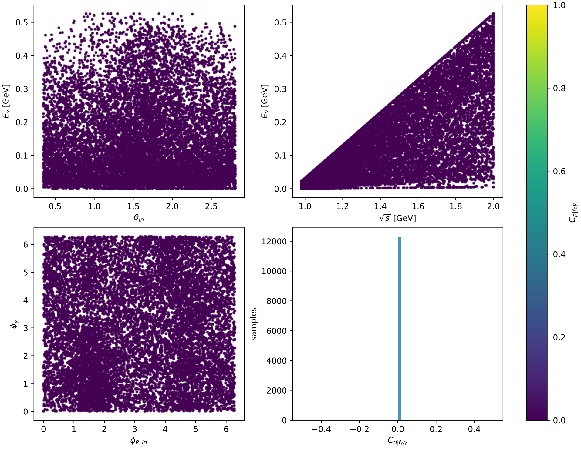
Phase-space scan: Unpolarized [unpolarized], max C_{p|\ell_0\gamma}=0
