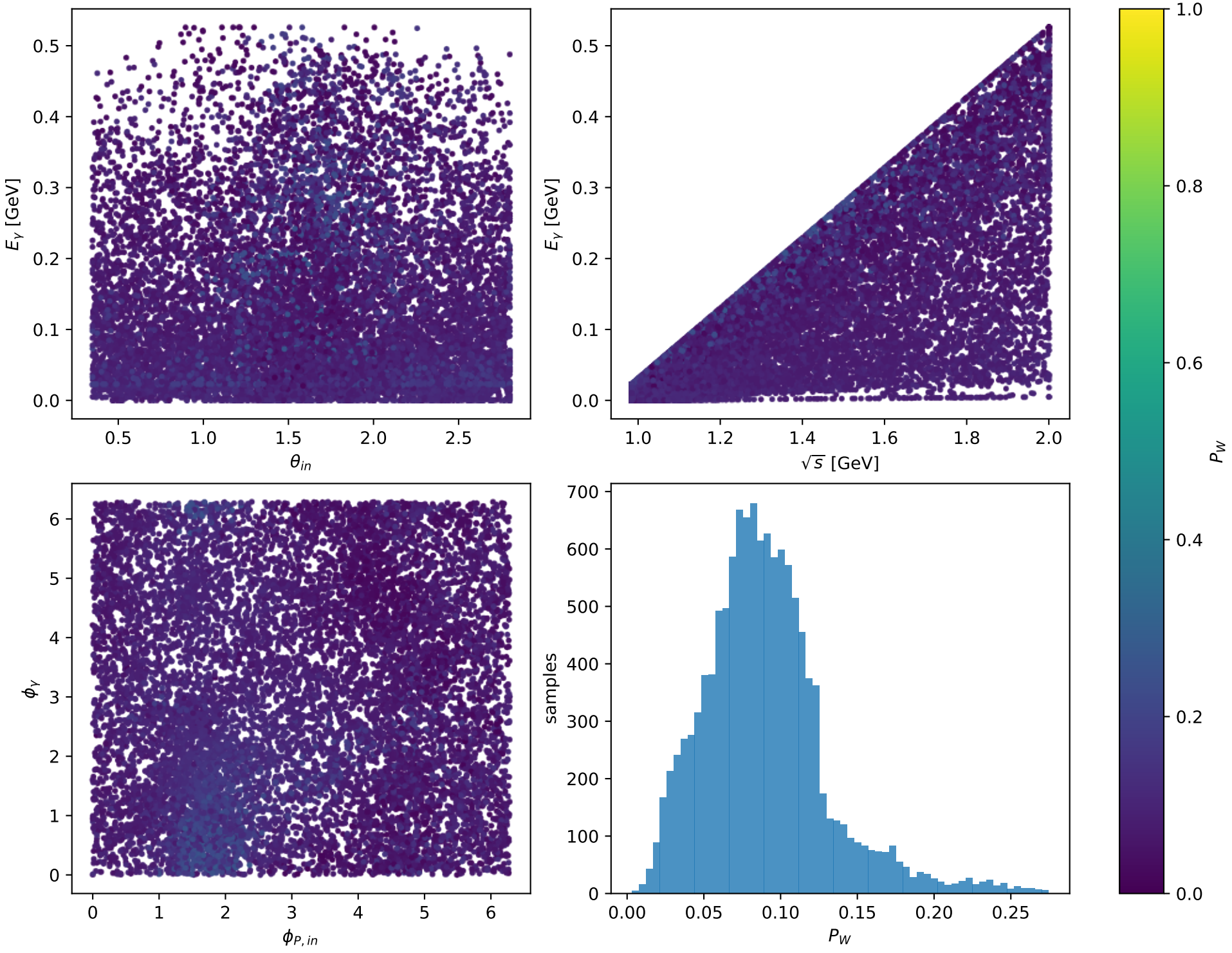
Phase-space scan: Unpolarized [unpolarized], max P_W=0.27477
