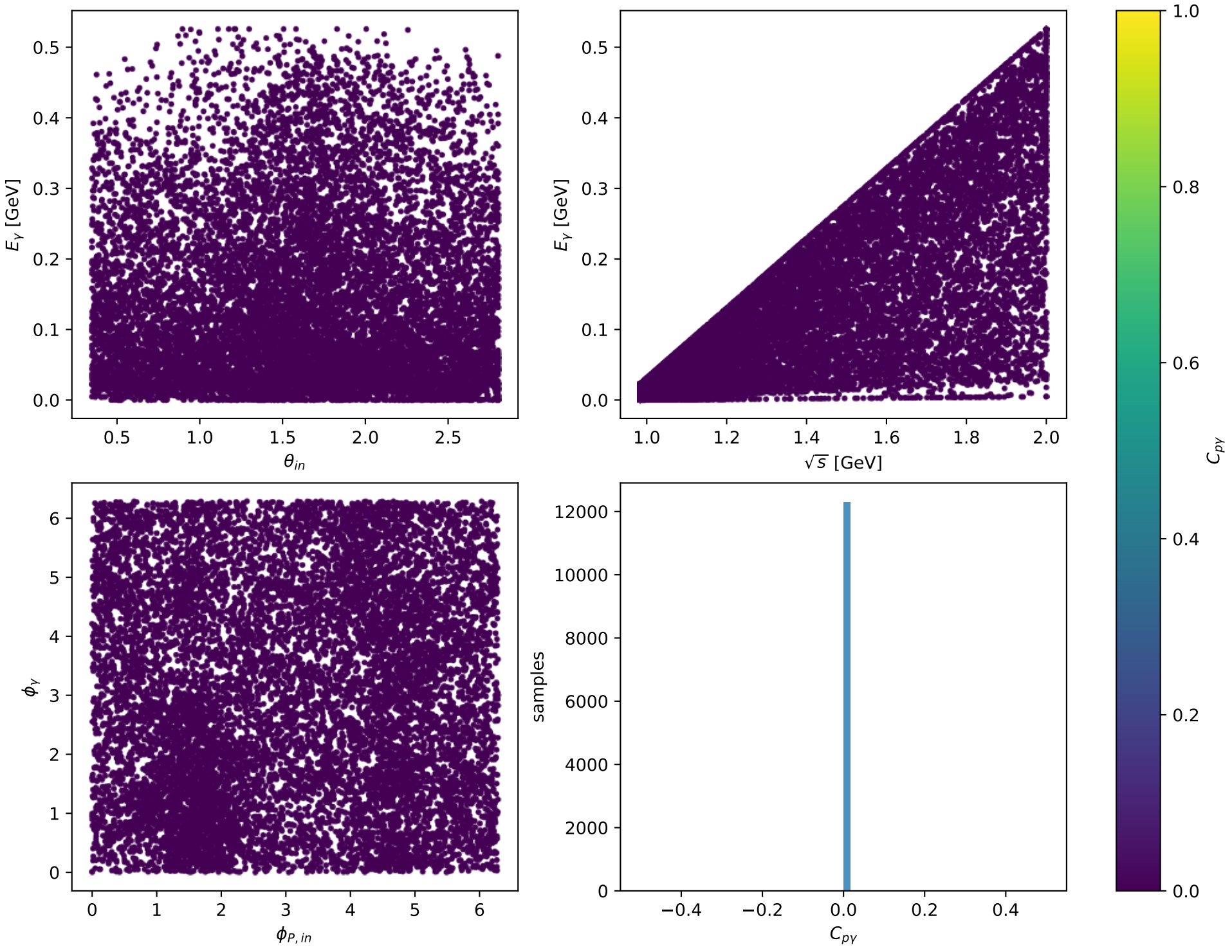
Phase-space scan: Unpolarized [unpolarized], max C_{p\gamma}=0
