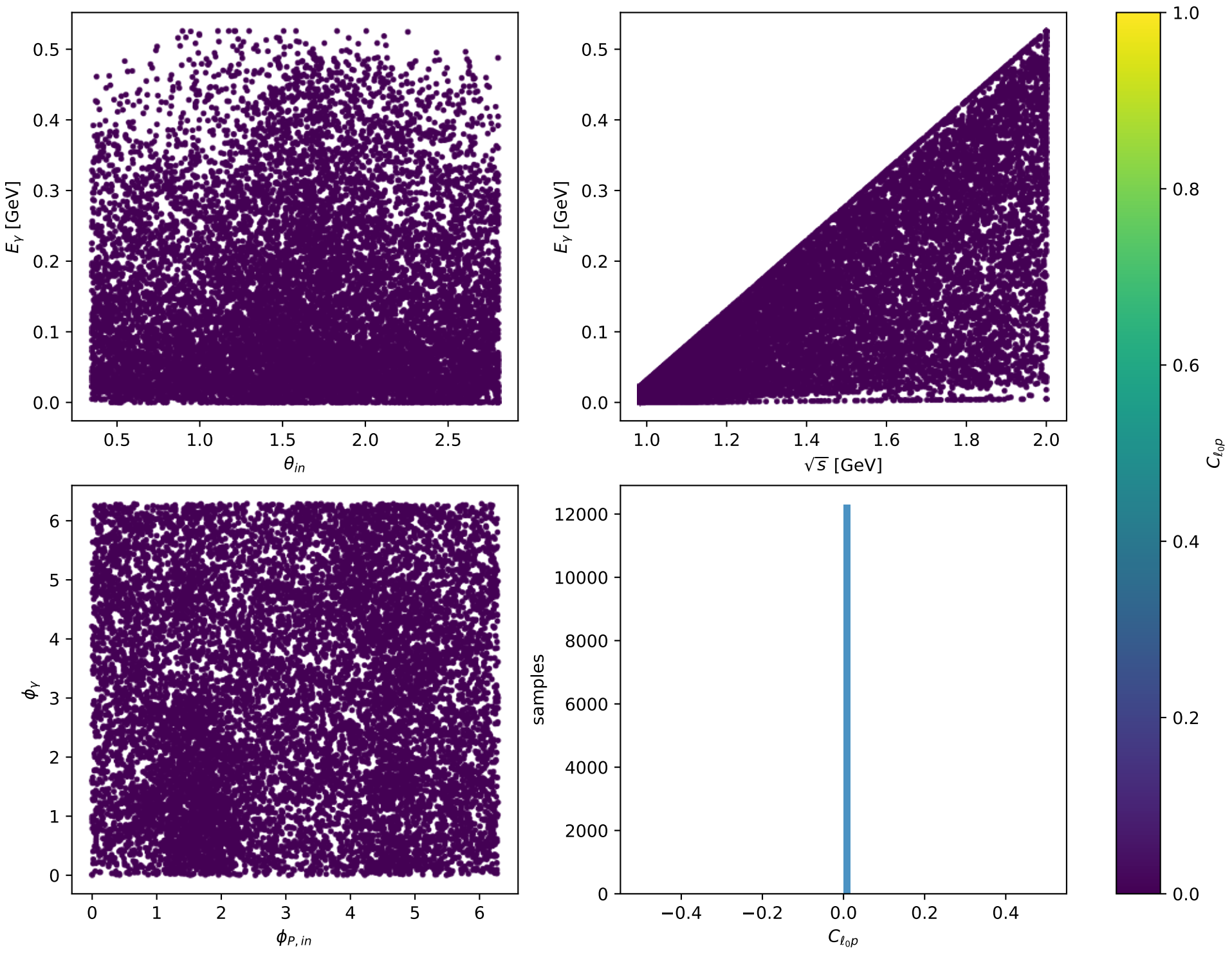
Phase-space scan: Unpolarized [unpolarized], max C_{\ell_{0p}}=0
