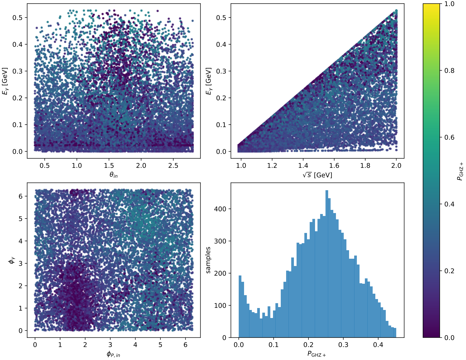
Phase-space scan: Unpolarized [unpolarized], max P_{\text{GHZ}+}=0.45193
