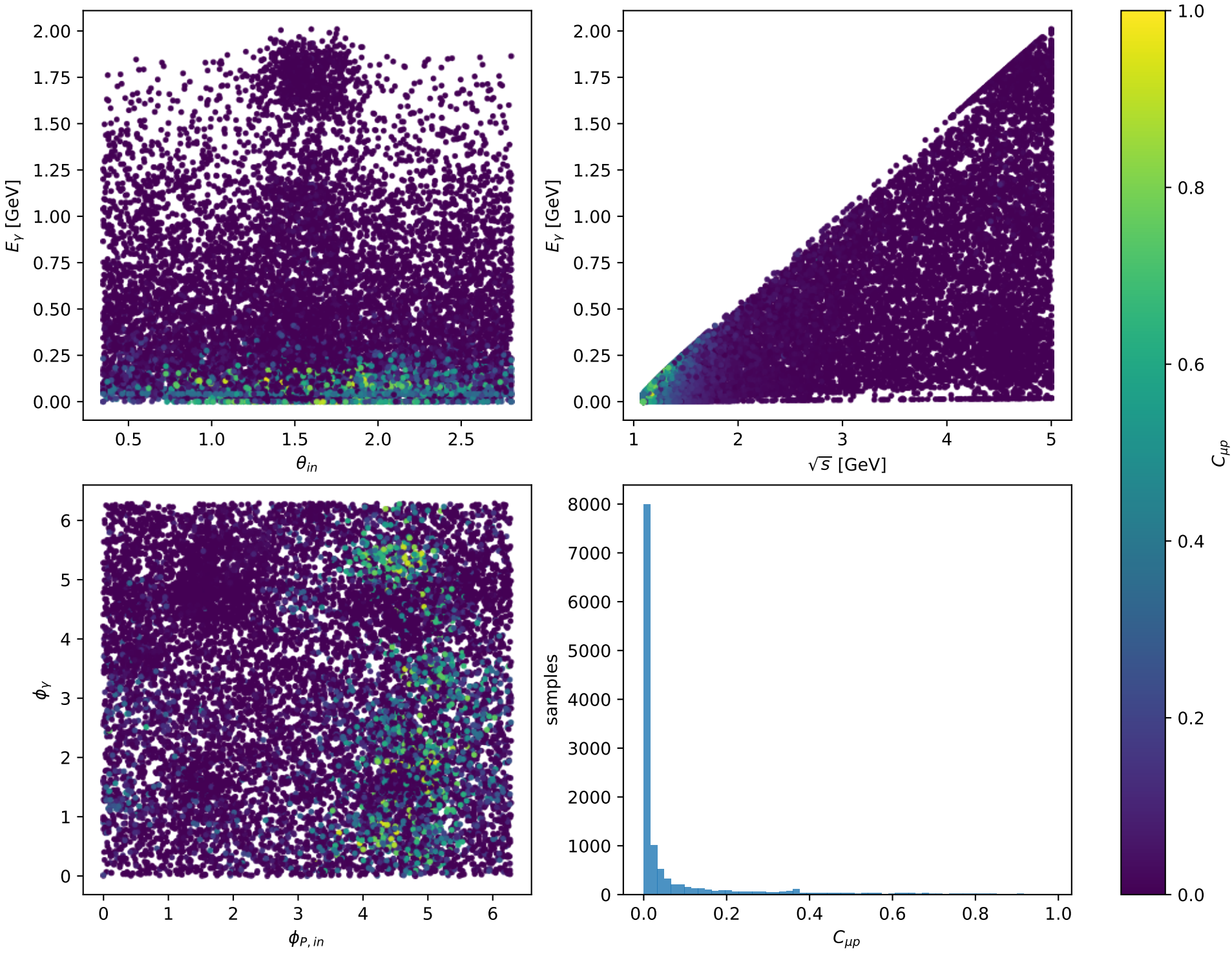
Phase-space scan: L muon + L proton [LL], max C_{\mu p}=0.98291
