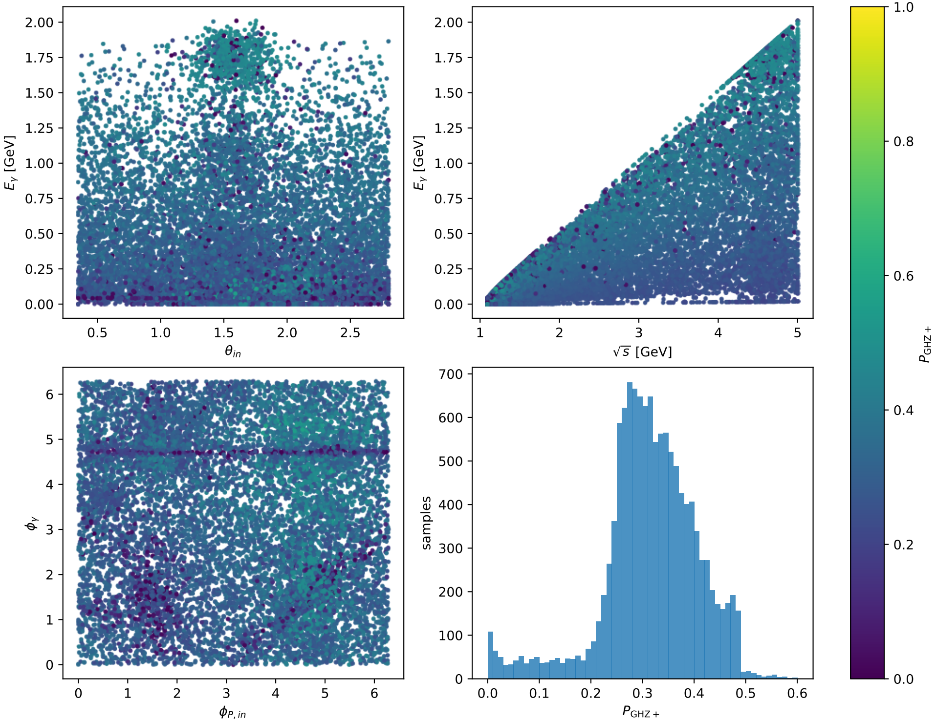
Phase-space scan: L muon + L proton [LL], max P_{\text{GHZ}+}=0.60059
