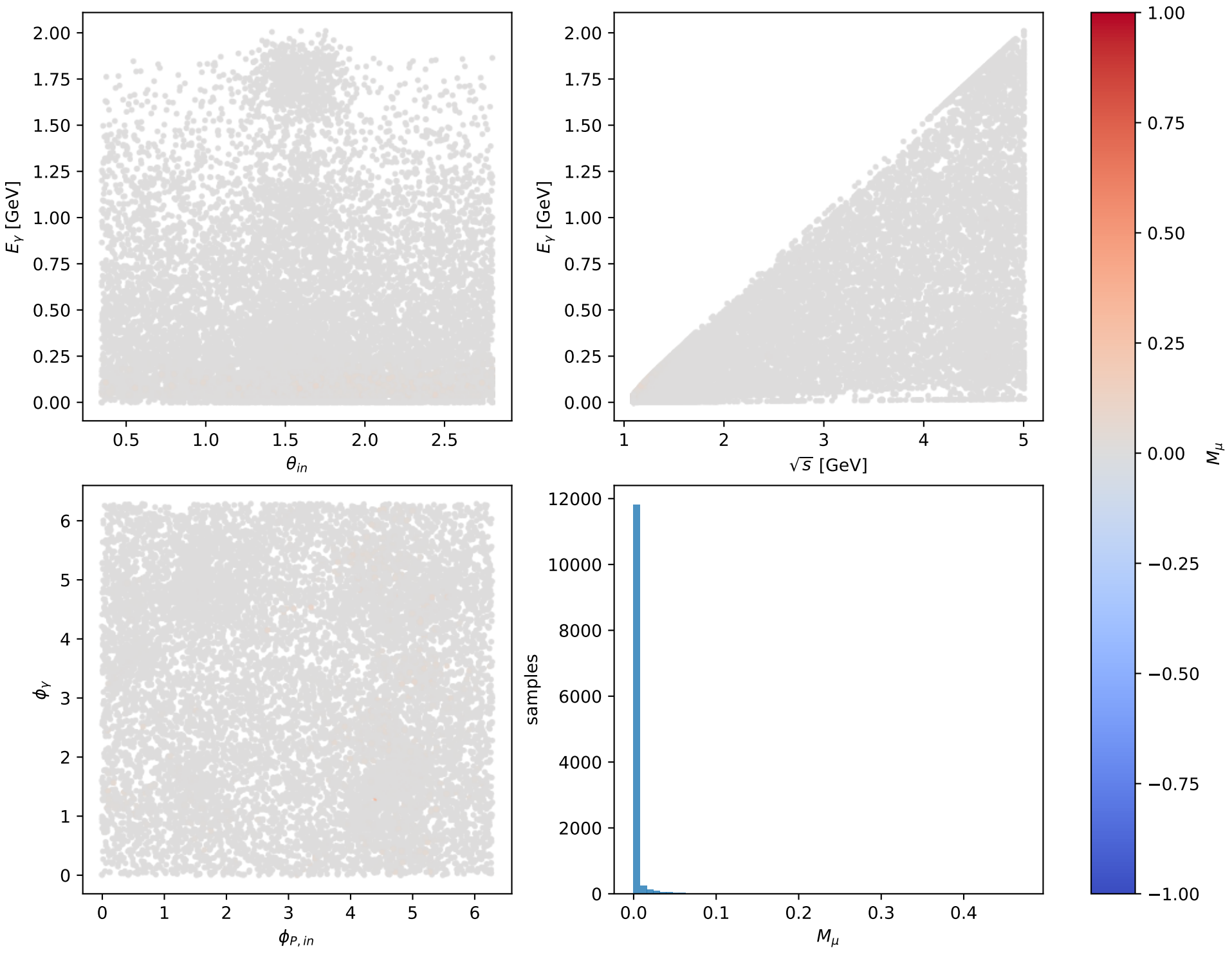
Phase-space scan: L muon + L proton [LL], max M_\mu=0.47258
