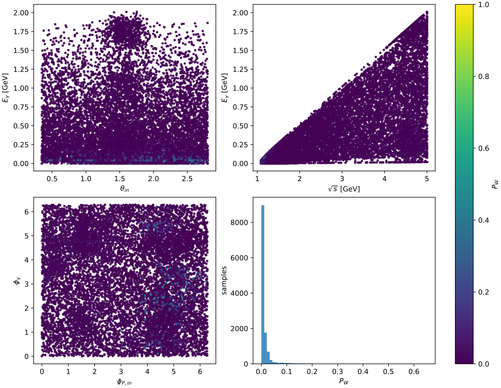
Phase-space scan: L muon + L proton [LL], max P_W=0.65114
