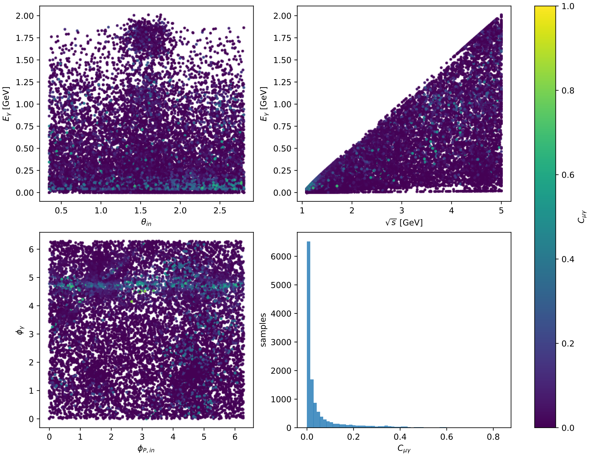
Phase-space scan: L muon + L proton [LL], max C_{\mu\gamma}=0.83455
