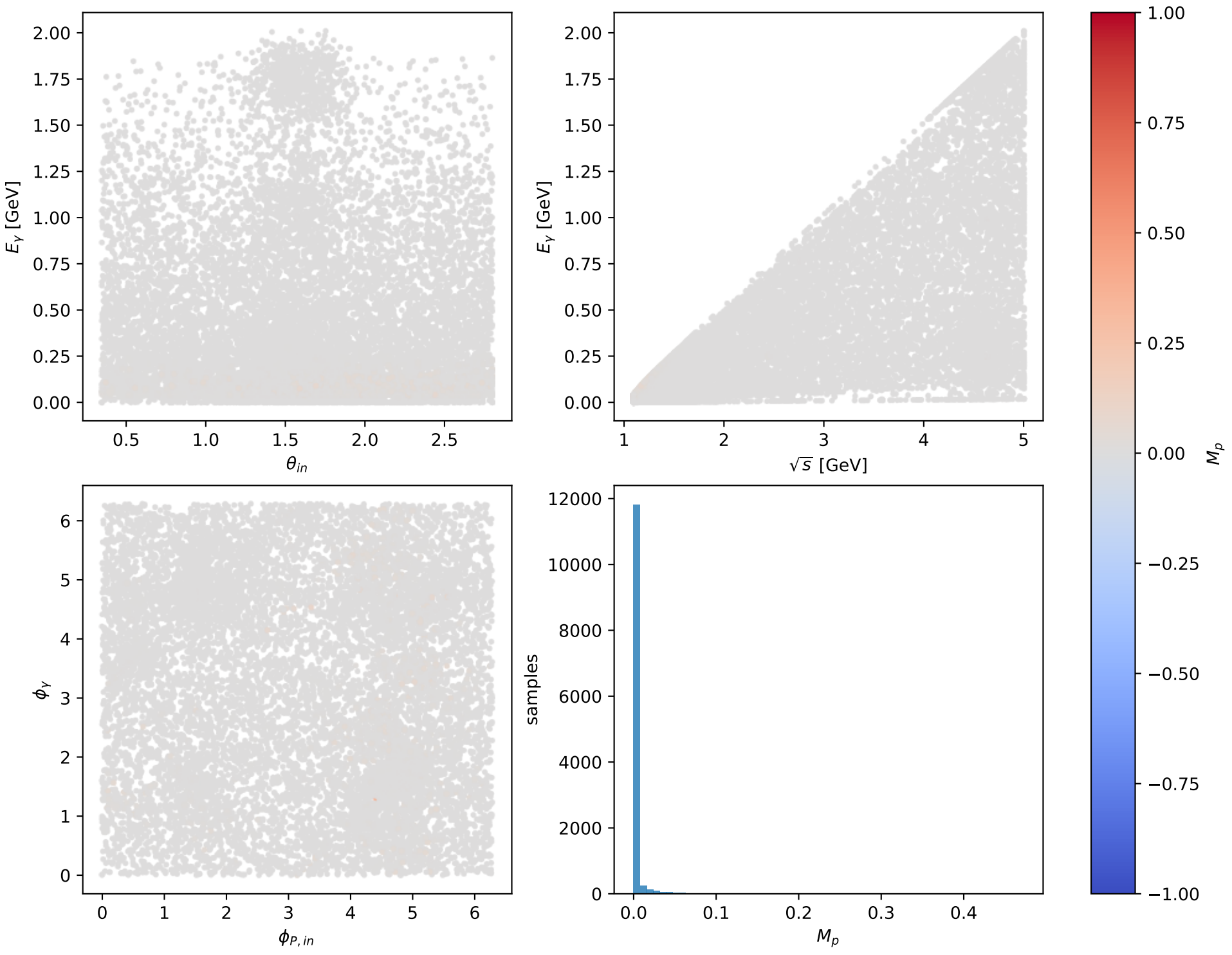
Phase-space scan: L muon + L proton [LL], max M_p=0.47258
