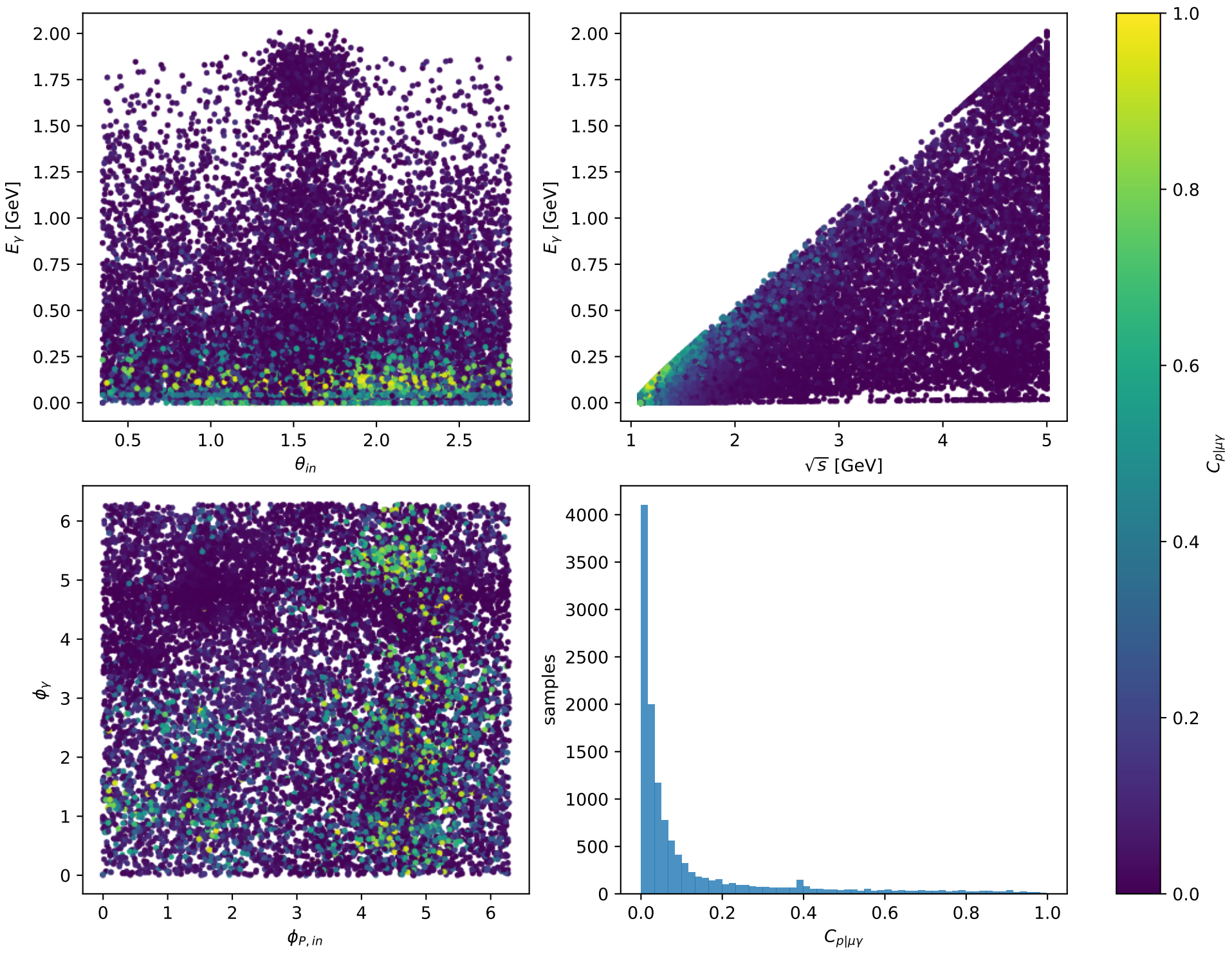
Phase-space scan: L muon + L proton [LL], max C_{p|\mu\gamma}=0.99847
