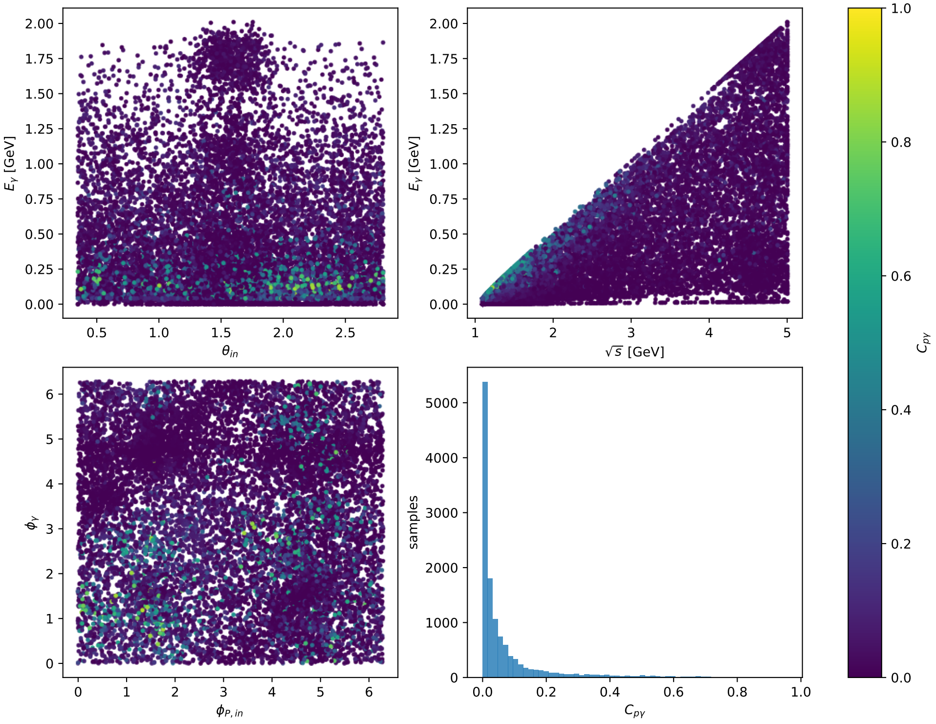
Phase-space scan: L muon + L proton [LL], max C_{py}=0.95678
