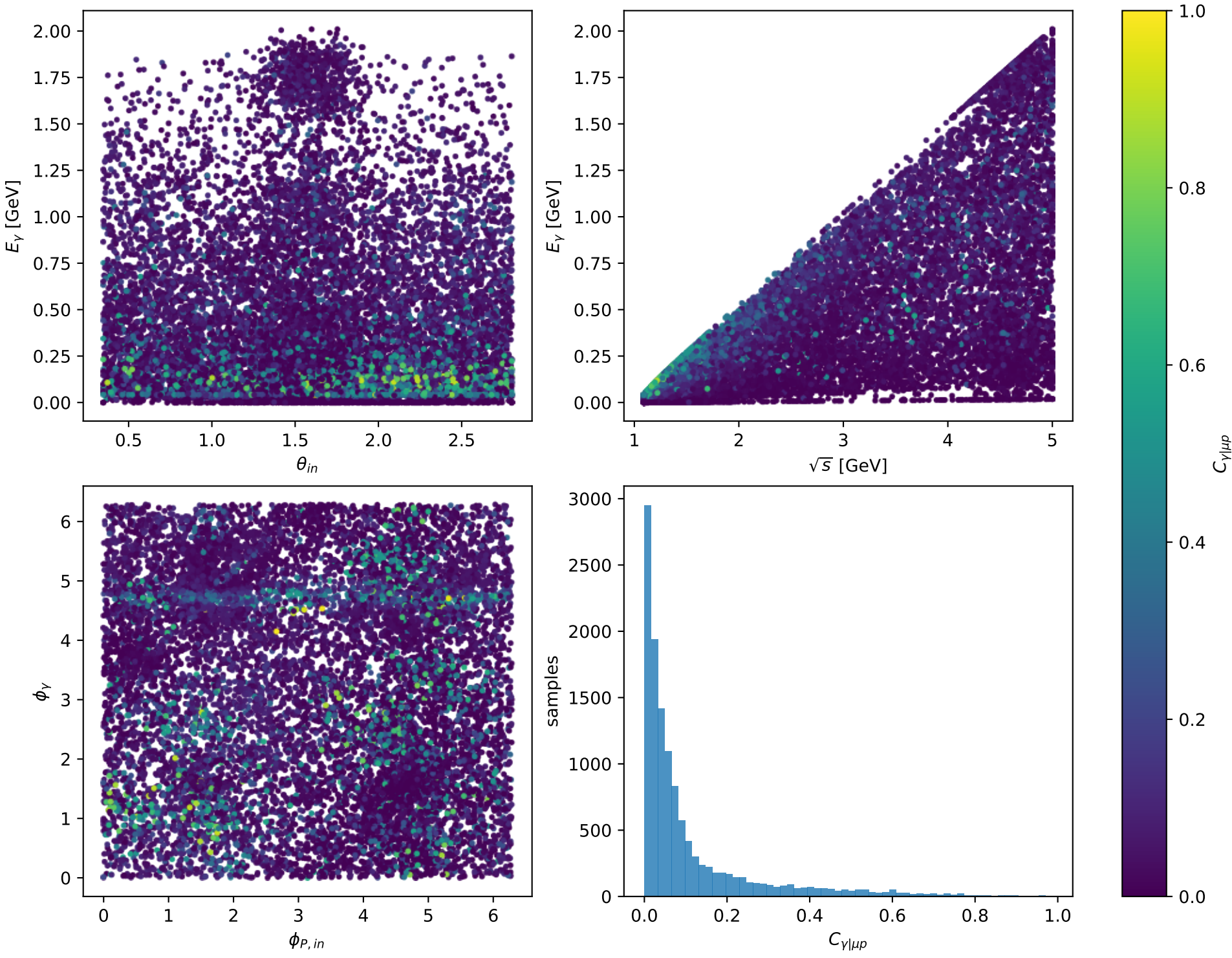
Phase-space scan: L muon + L proton [LL], max C_{\gamma|\mu p}=0.98692
