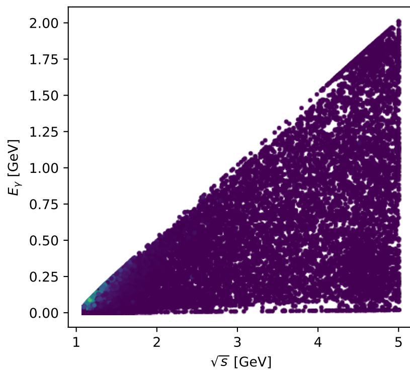
Phase-space scan: L muon + L proton [LL], max F_3=0.86751
