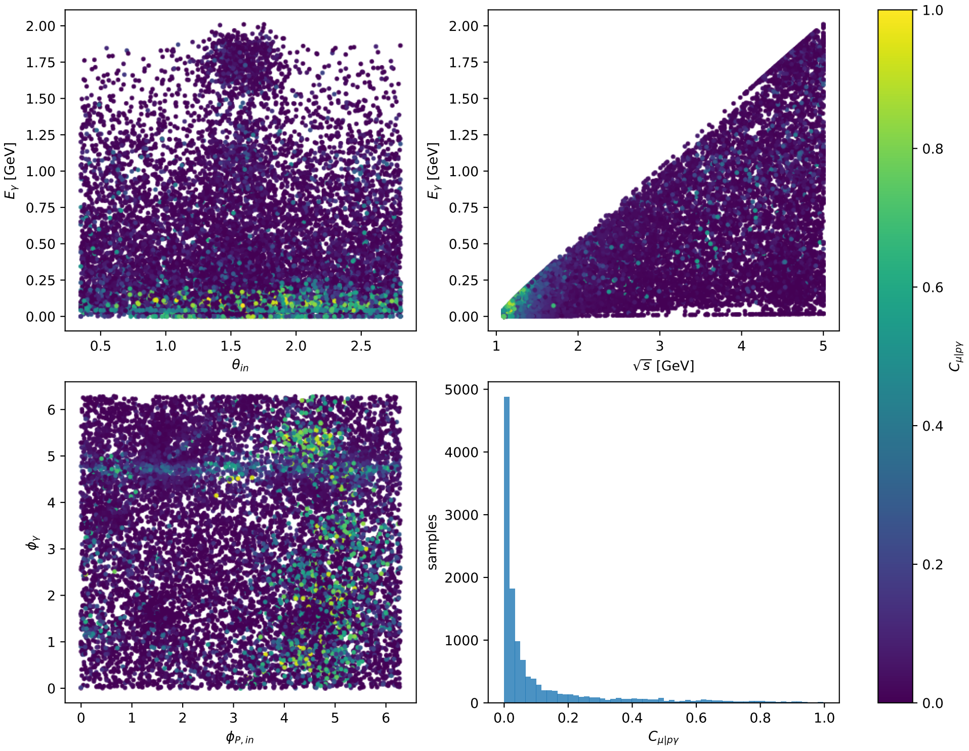
Phase-space scan: L muon + L proton [LL], max C_{\mu|p\gamma}=0.99684
