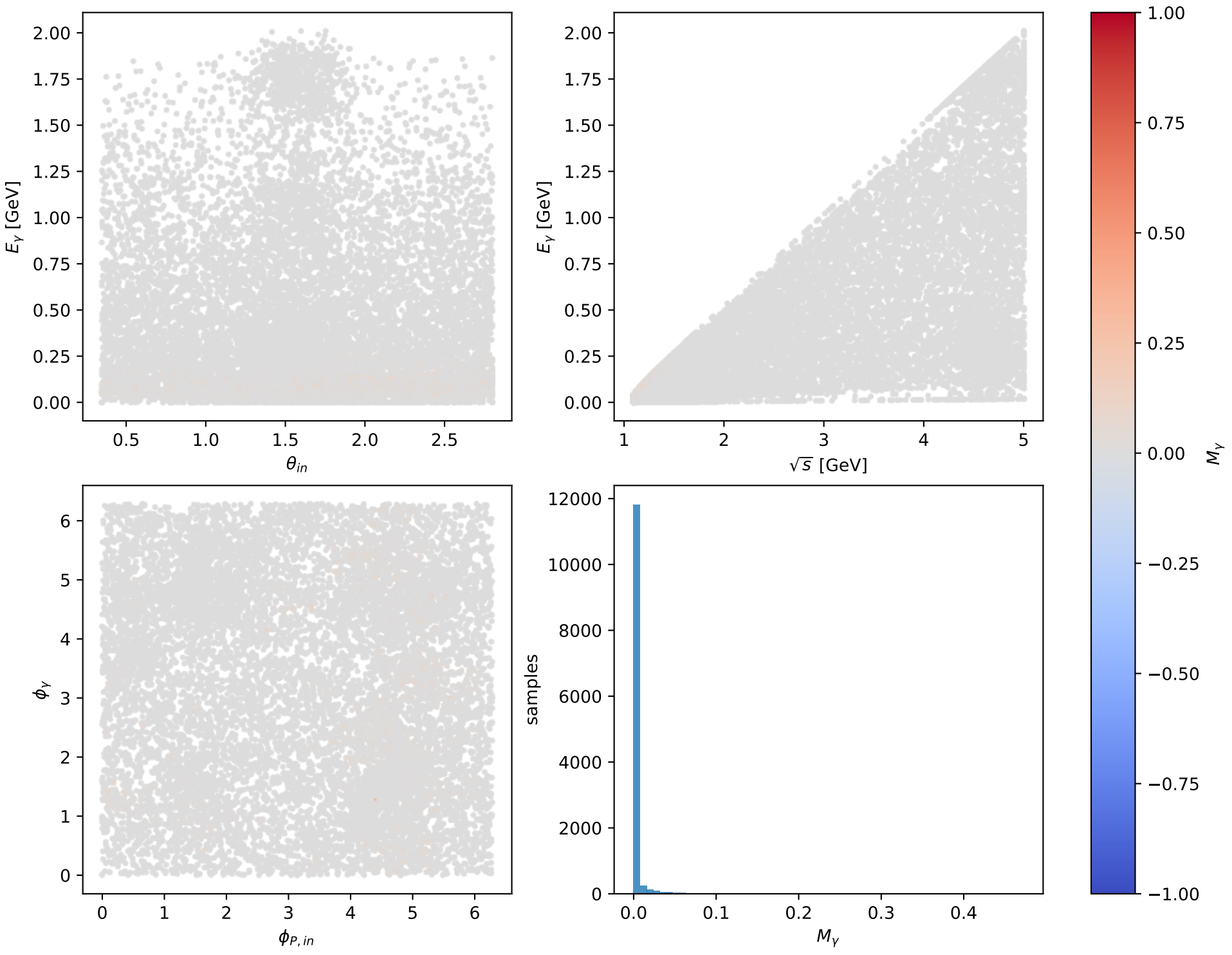
Phase-space scan: L muon + L proton [LL], max M_\gamma=0.47258
