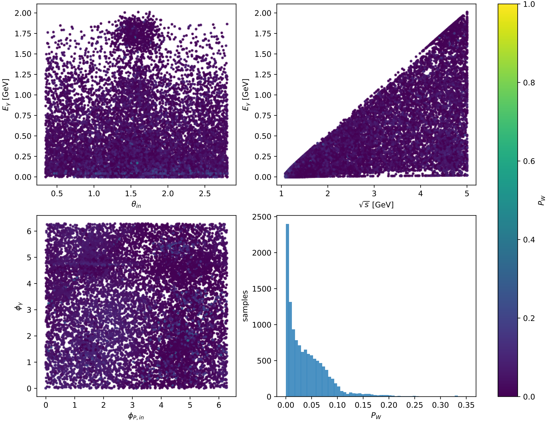
Phase-space scan: L muon [L_electron], max P_W=0.35145
