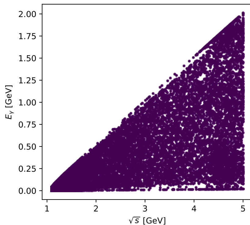
Phase-space scan: L muon [L_electron], max F_3=0
