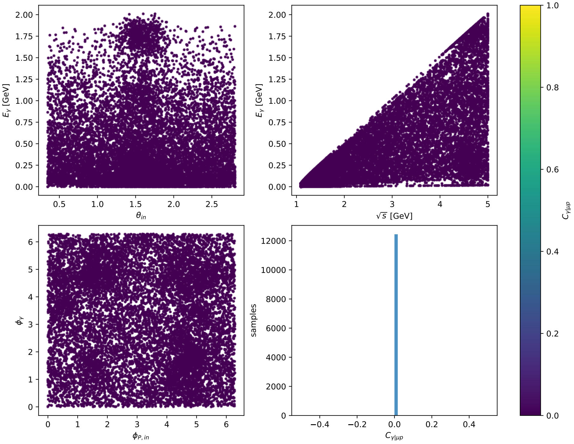
Phase-space scan: L muon [L_electron], max C_{\gamma|\mu p}=0
