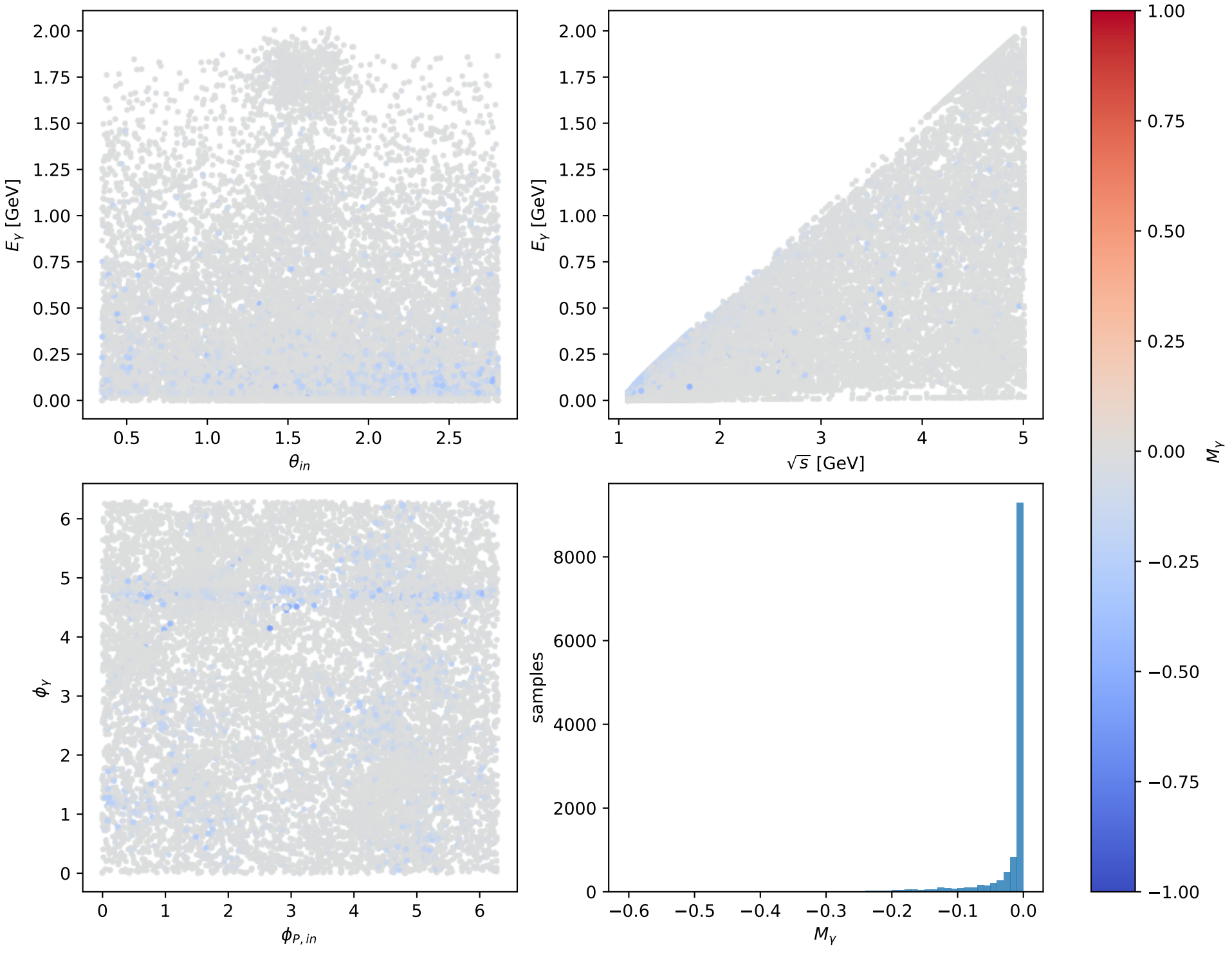
Phase-space scan: L muon [L_electron], max M_\gamma = -0
