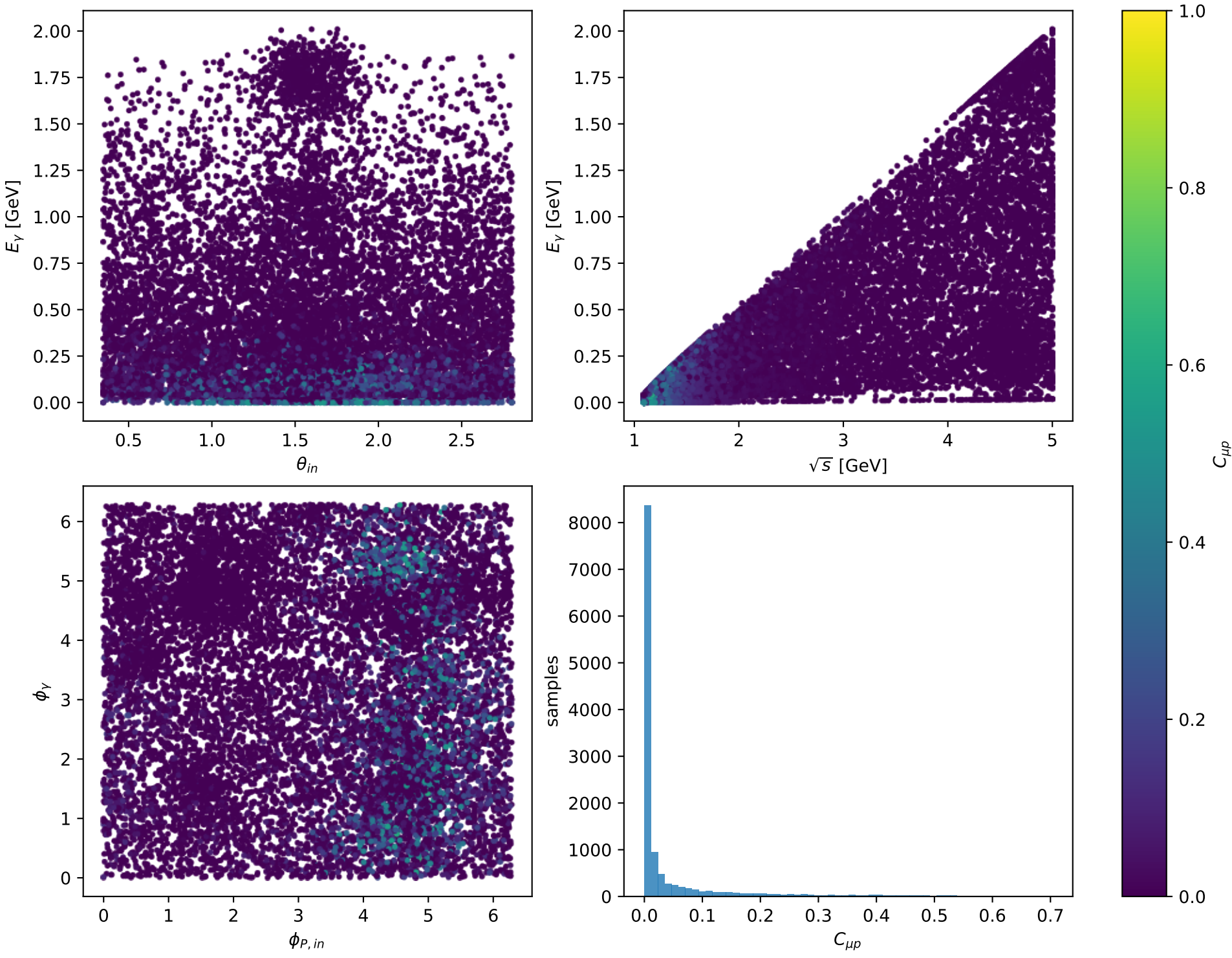
Phase-space scan: L muon [L_electron], max C_{\mu p}=0.70327
