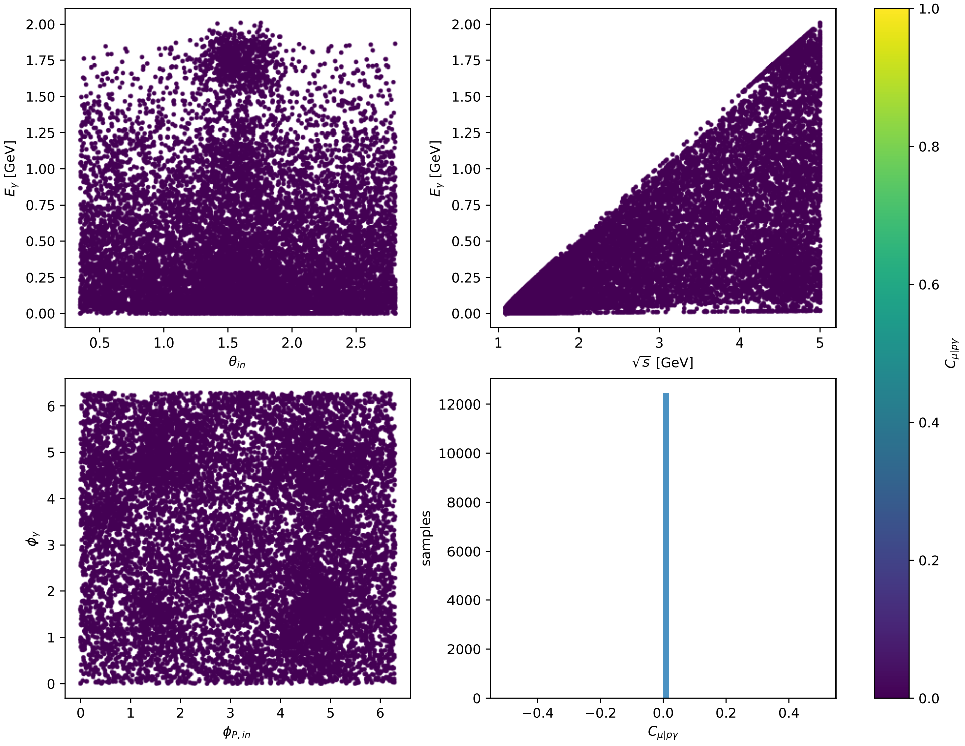
Phase-space scan: L muon [L_electron], max C_{\mu|p\gamma}=0
