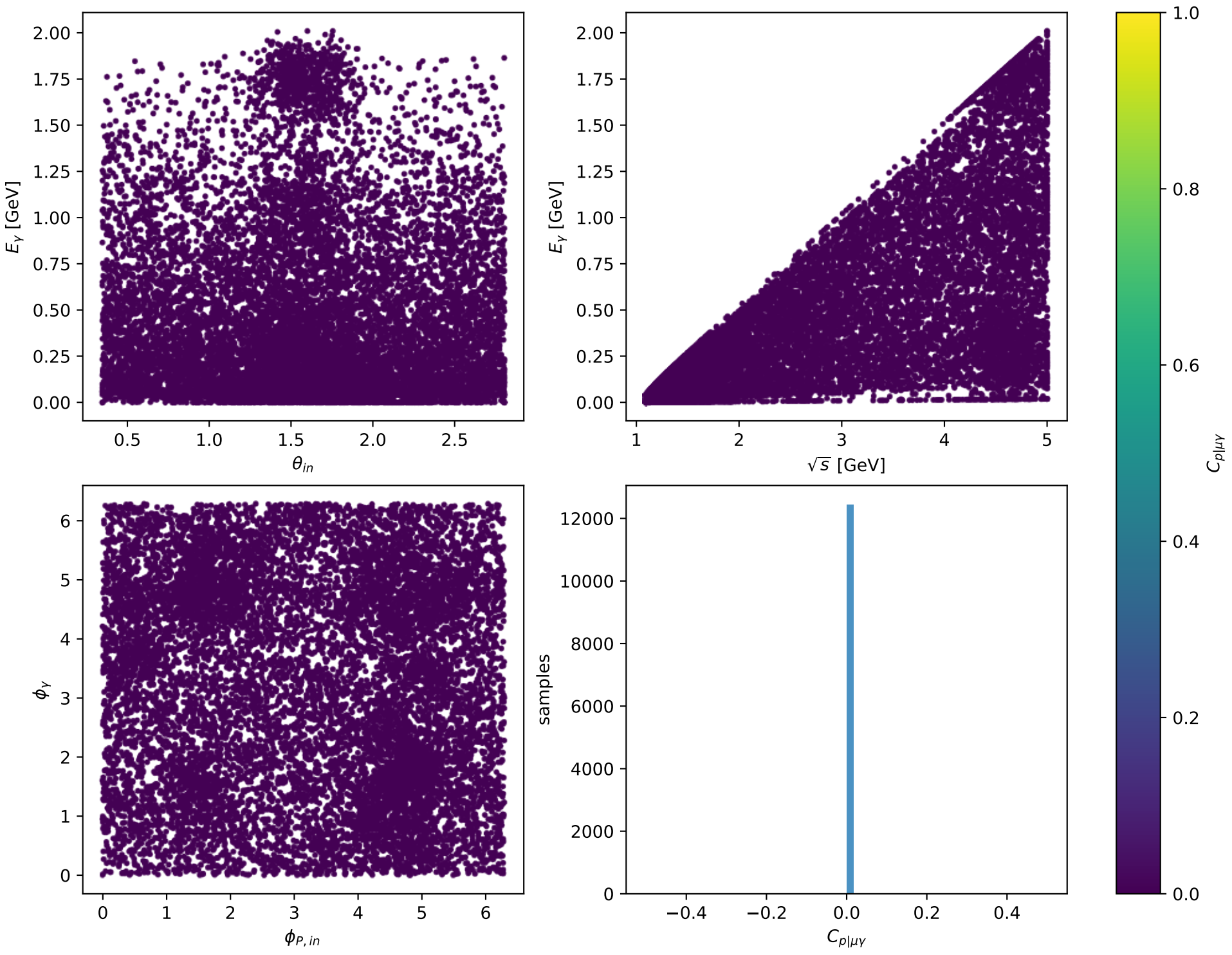
Phase-space scan: L muon [L_electron], max C_{\rho|\mu\gamma}=0
