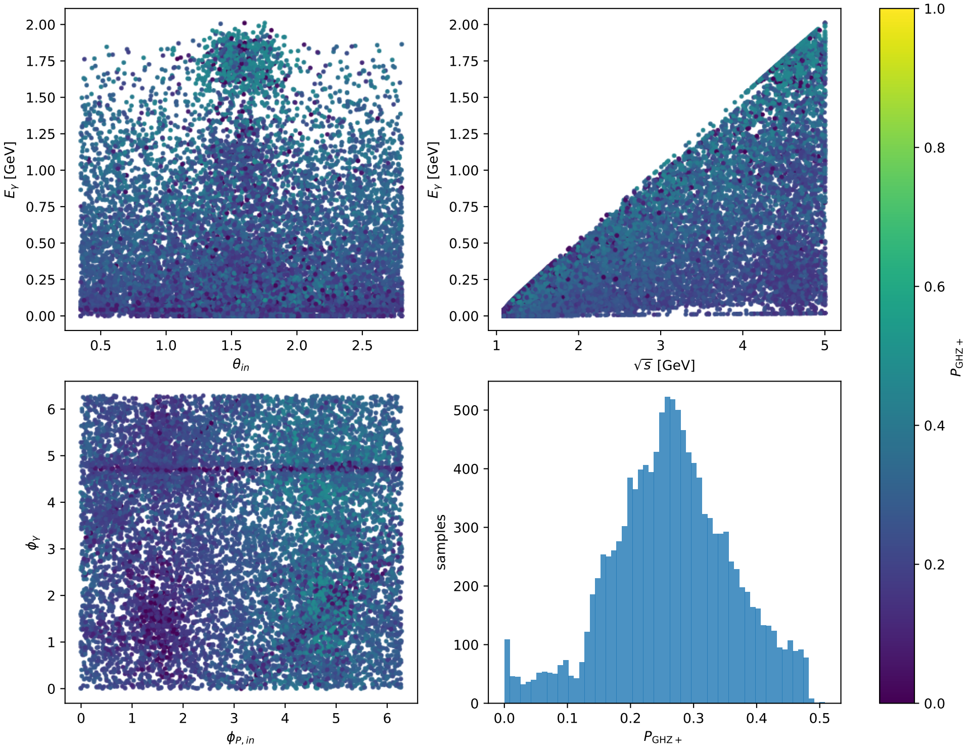
Phase-space scan: L muon [L_electron], max P_{\text{GHZ}+}=0.50816
