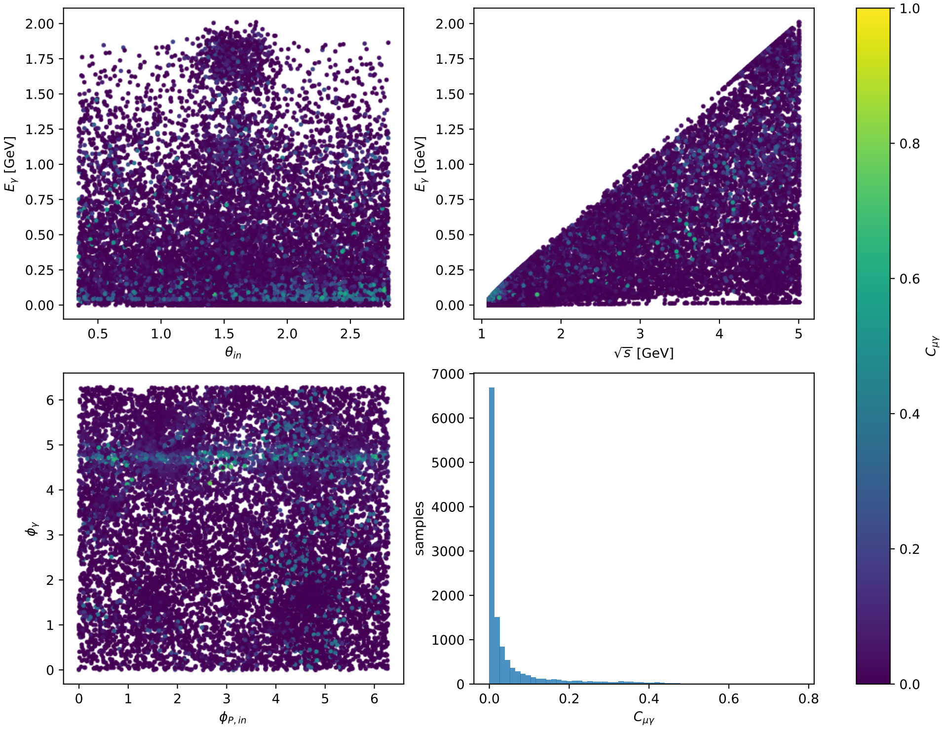
Phase-space scan: L muon [L_electron], max C_{\mu\gamma}=0.77494
