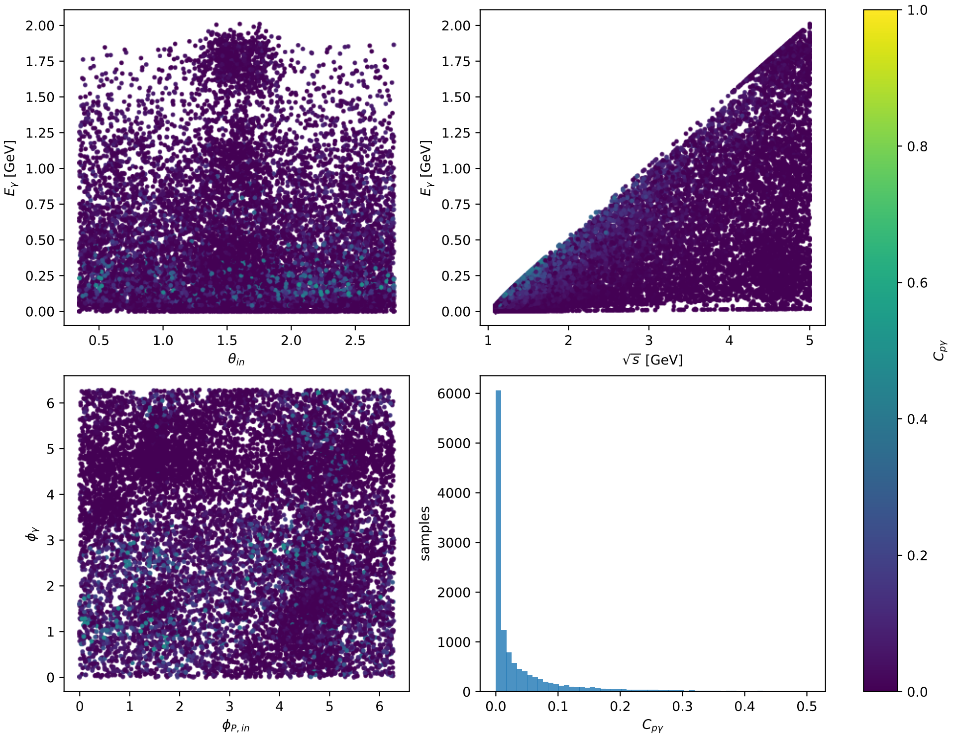
Phase-space scan: L muon [L_electron], max C_{p\gamma}=0.50462
