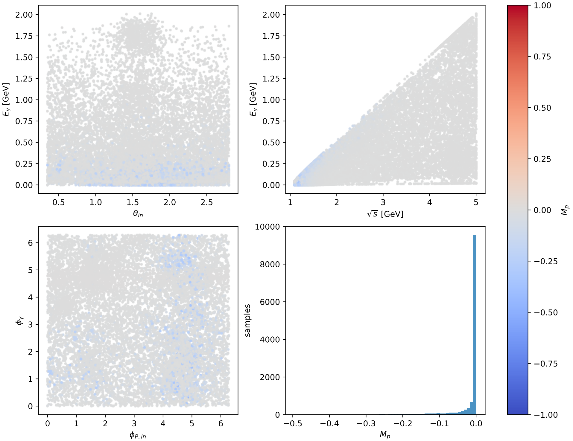
Phase-space scan: L muon [L_electron], max M_p = -0
