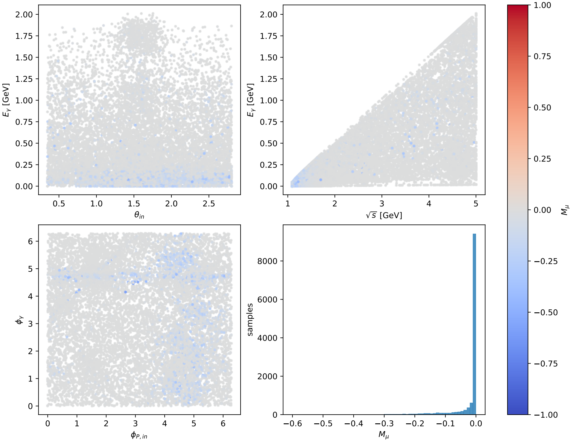
Phase-space scan: L muon [L_electron], max M_\mu = -5.2754\text{e-}19
