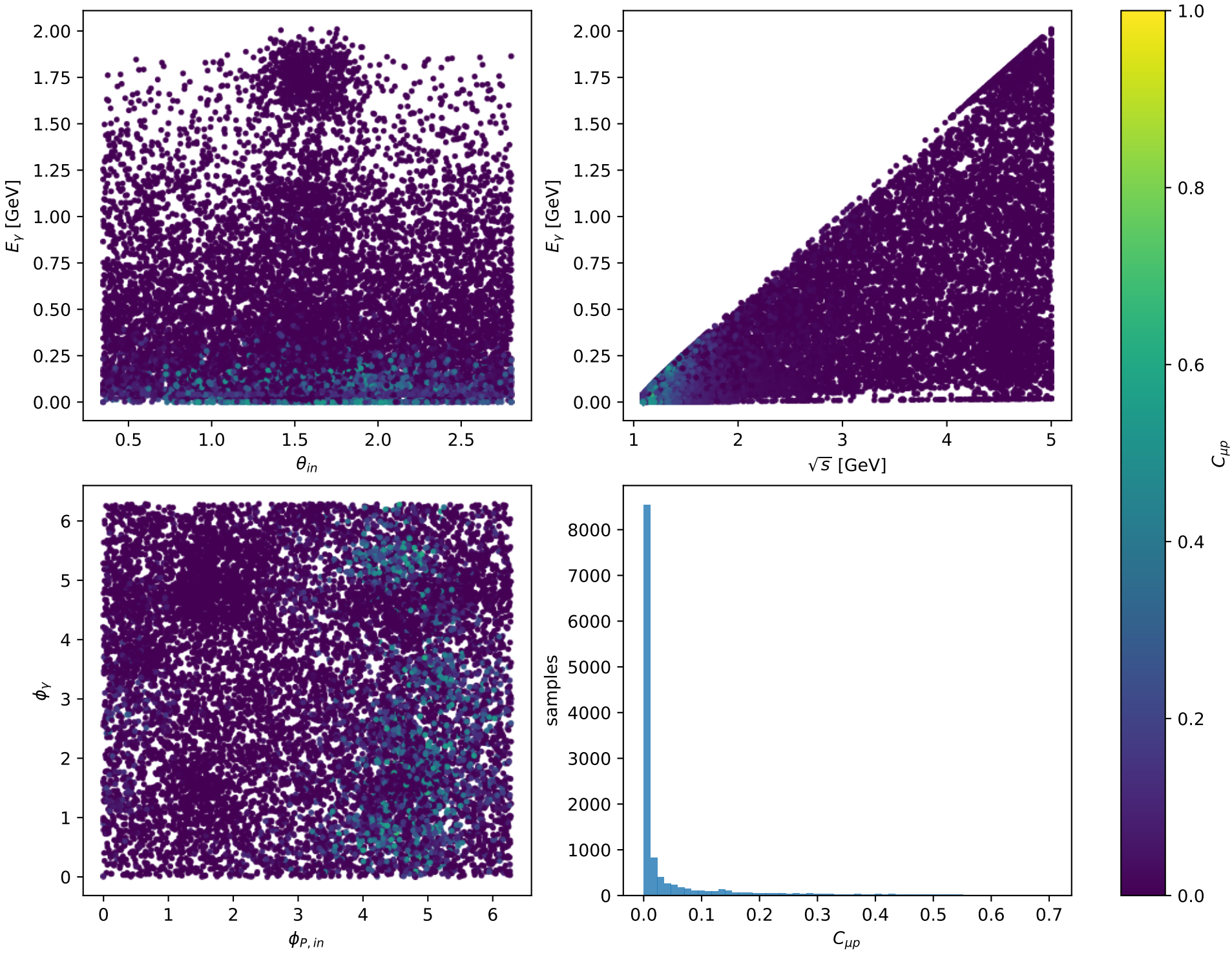
Phase-space scan: L proton [L_proton], max C_{\mu p}=0.70358
