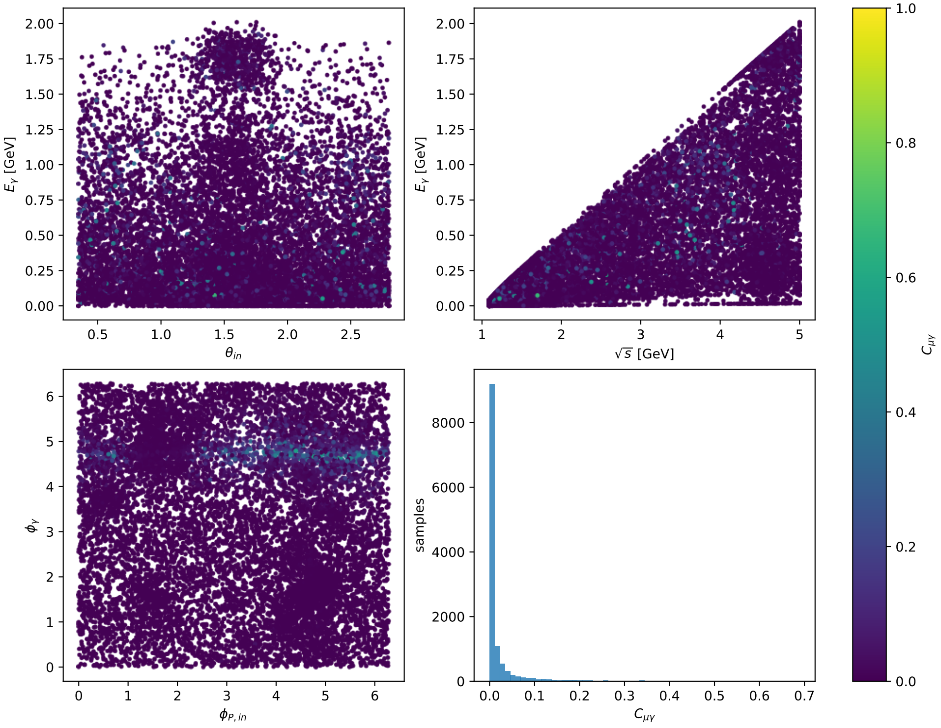
Phase-space scan: L proton [L_proton], max C_{\mu\gamma}=0.68922
