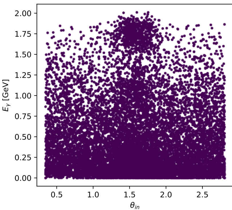
Phase-space scan: L proton [L_proton], max C_{\mu|p\gamma}=0
