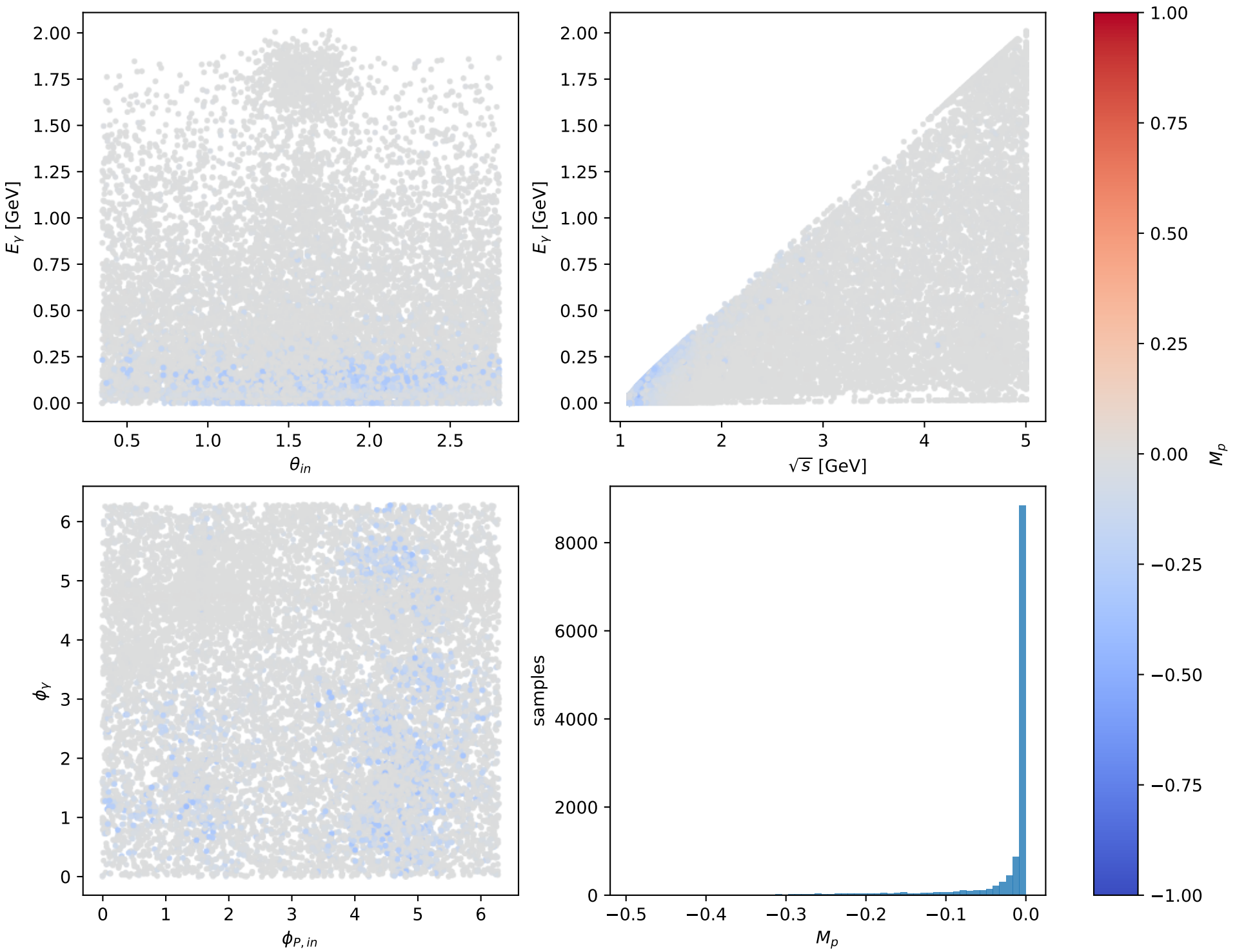
Phase-space scan: L proton [L_proton], max M_p=-0
