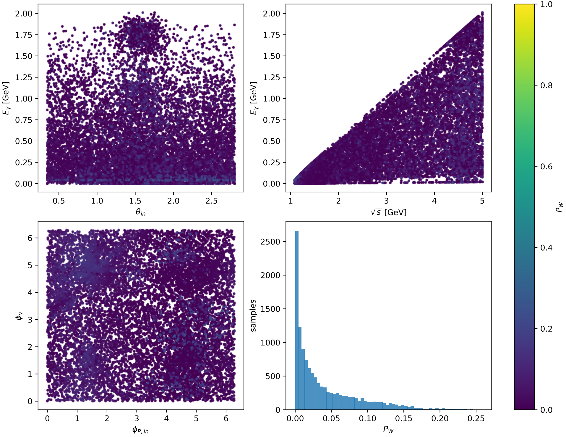
Phase-space scan: L proton [L_proton], max P_W=0.25857
