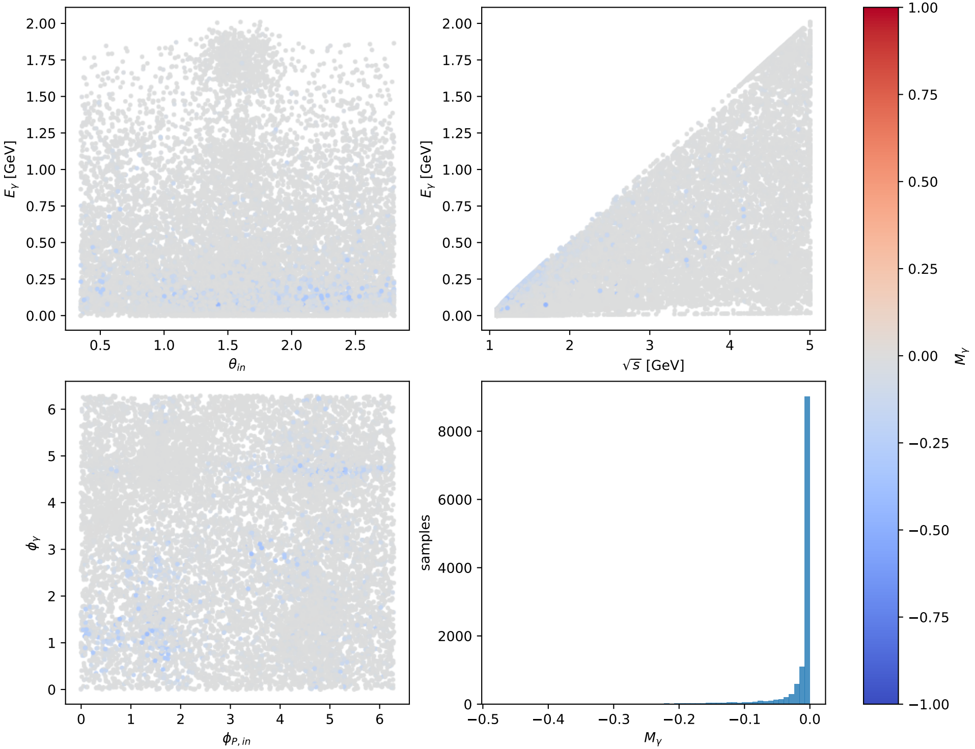
Phase-space scan: L proton [L_proton], max M_Y=-0
