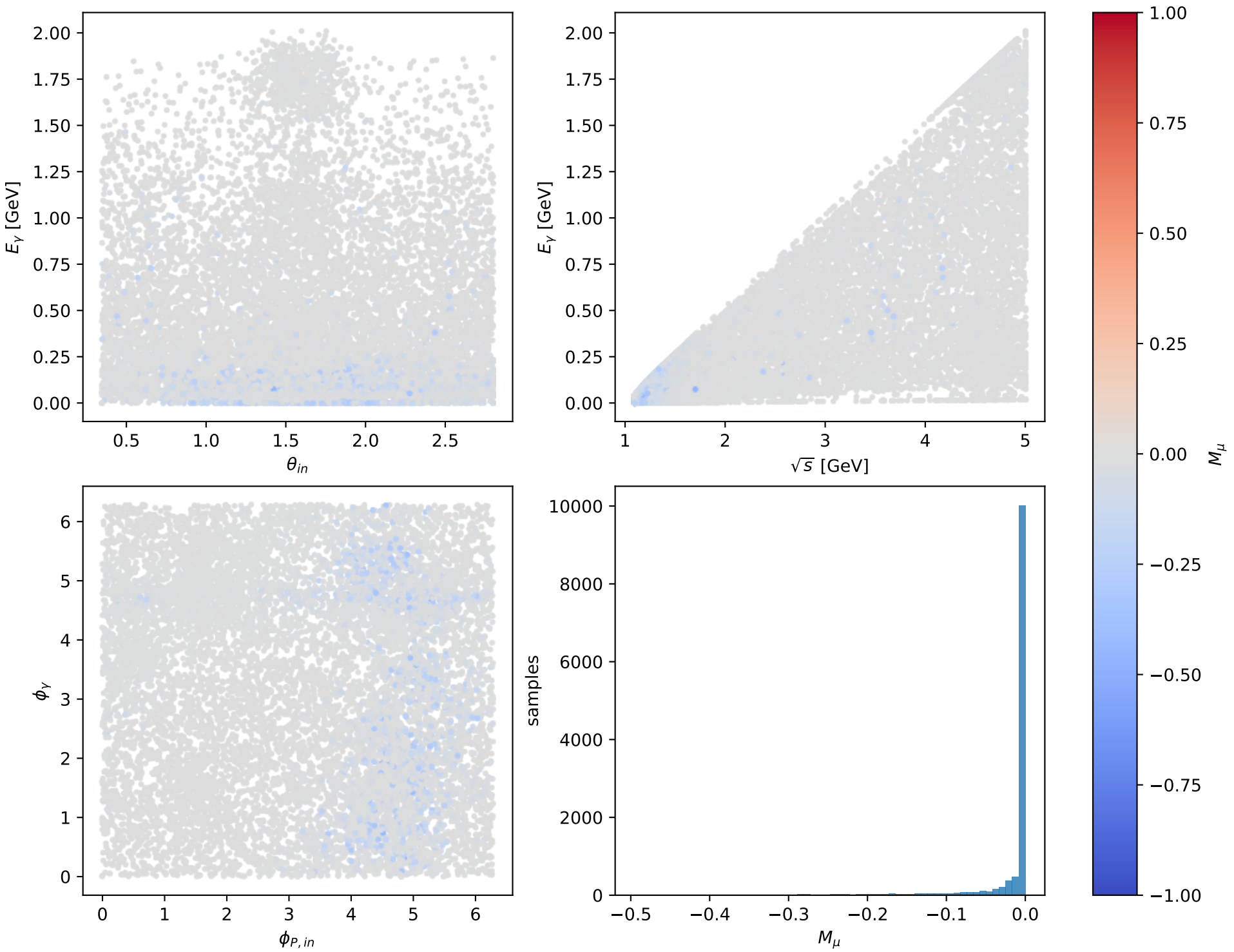
Phase-space scan: L proton [L_proton], max M_\mu = -0
