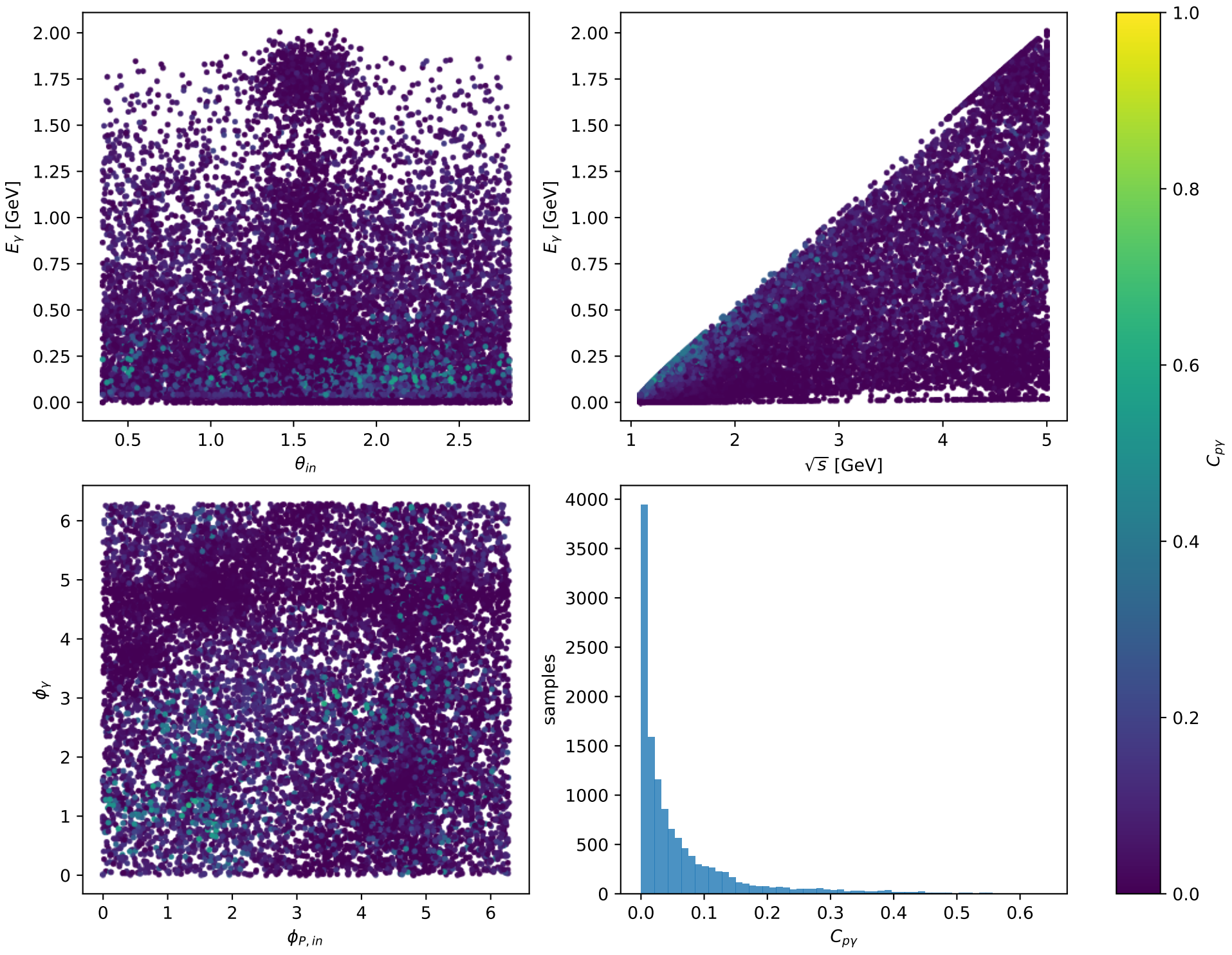
Phase-space scan: L proton [L_proton], max C_{py}=0.6424
