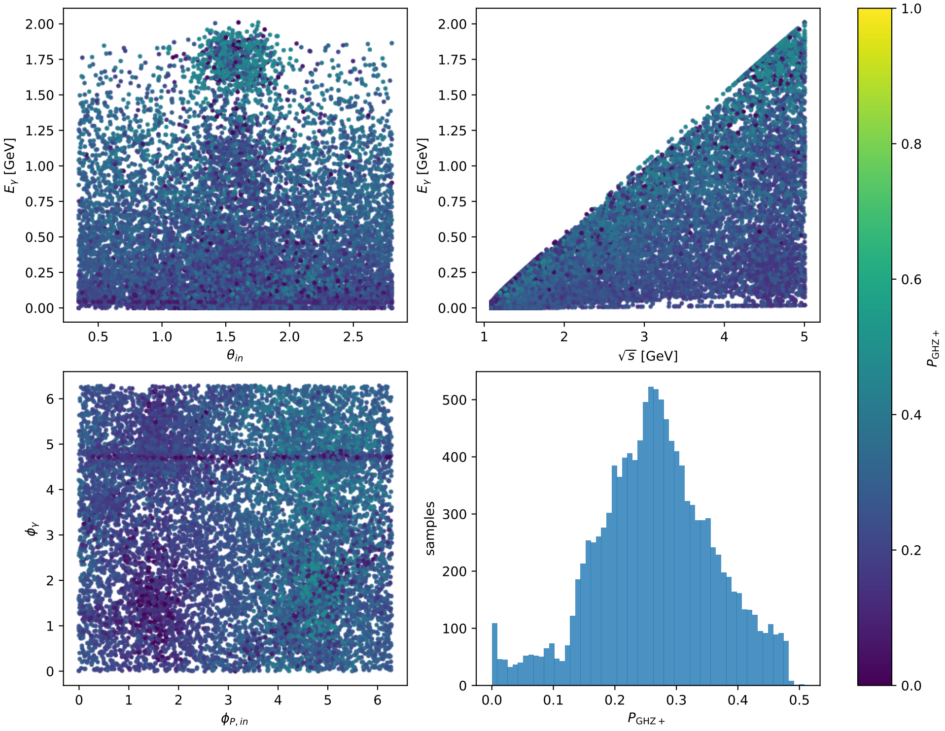
Phase-space scan: L proton [ L_{\text{proton}} ], max P_{\text{GHZ}+}=0.50816
