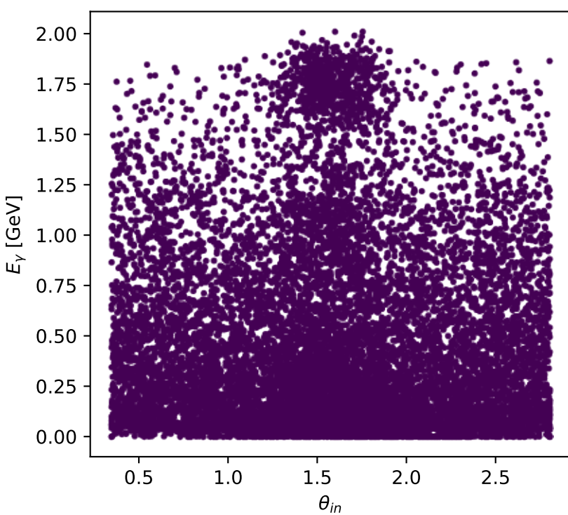
Phase-space scan: L proton [L_proton], max C_{p|\mu\gamma}=0
