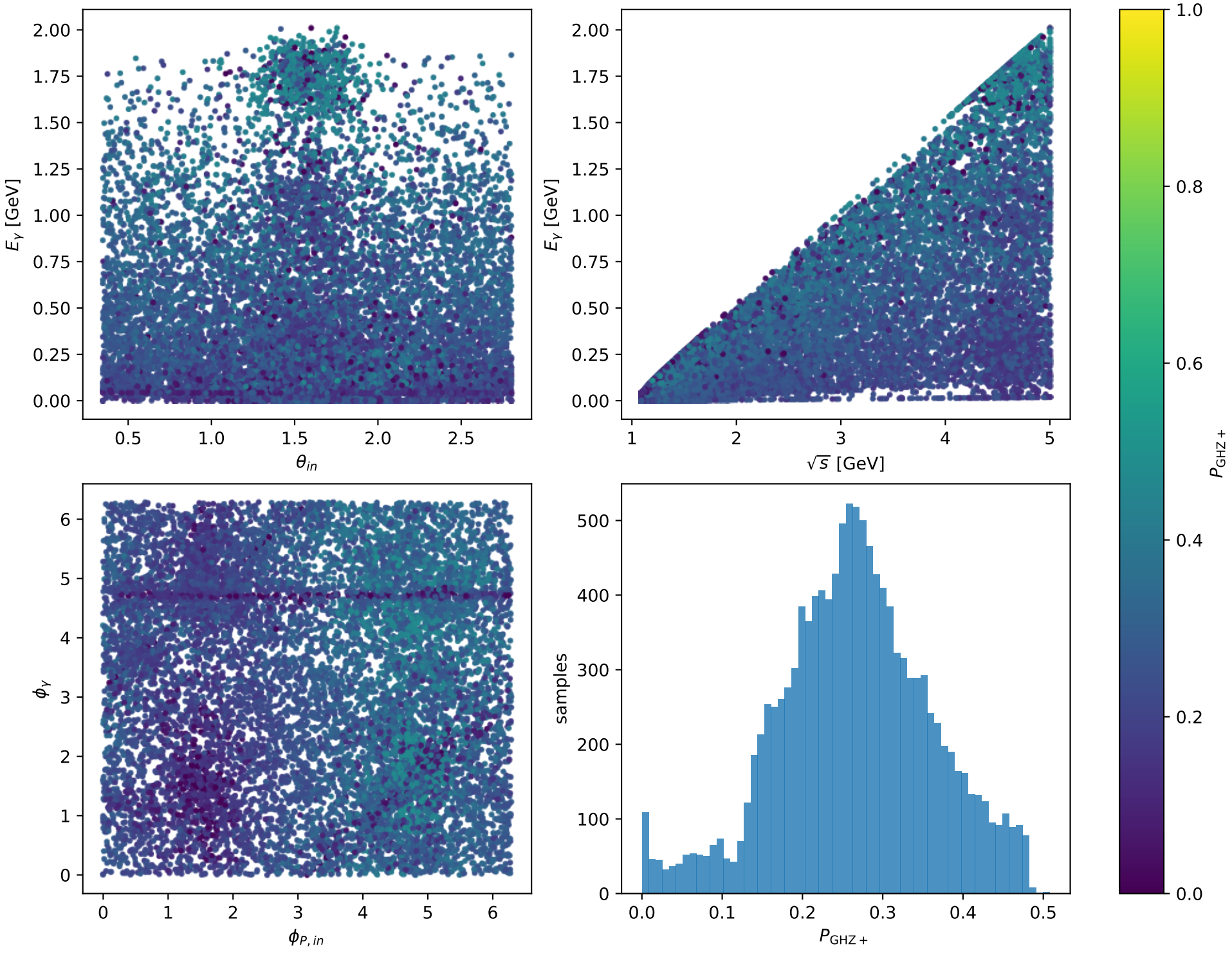
Phase-space scan: Tx muon [Tx_electron], max P_{\text{GHZ}+}=0.50816
