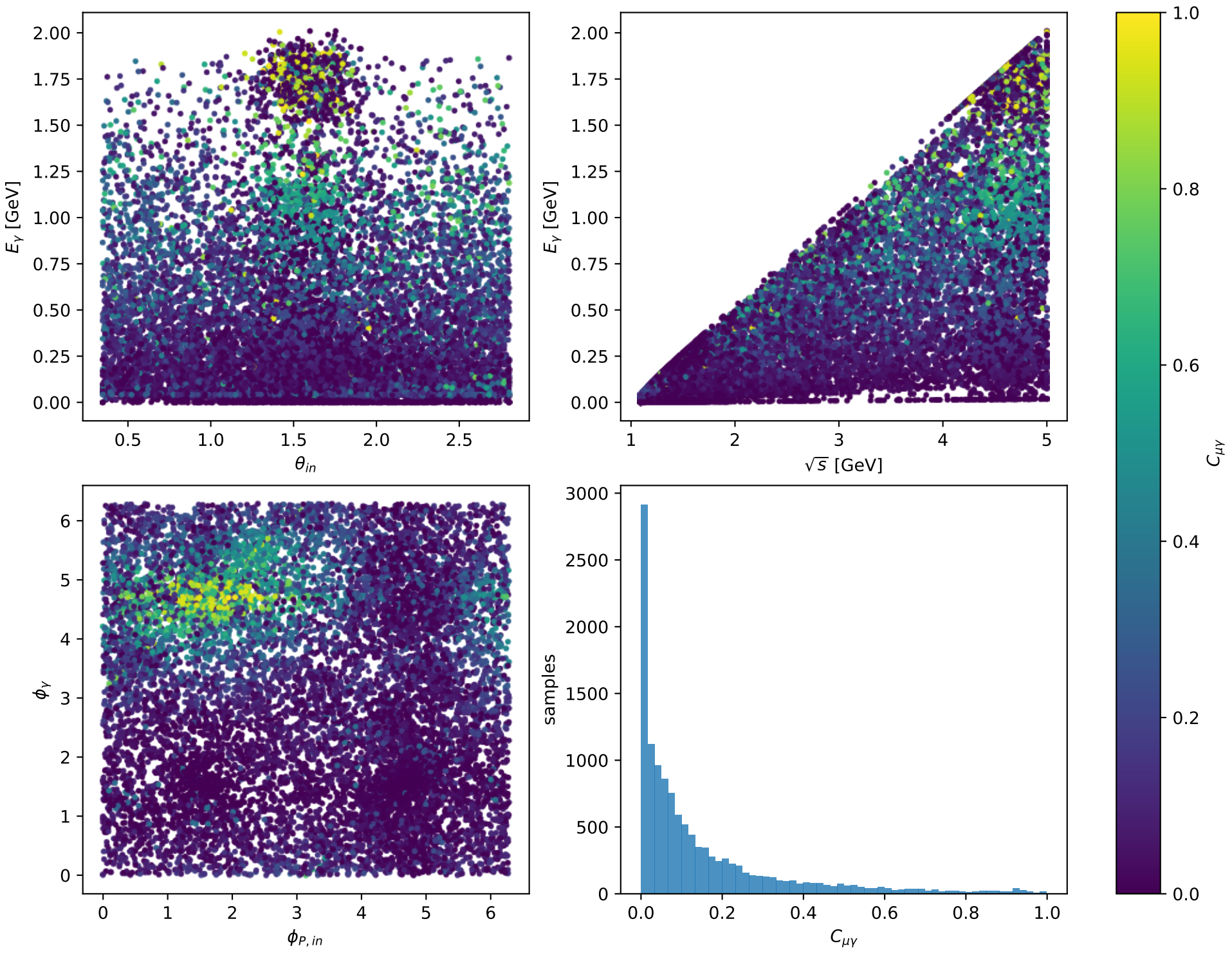
Phase-space scan: Tx muon [Tx_electron], max C_{\mu\gamma}=0.99935
