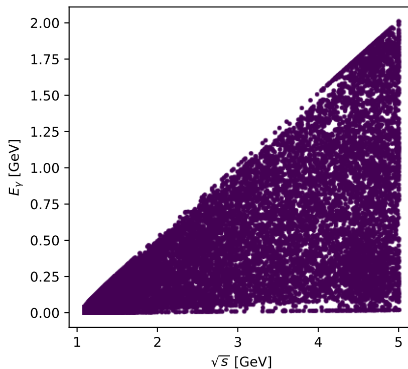
Phase-space scan: Tx muon [Tx_electron], max F_3=0
