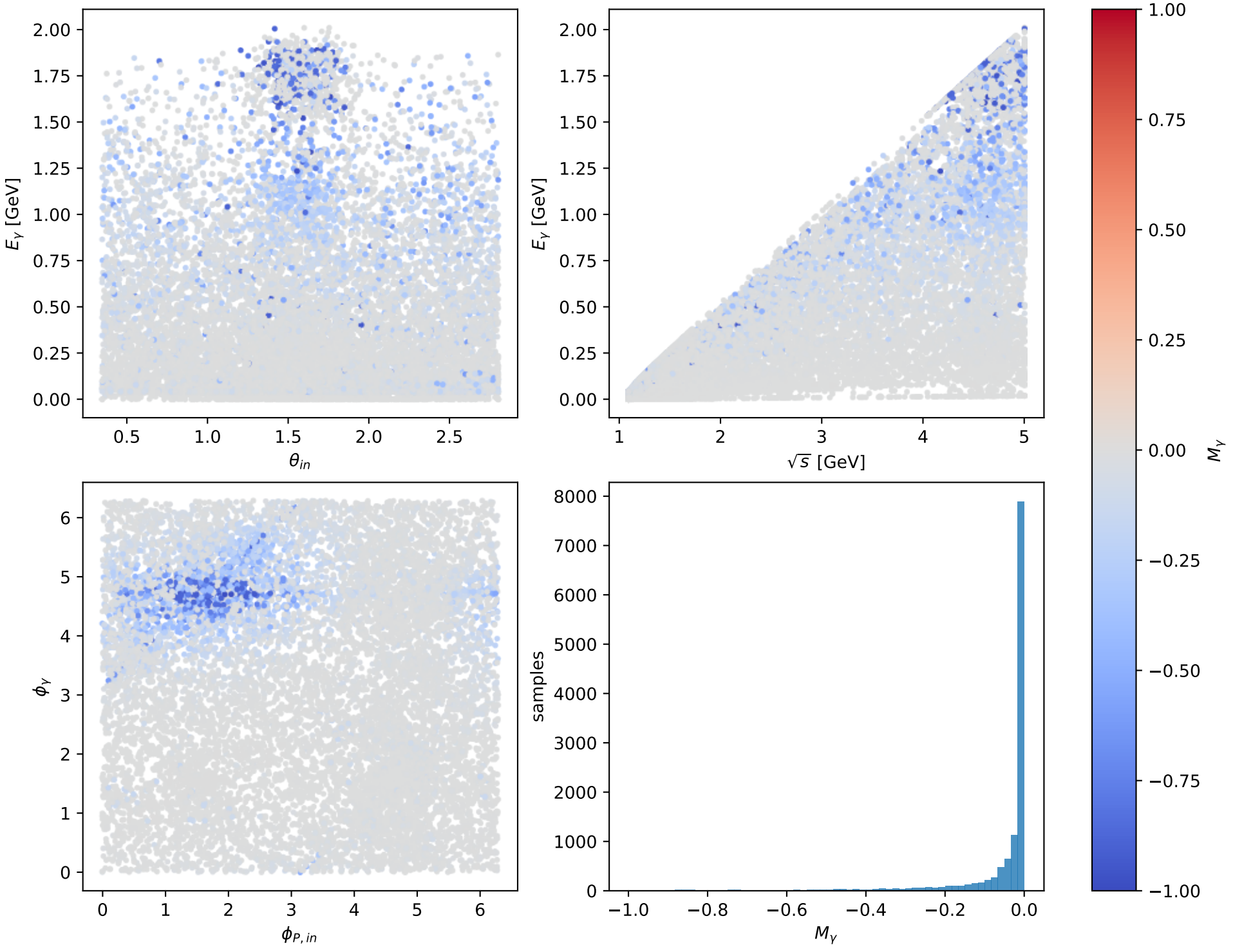
Phase-space scan: Tx muon [Tx_electron], max M_\gamma = -0
