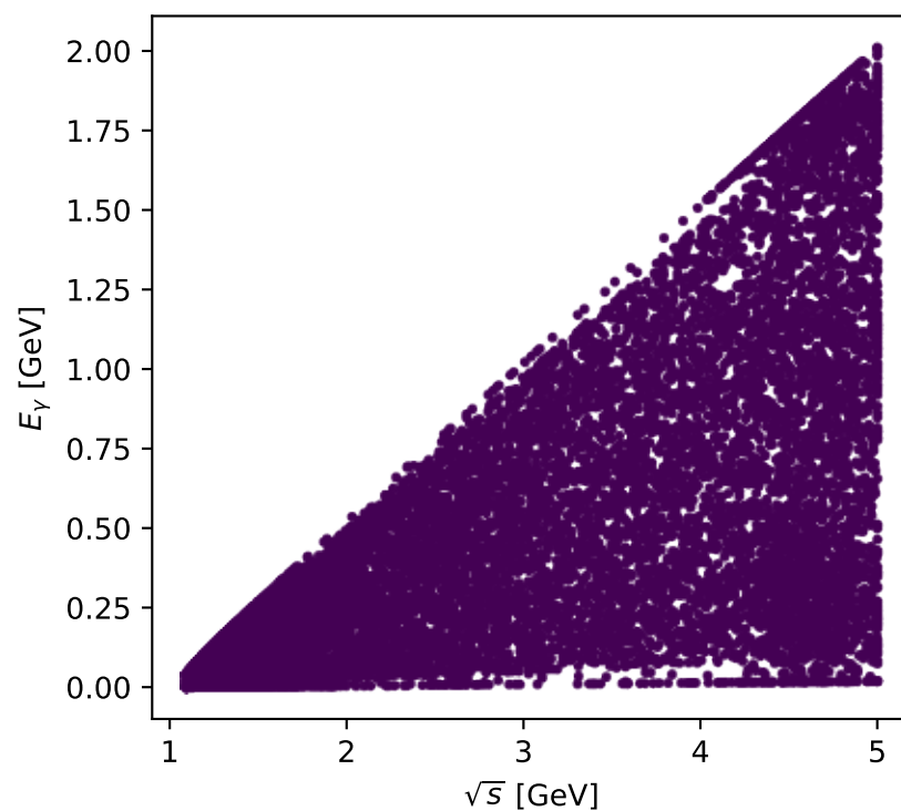
Phase-space scan: Tx muon [Tx_electron], max C_{\rho|\mu\gamma}=0
