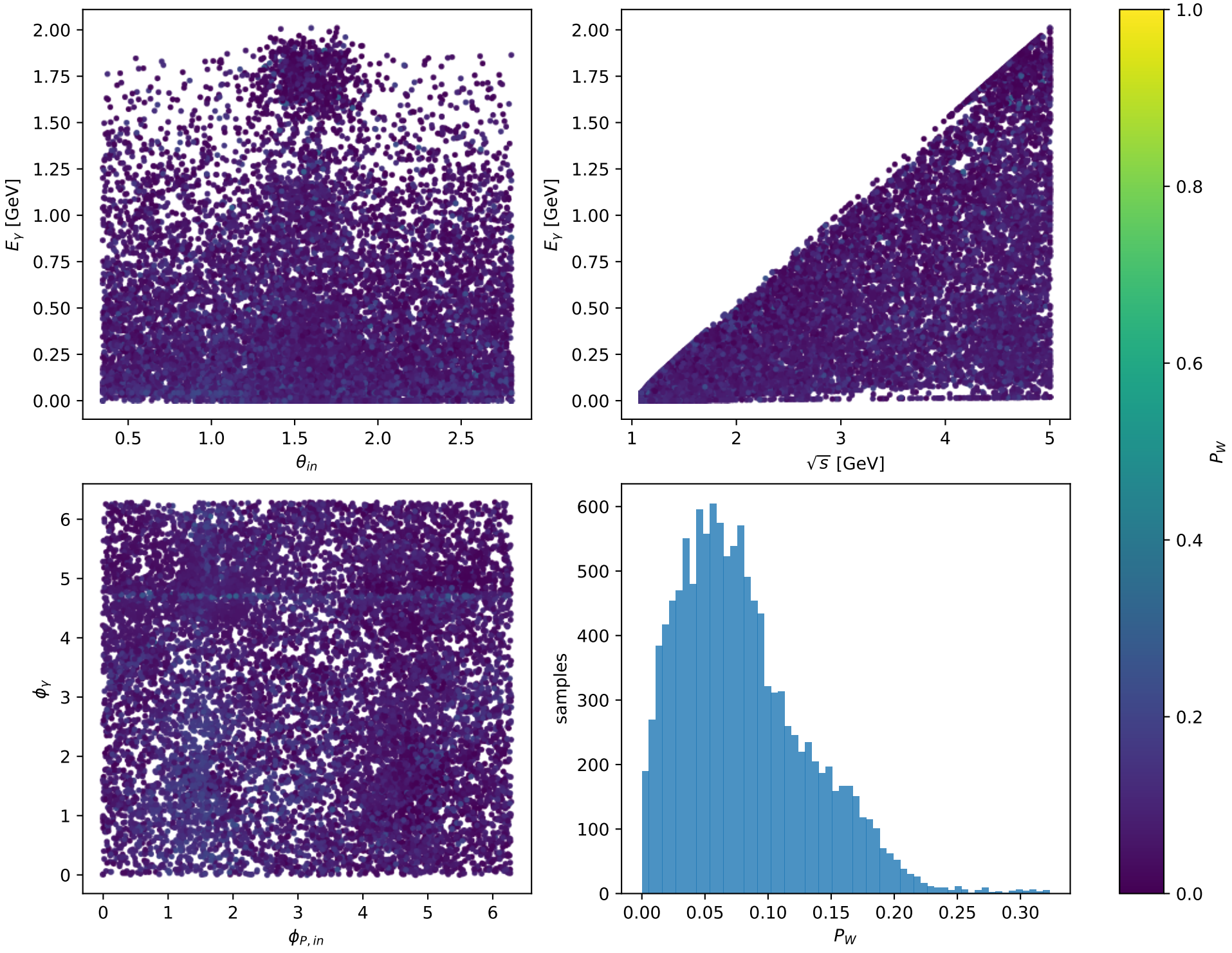
Phase-space scan: Tx muon [Tx_electron], max P_W=0.3233
