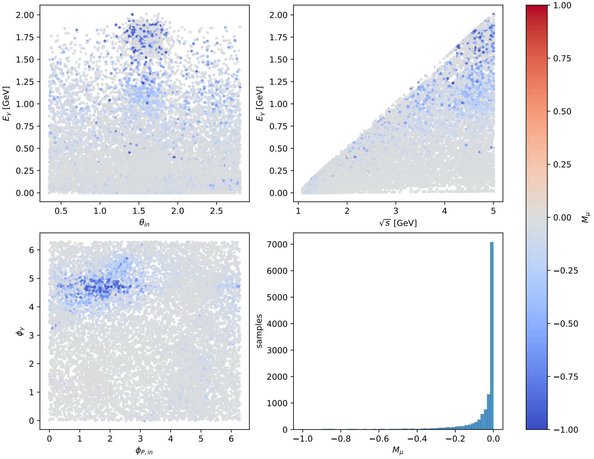
Phase-space scan: Tx muon [Tx_electron], max M_\mu=-0
