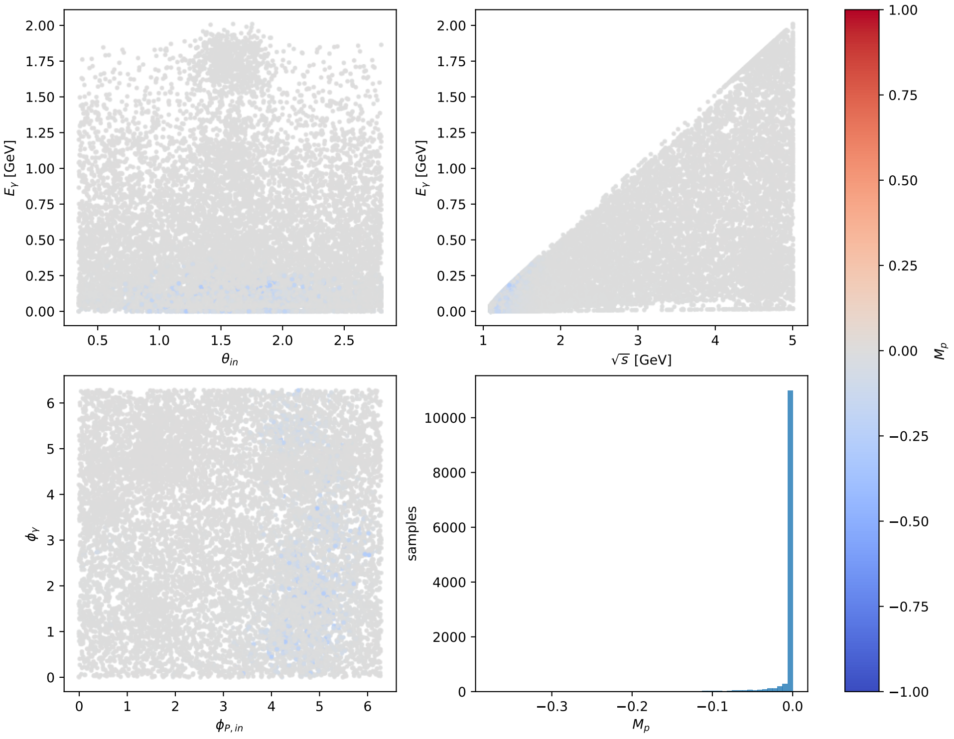
Phase-space scan: Tx muon [Tx_electron], max M_p = -0
