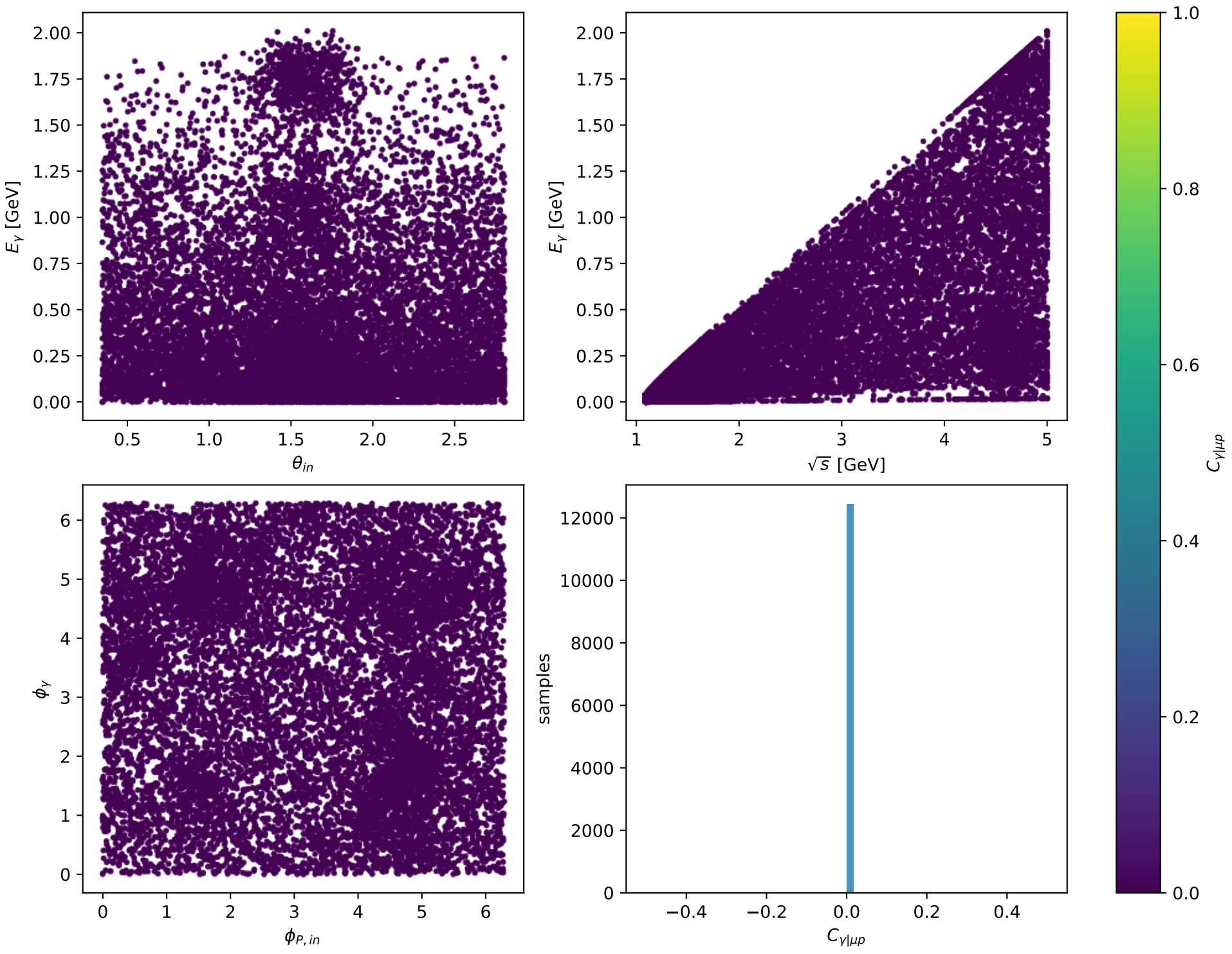
Phase-space scan: Tx muon [Tx_electron], max C_{\gamma|\mu p}=0
