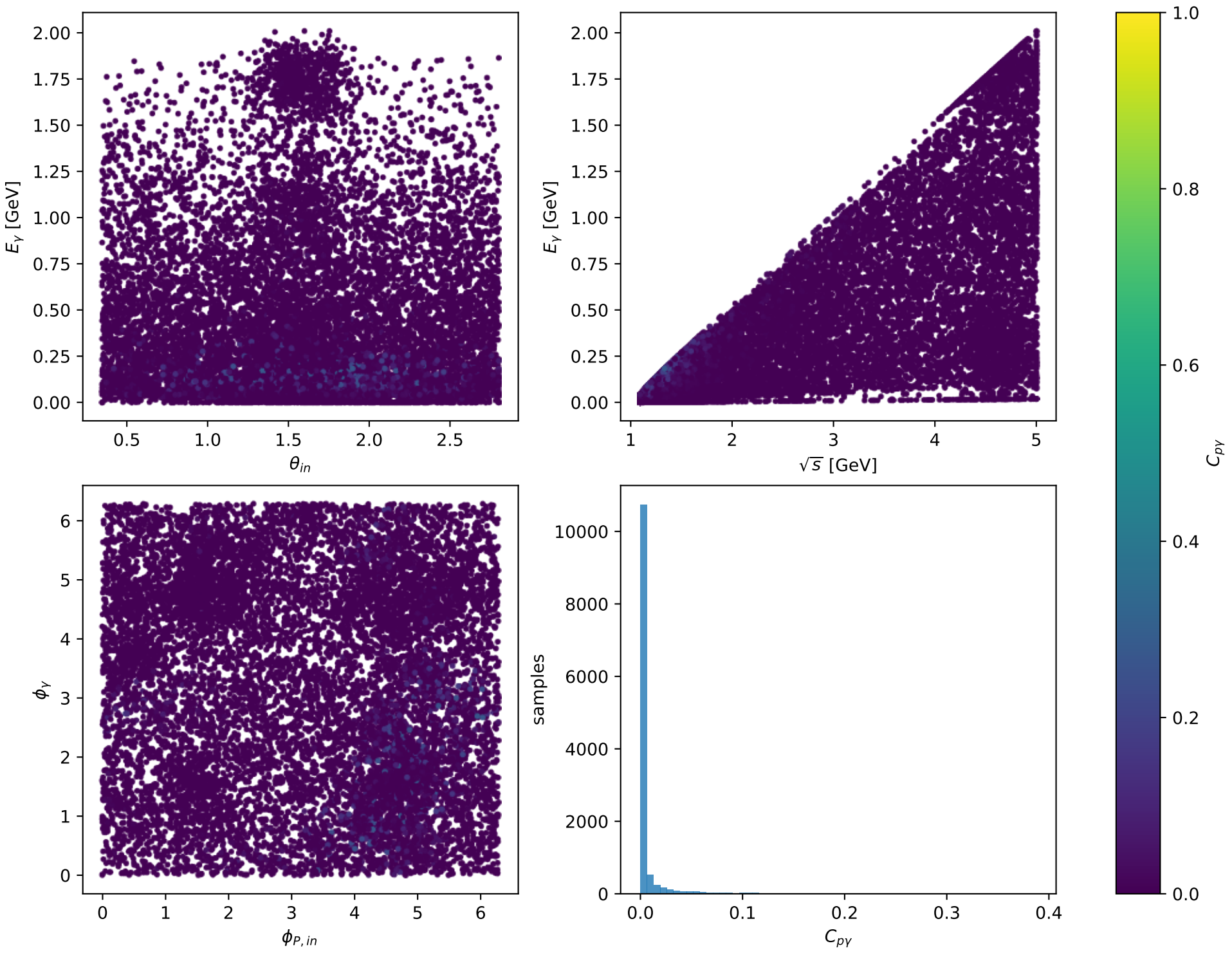
Phase-space scan: Tx muon [Tx_electron], max C_{py}=0.38768
