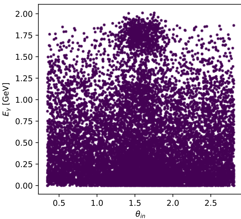
Phase-space scan: Tx muon [Tx_electron], max C_{\rho|\mu\gamma}=0
