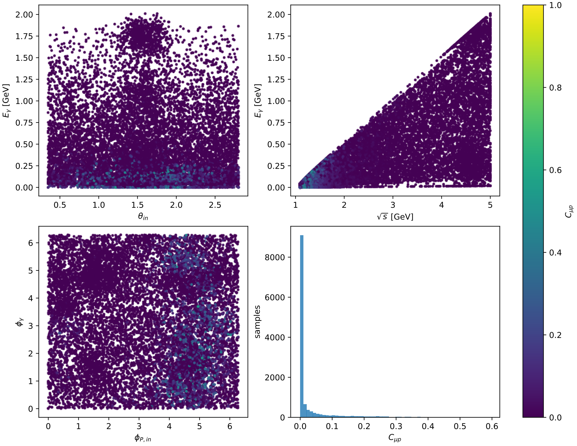
Phase-space scan: Tx muon [Tx_electron], max C_{\mu p}=0.59471
