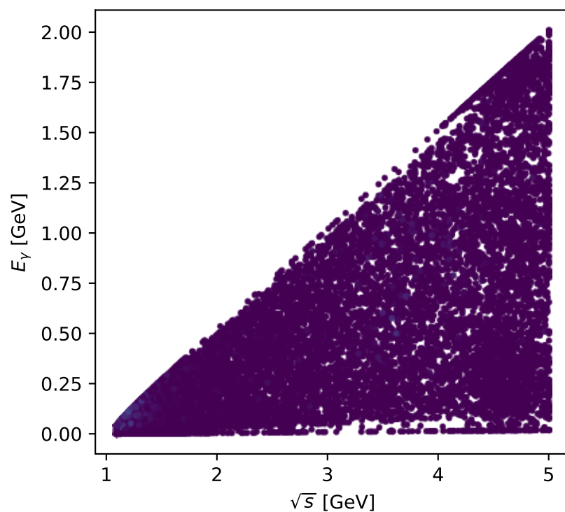
Phase-space scan: Tx proton [Tx_proton], max C_{\mu\gamma}=0.29192
