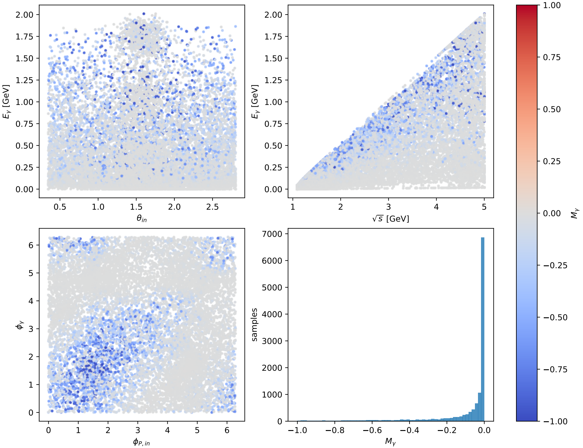
Phase-space scan: Tx proton [Tx_proton], max M_\gamma = -0
