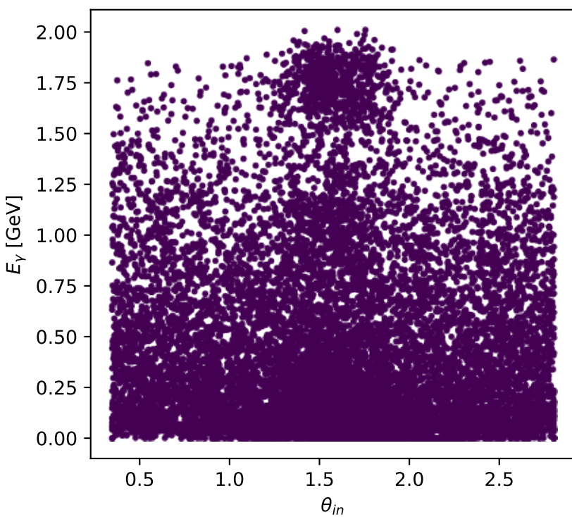
Phase-space scan: Tx proton [Tx_proton], max F_3=0
