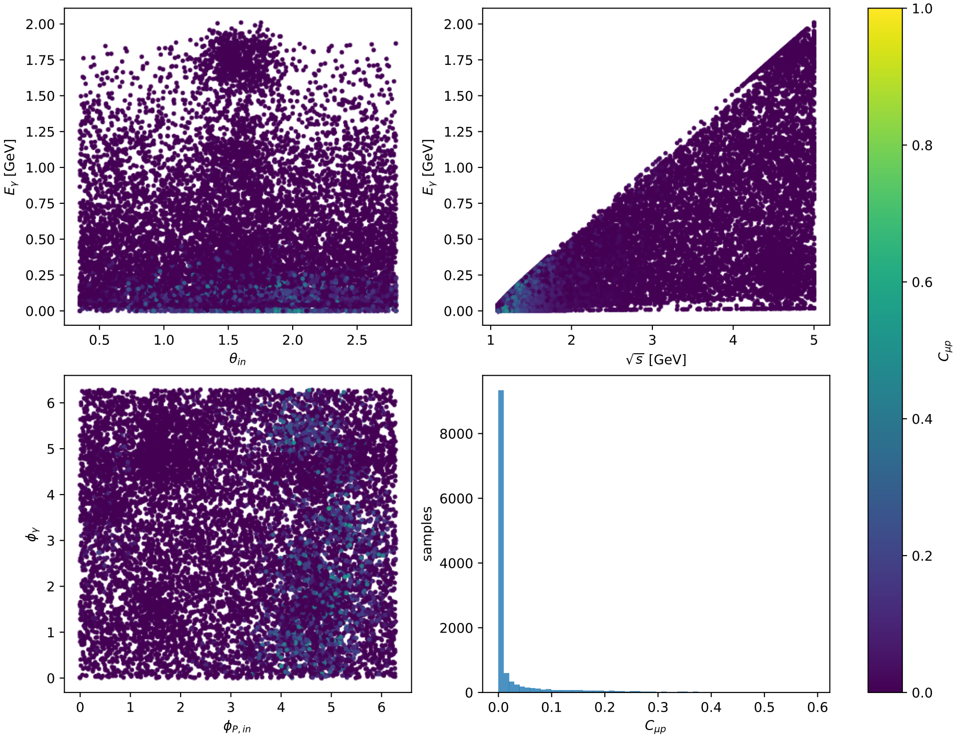
Phase-space scan: Tx proton [Tx_proton], max C_{\mu p}=0.59326
