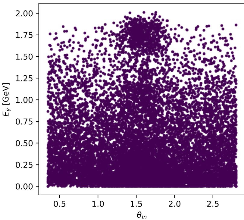
Phase-space scan: Tx proton [Tx_proton], max C_{\mu|p\gamma}=0
