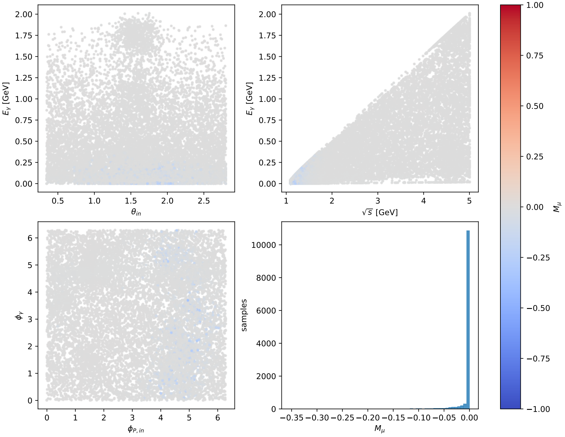
Phase-space scan: Tx proton [Tx_proton], max M_\mu = -0
