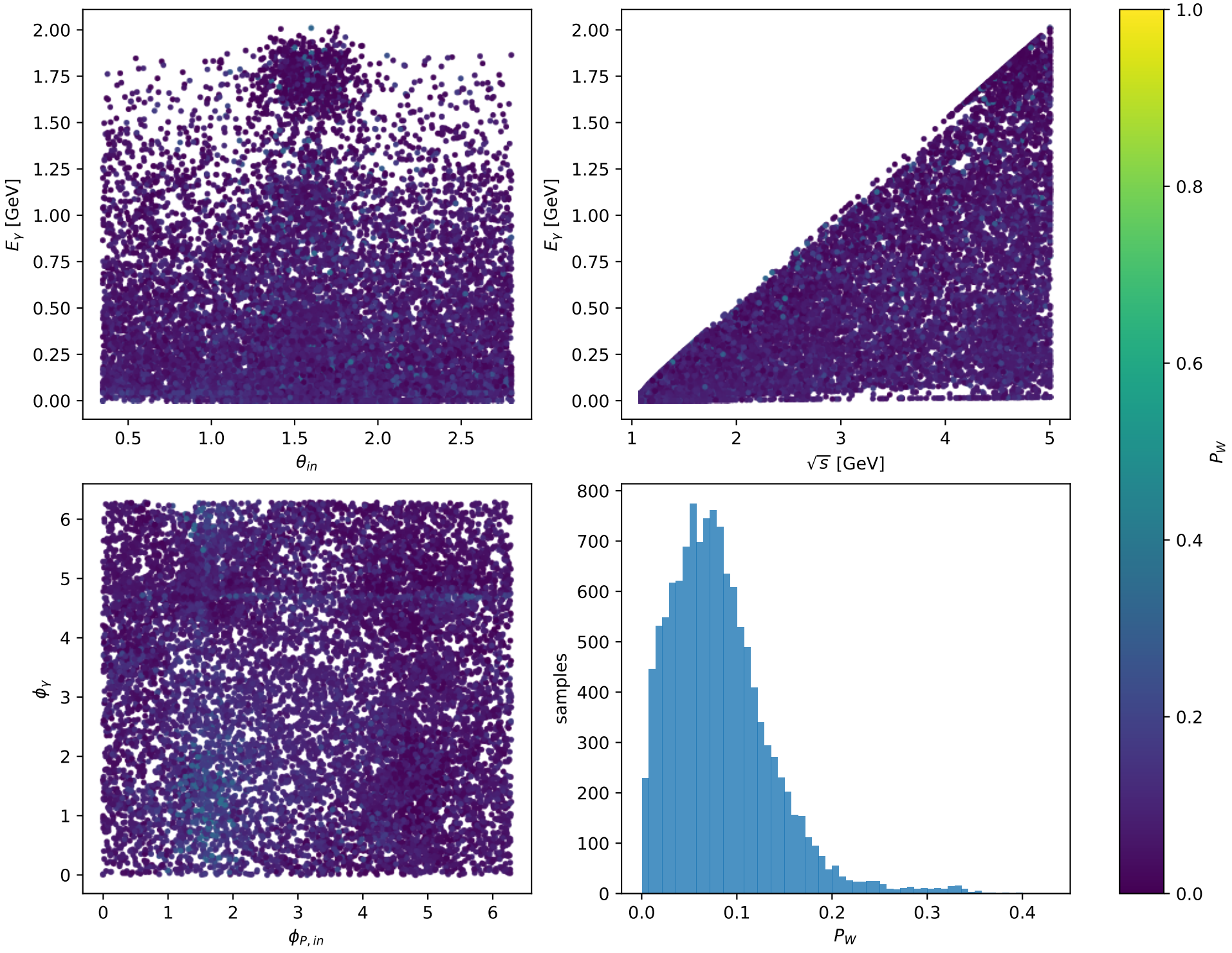
Phase-space scan: Tx proton [Tx_proton], max P_W=0.42881
