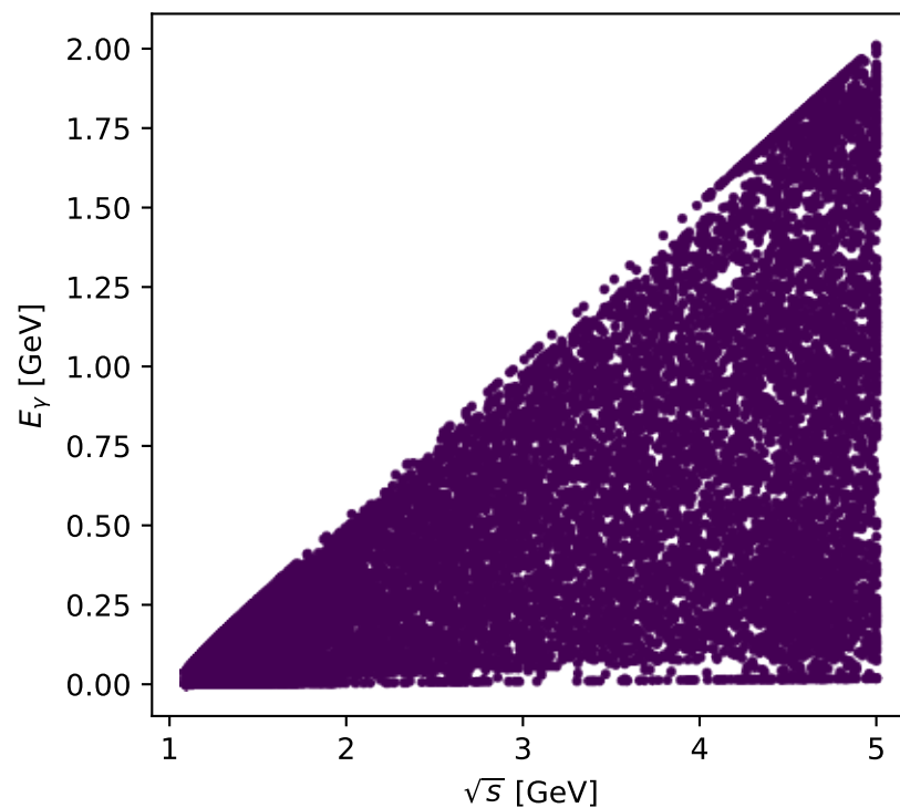
Phase-space scan: Tx proton [Tx_proton], max C_{p|\mu\gamma}=0
