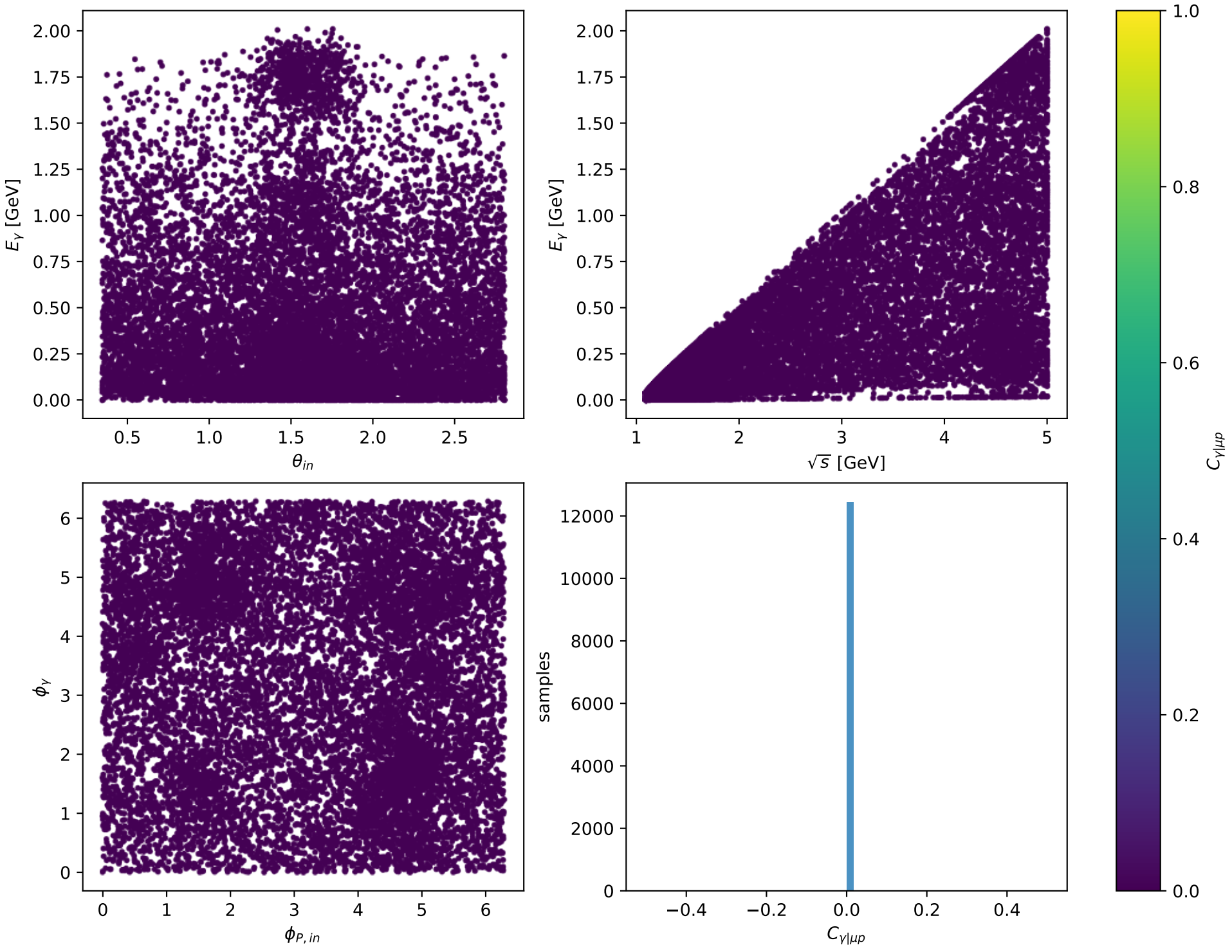
Phase-space scan: Ty muon [Ty_electron], max C_{\gamma|\mu p}=0
