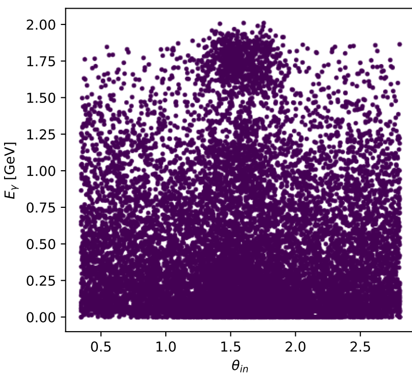
Phase-space scan: Ty muon [Ty_electron], max C_{\mu|p\gamma}=0
