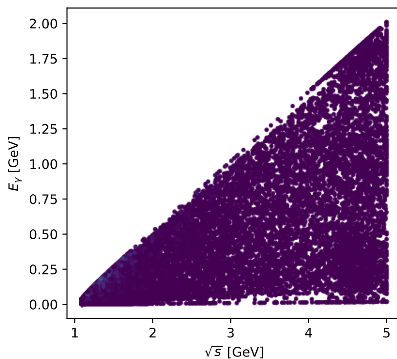
Phase-space scan: Ty muon [Ty_electron], max C_{py}=0.30967
