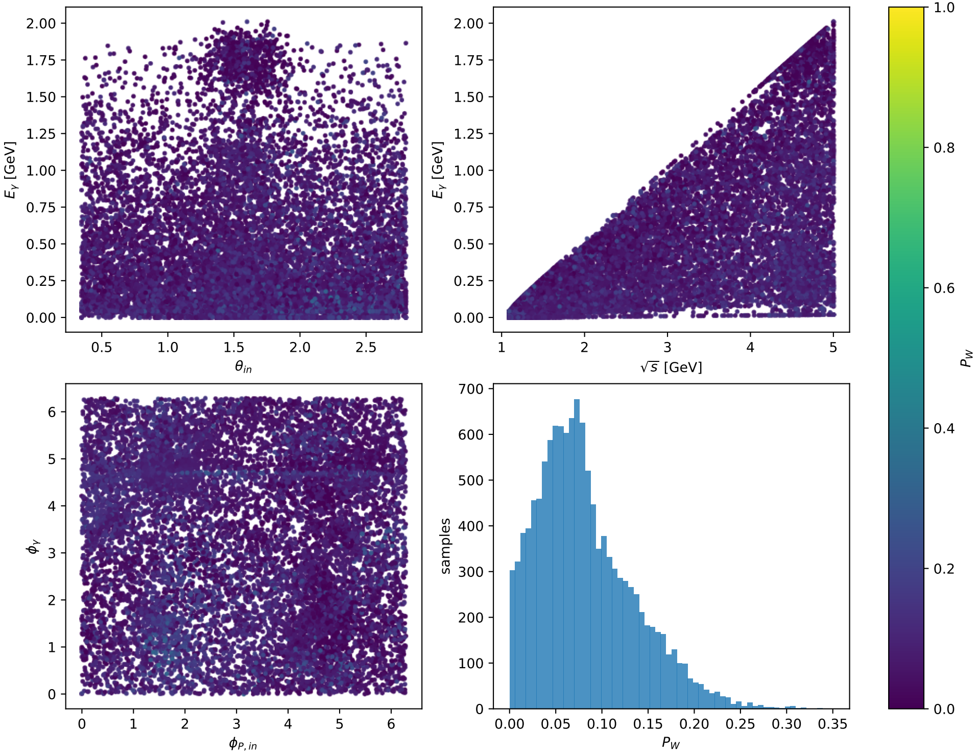
Phase-space scan: Ty muon [Ty_electron], max P_W=0.35065
