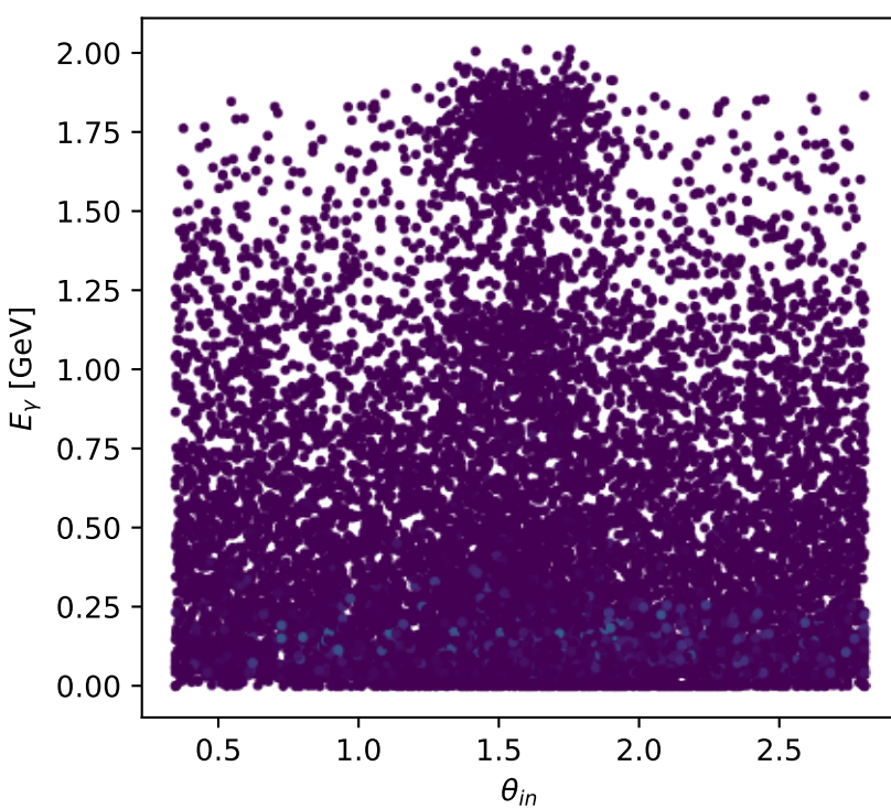
Phase-space scan: Ty muon [Ty_electron], max C_{py}=0.30967
