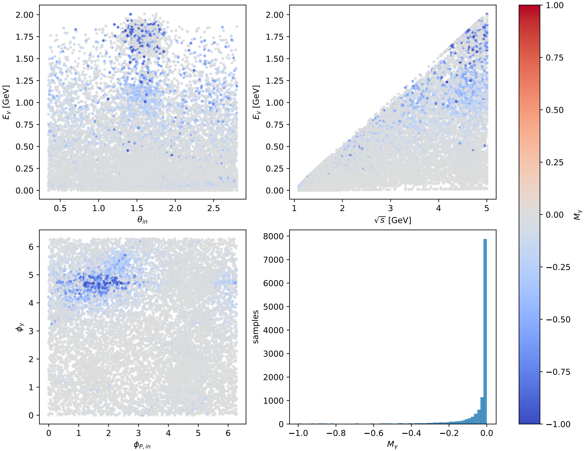
Phase-space scan: Ty muon [Ty_electron], max M_\gamma = -0
