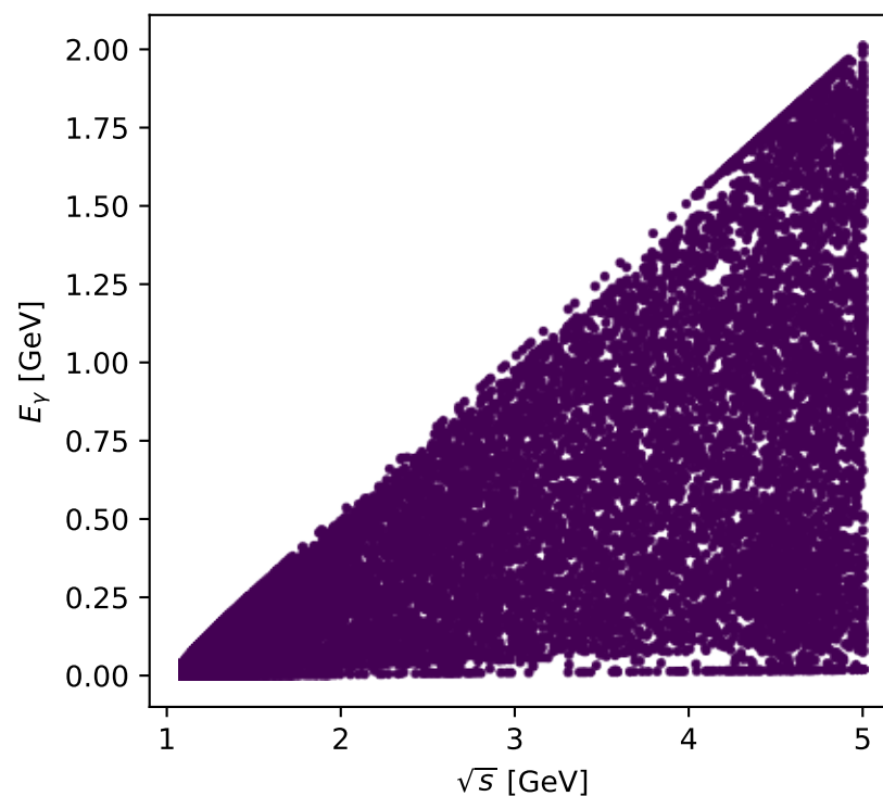
Phase-space scan: Ty muon [Ty_electron], max F_3=0
