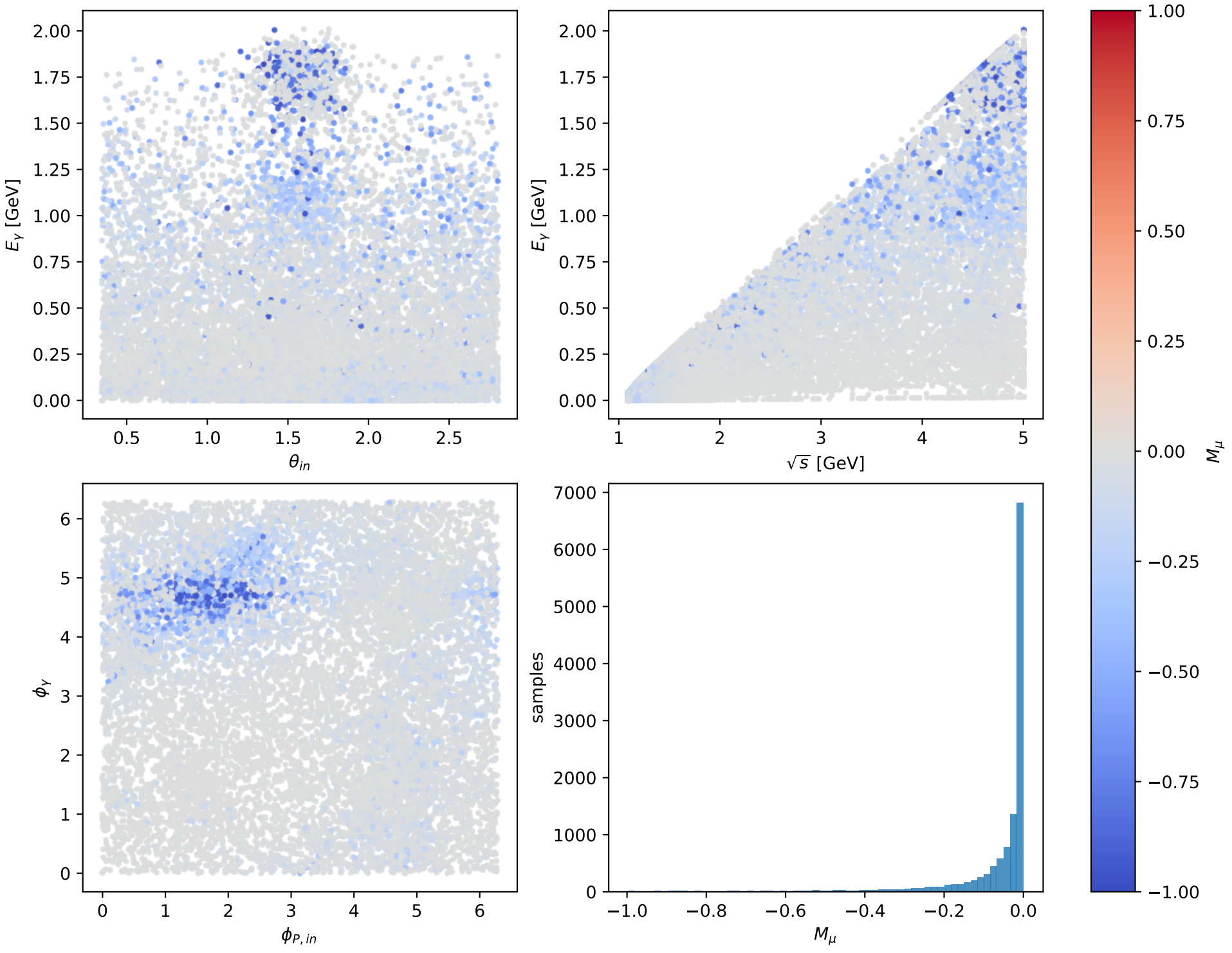
Phase-space scan: Ty muon [Ty_electron], max M_\mu=-0
