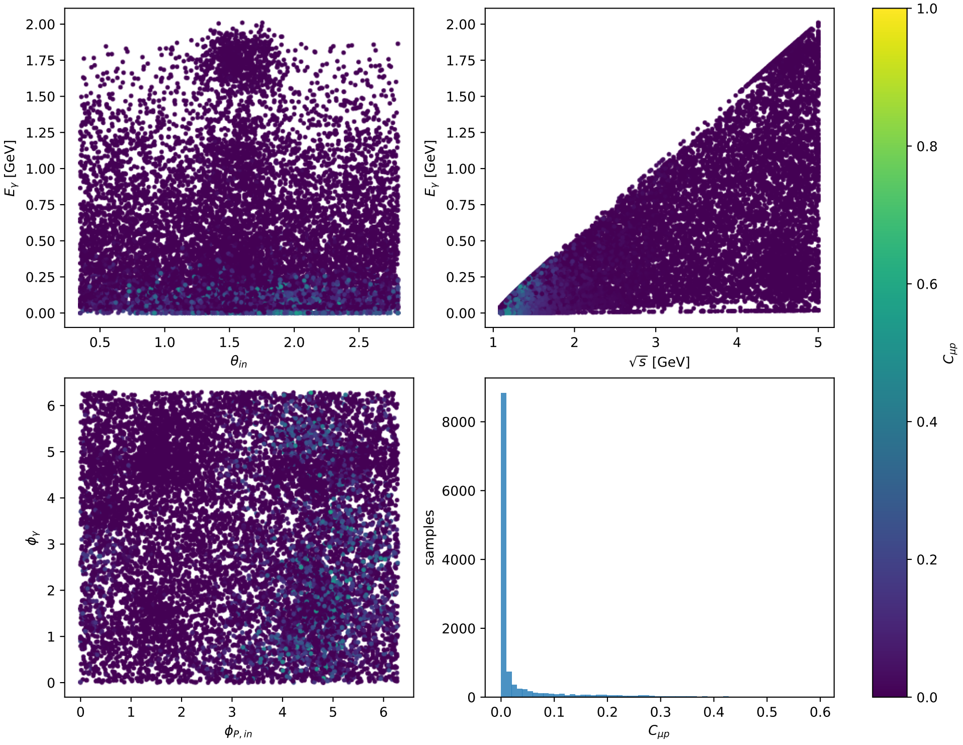
Phase-space scan: Ty muon [Ty_electron], max C_{\mu p}=0.59627
