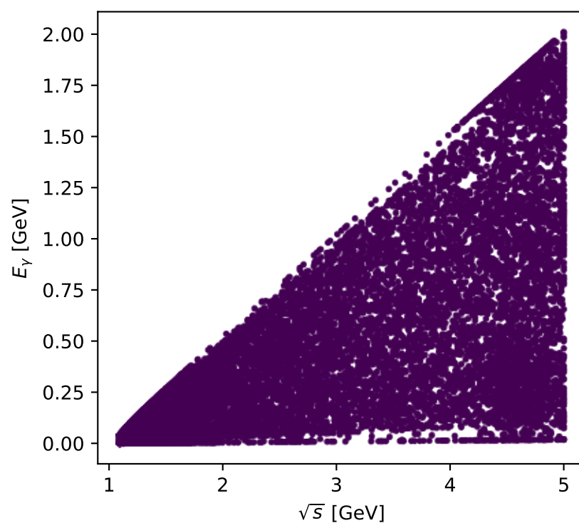
Phase-space scan: Ty muon [Ty_electron], max C_{\mu|p\gamma}=0
