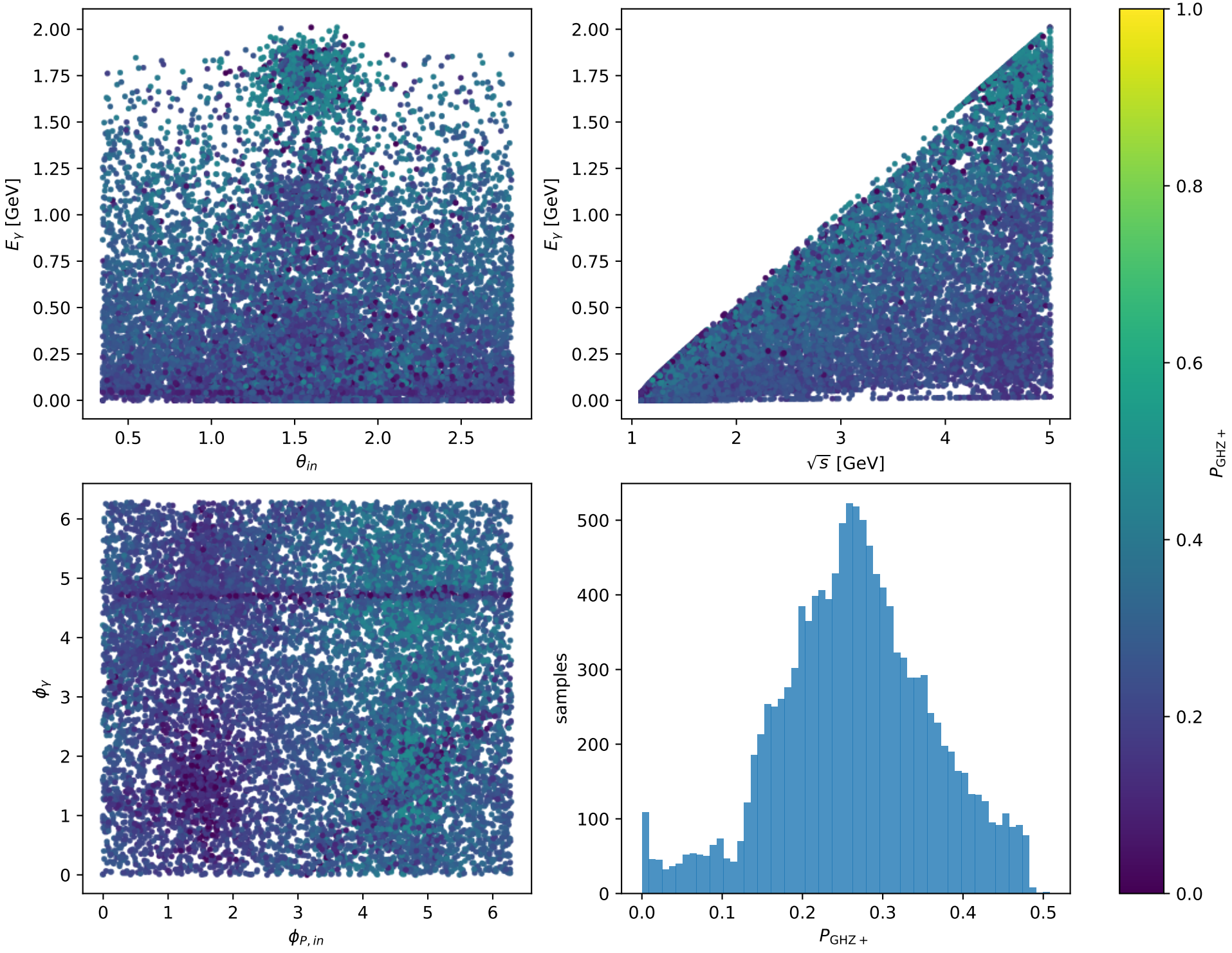
Phase-space scan: Ty muon [Ty_electron], max P_{\text{GHZ}+}=0.50816
