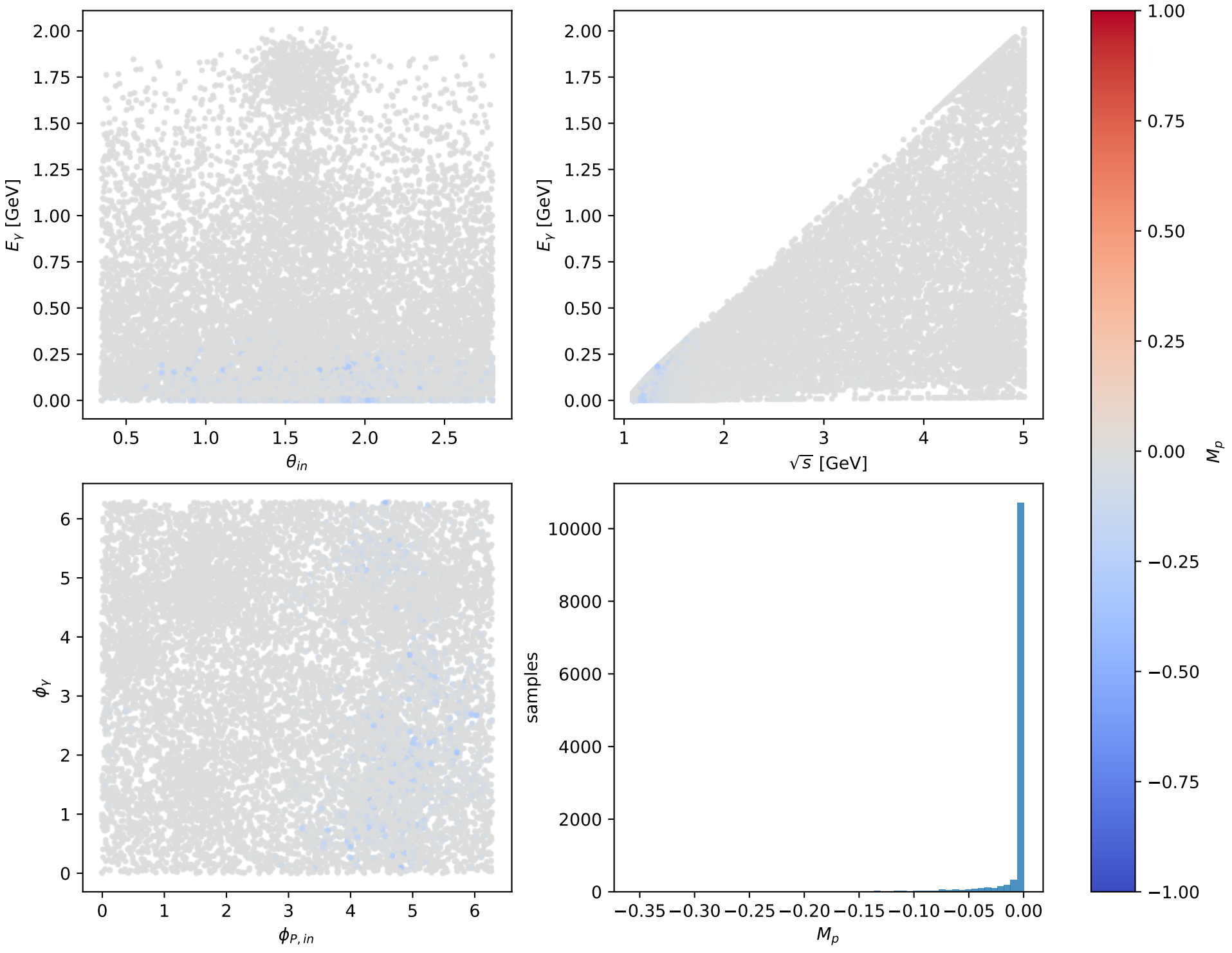
Phase-space scan: Ty muon [Ty_electron], max M_p=-0
