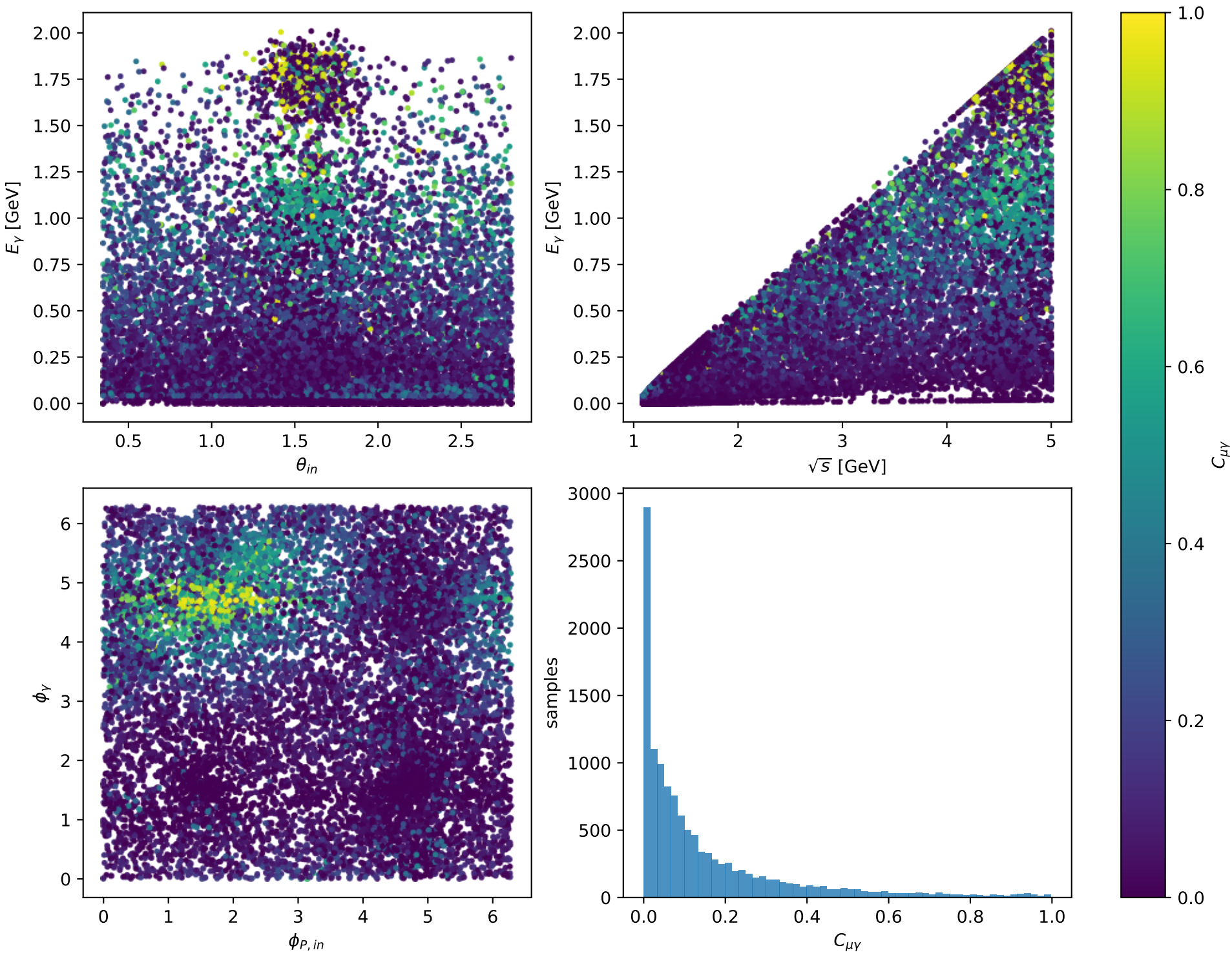
Phase-space scan: Ty muon [Ty_electron], max C_{\mu\gamma}=0.9982
