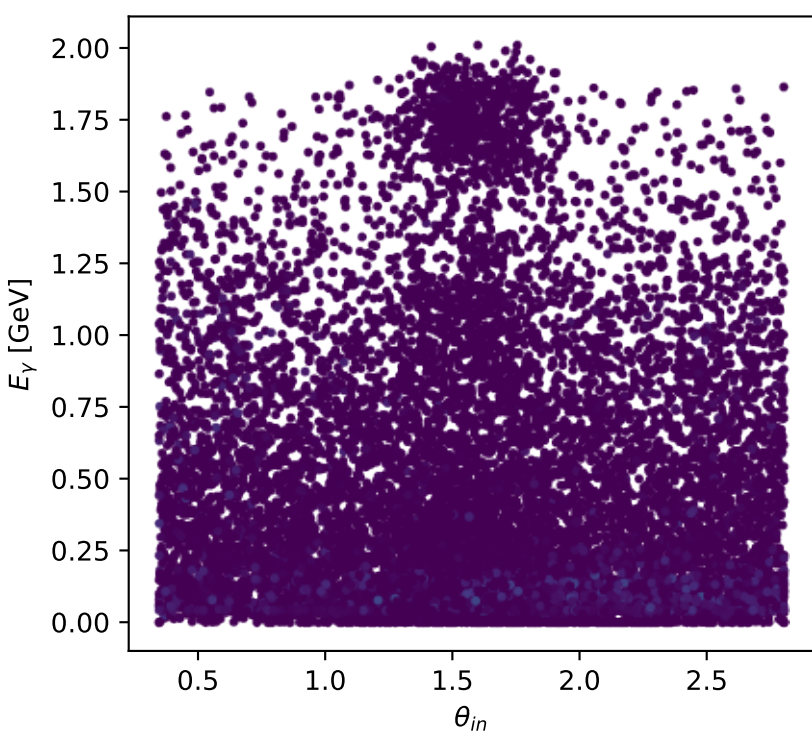
Phase-space scan: Ty proton [Ty_proton], max C_{\mu\gamma}=0.23569
