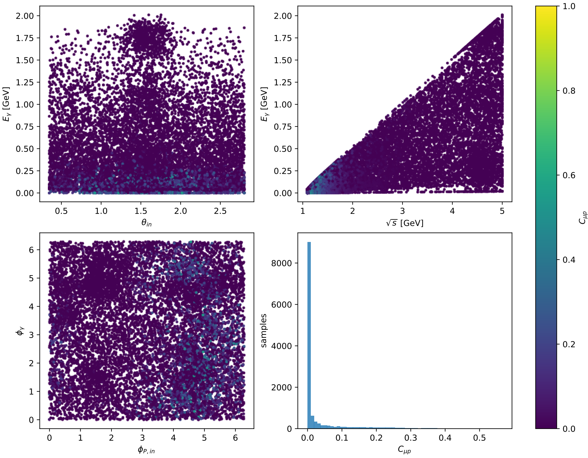
Phase-space scan: Ty proton [Ty_proton], max C_{\mu p}=0.56599
