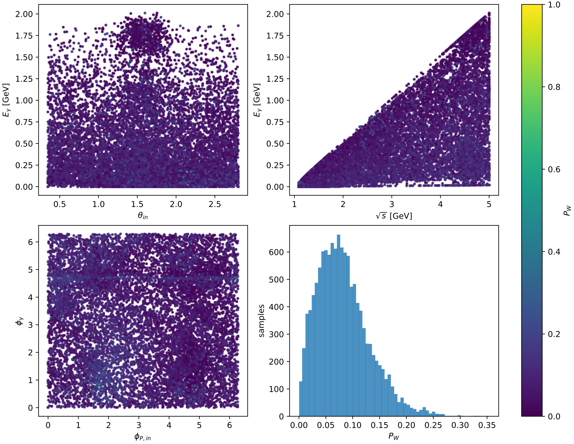
Phase-space scan: Ty proton [Ty_proton], max P_W=0.35388
