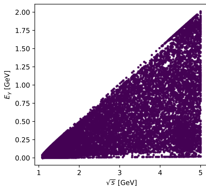
Phase-space scan: Ty proton [Ty_proton], max C_{\mu|p\gamma}=0
