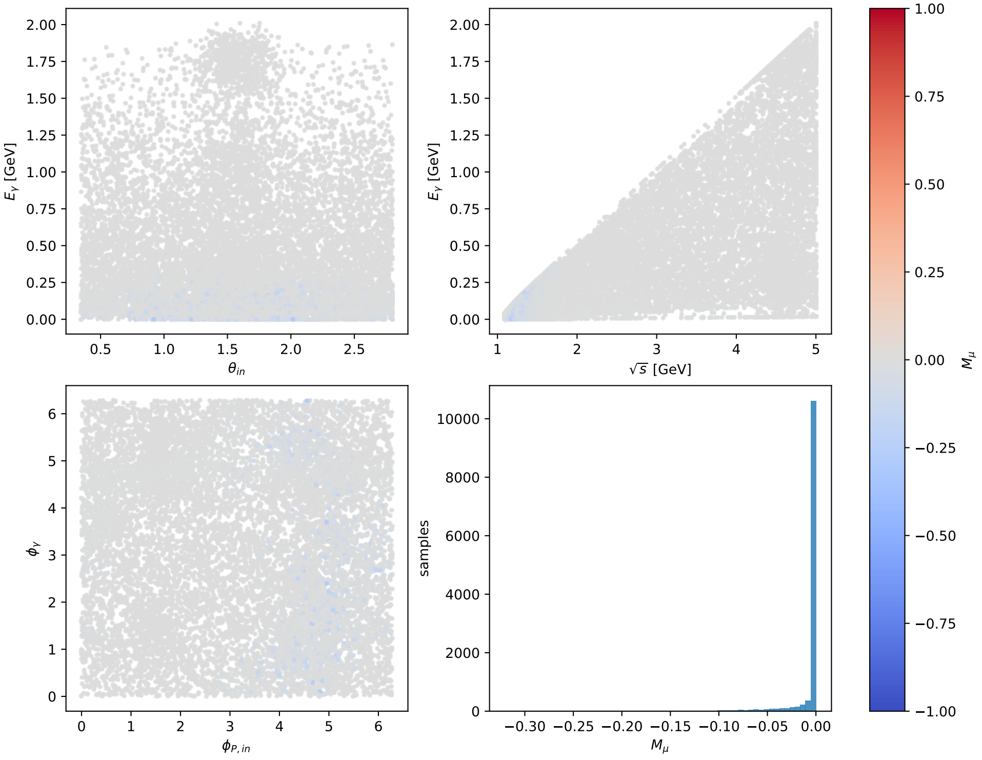
Phase-space scan: Ty proton [Ty_proton], max M_\mu = -0
