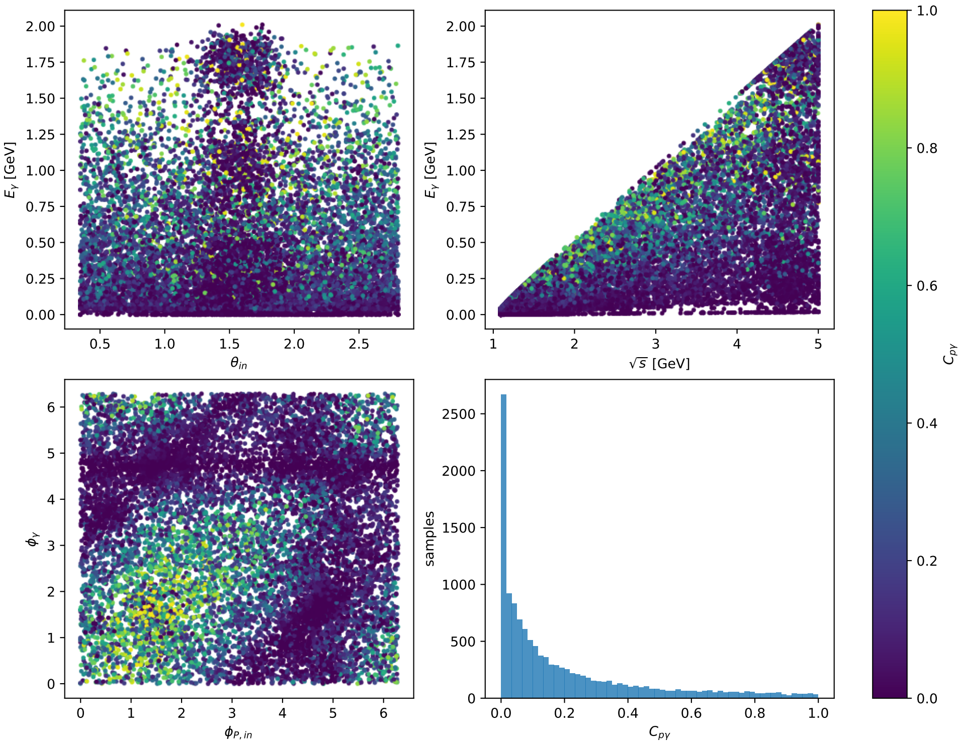
Phase-space scan: Ty proton [Ty_proton], max C_{p\gamma}=0.99999
