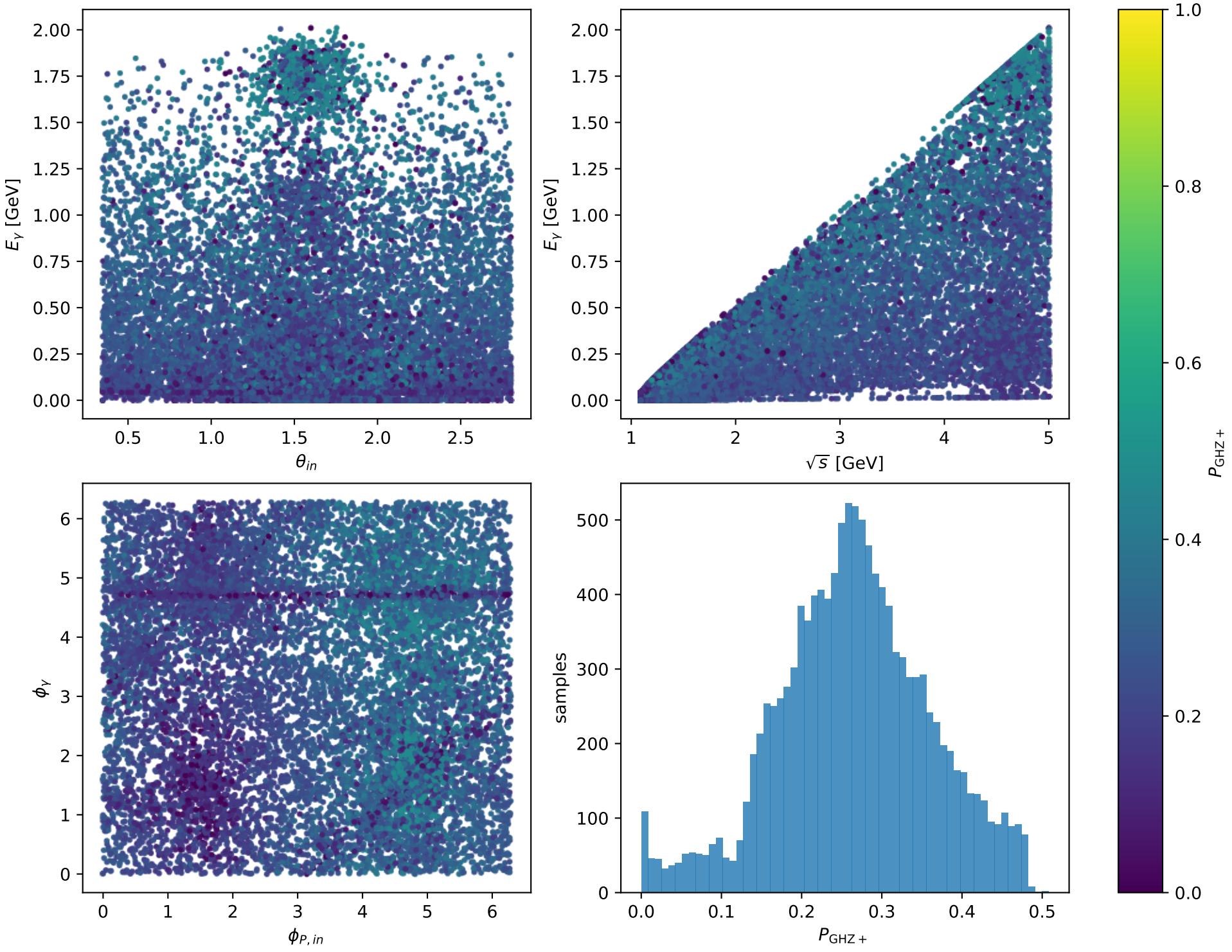
Phase-space scan: Ty proton [Ty_proton], max P_{\text{GHZ}+}=0.50816
