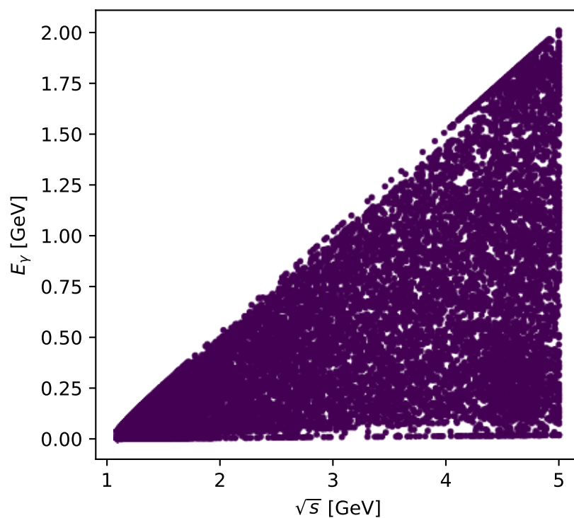
Phase-space scan: Ty proton [Ty_proton], max C_{p|\mu\gamma}=0
