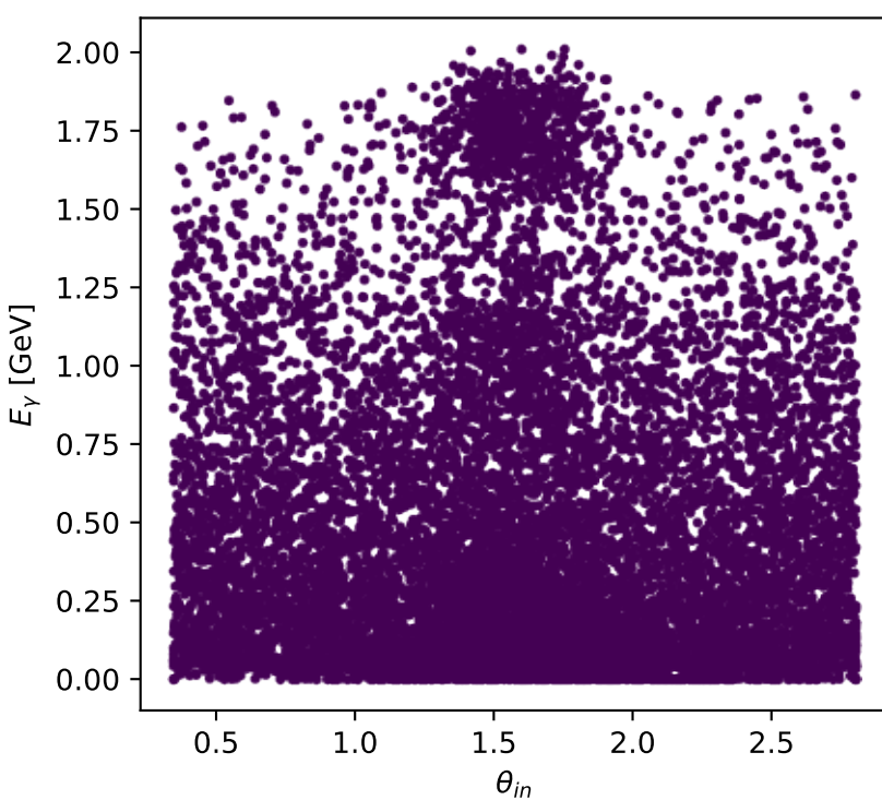
Phase-space scan: Ty proton [Ty_proton], max C_{\mu|p\gamma}=0
