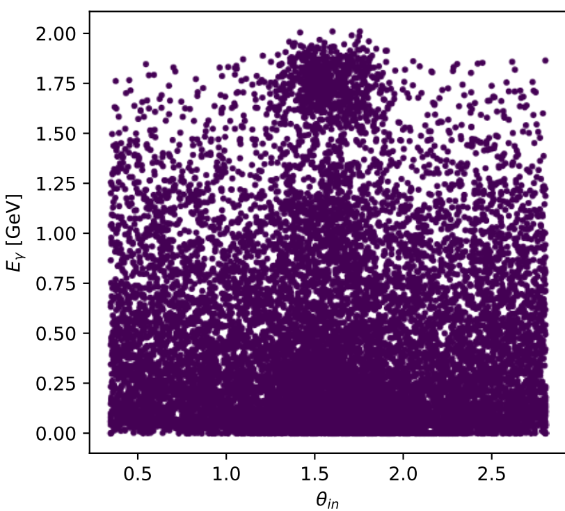
Phase-space scan: Unpolarized [unpolarized], max C_{\mu\gamma}=0
