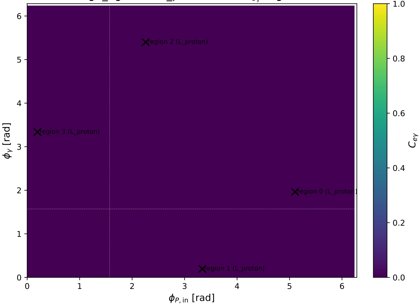
high_Egamma L_proton: max C_{ey} regions
