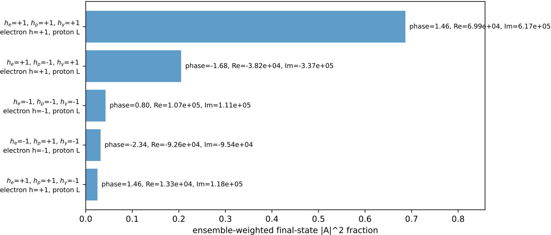
Leading initial-ensemble/final-state components (N=5, retained=99.0%)
