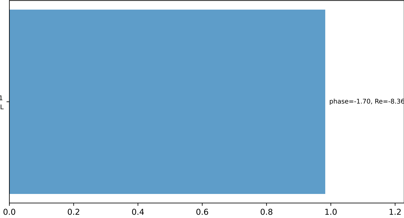
Leading initial-ensemble/final-state components (N=1, retained=98.2%)
