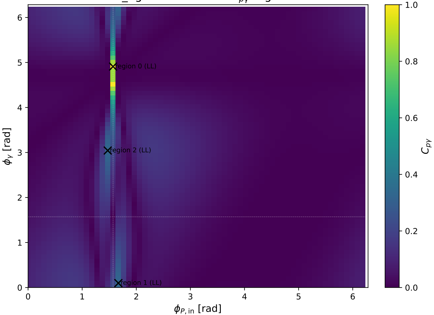
mid_Egamma LL: max C_{pY} regions
