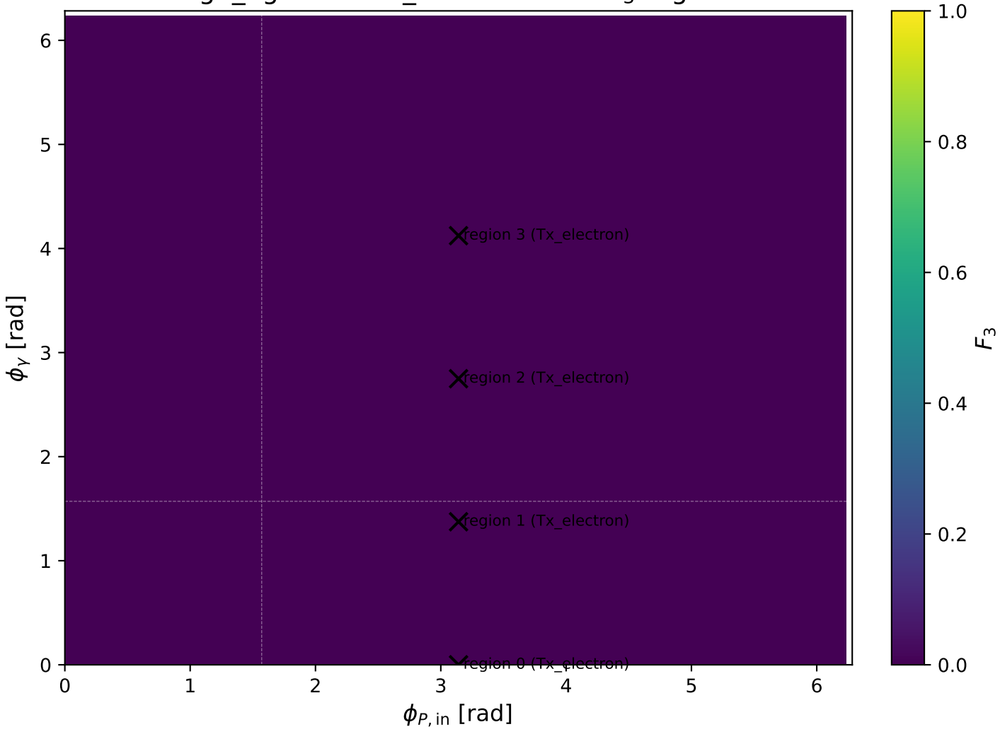
high_Egamma Tx_electron: max F_3 regions
