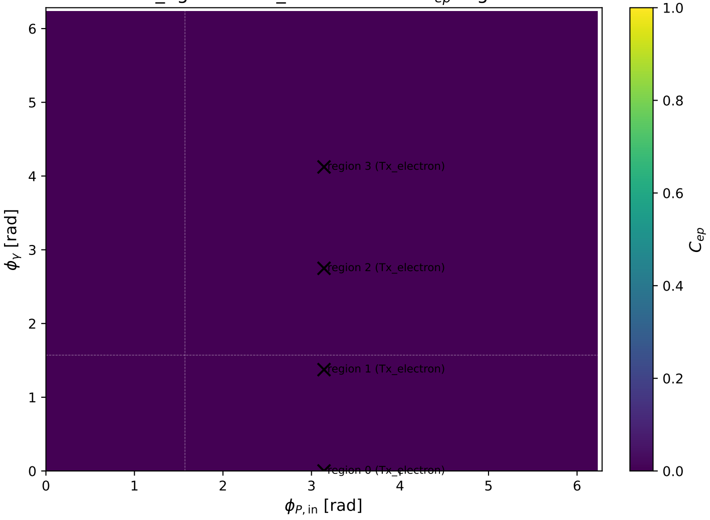
mid_Egamma Tx_electron: max C_{ep} regions
