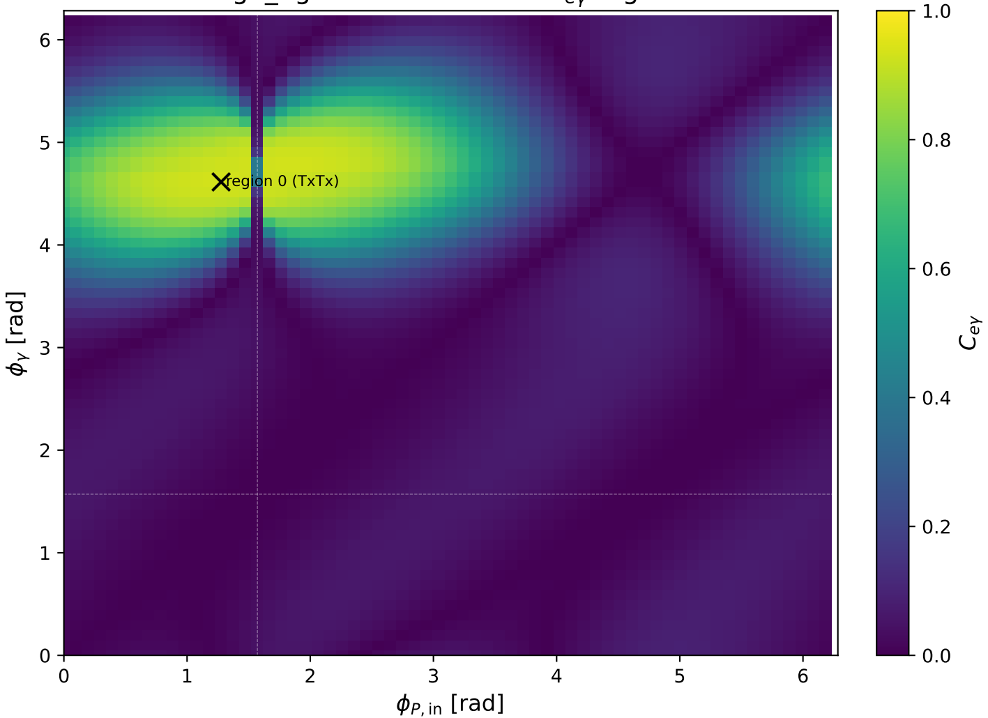
high_Egamma TxTx: max C_{e\gamma} regions
