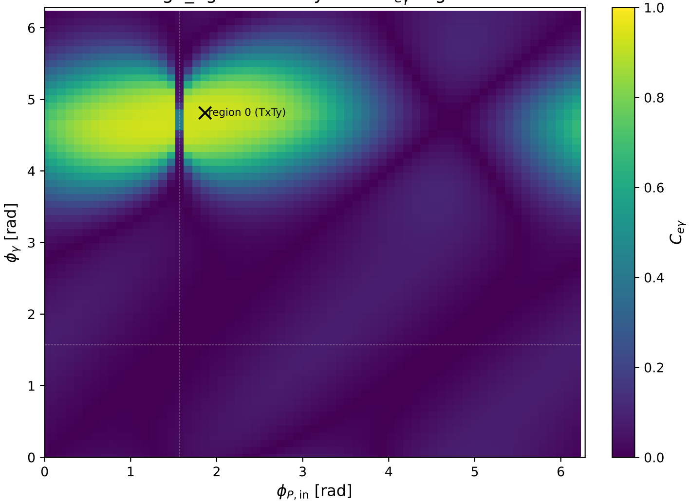
high_Egamma TxTy: max C_{e\gamma} regions
