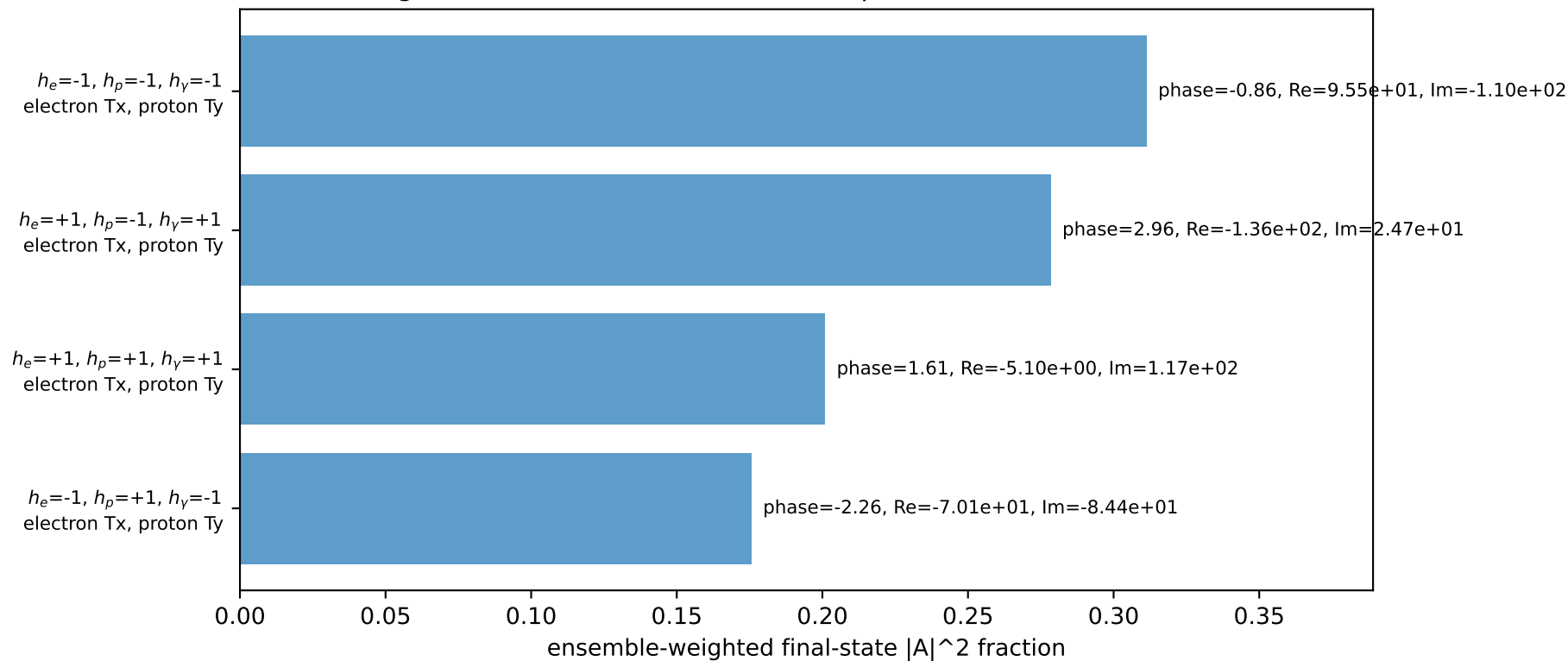
Leading initial-ensemble/final-state components (N=4, retained=96.6%)
