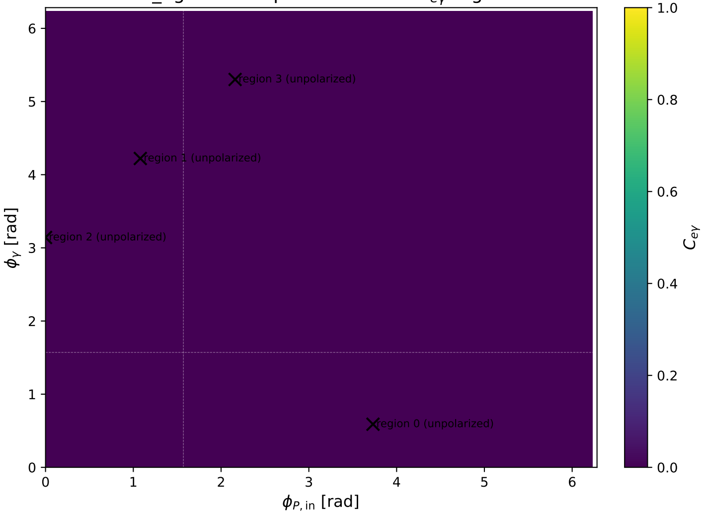
low_Egamma unpolarized: max C_{ey} regions
