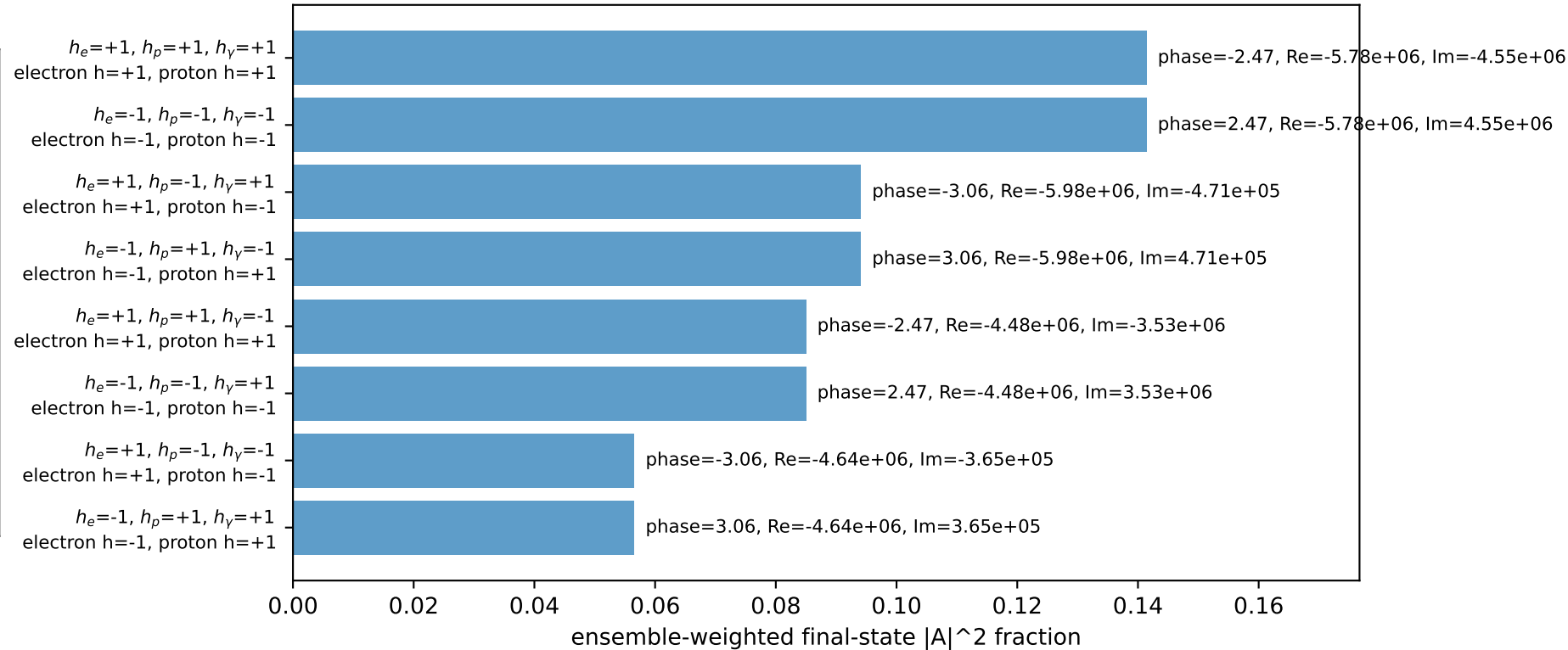
Leading initial-ensemble/final-state components (N=8, retained=75.4%)
