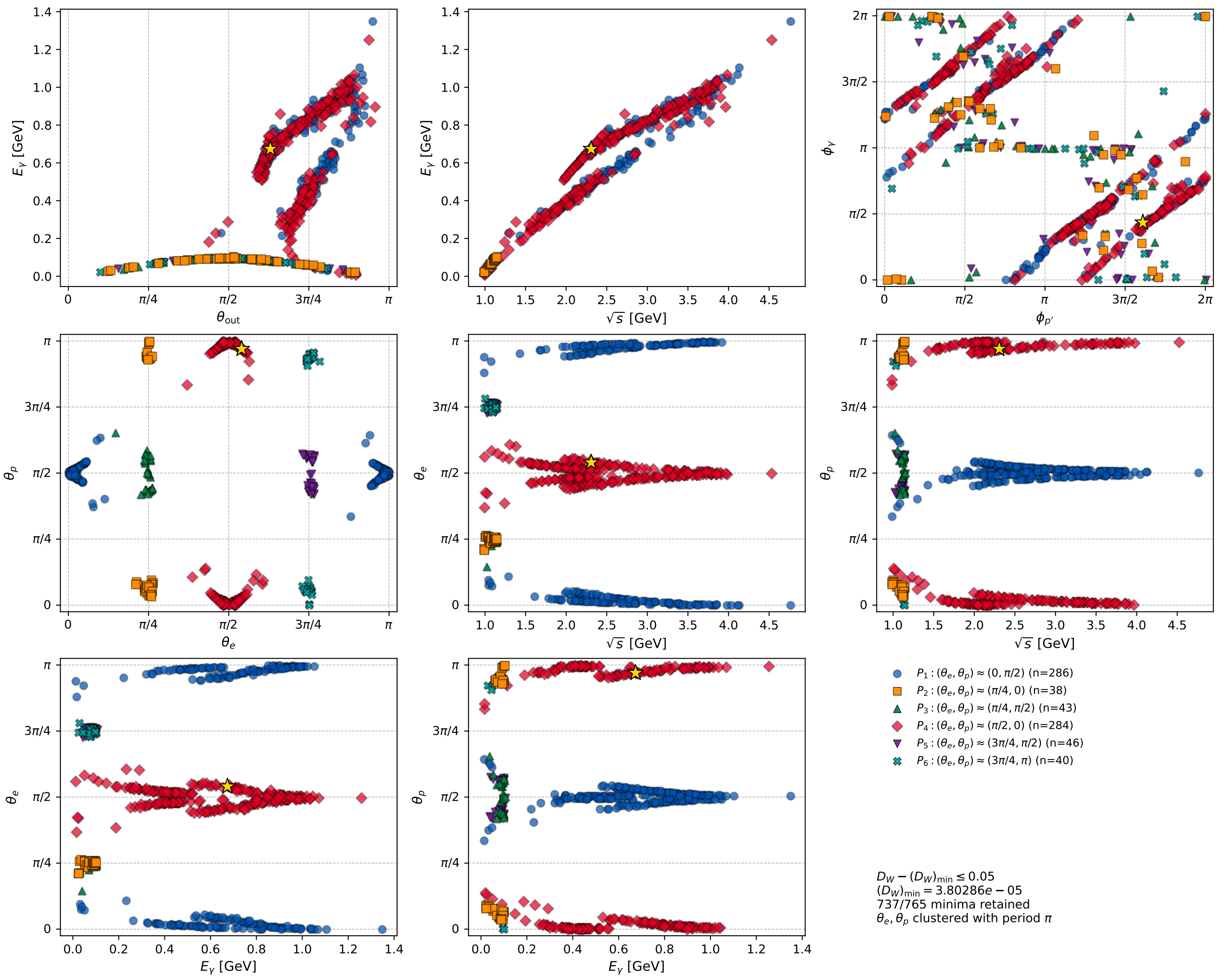
electron: low- D_W phase space colored by six major polarization configurations
