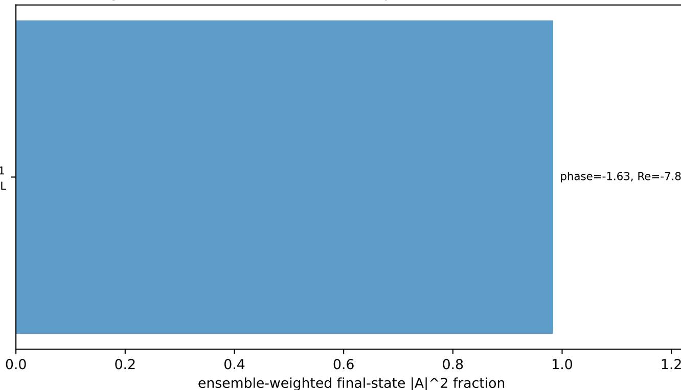
Leading initial-ensemble/final-state components (N=1, retained=98.3%)
