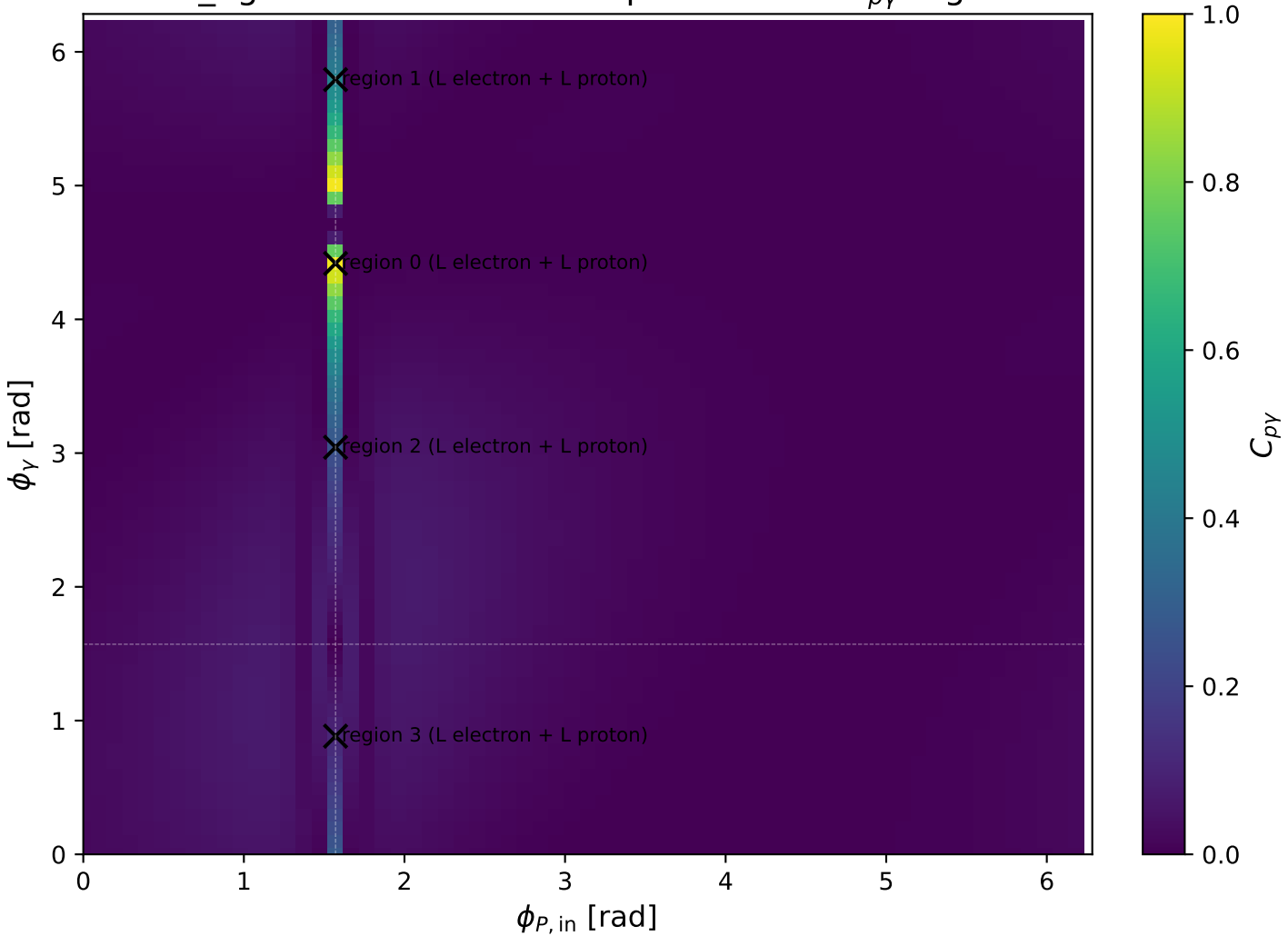
low_Egamma L electron + L proton: max C_{p\gamma} regions
