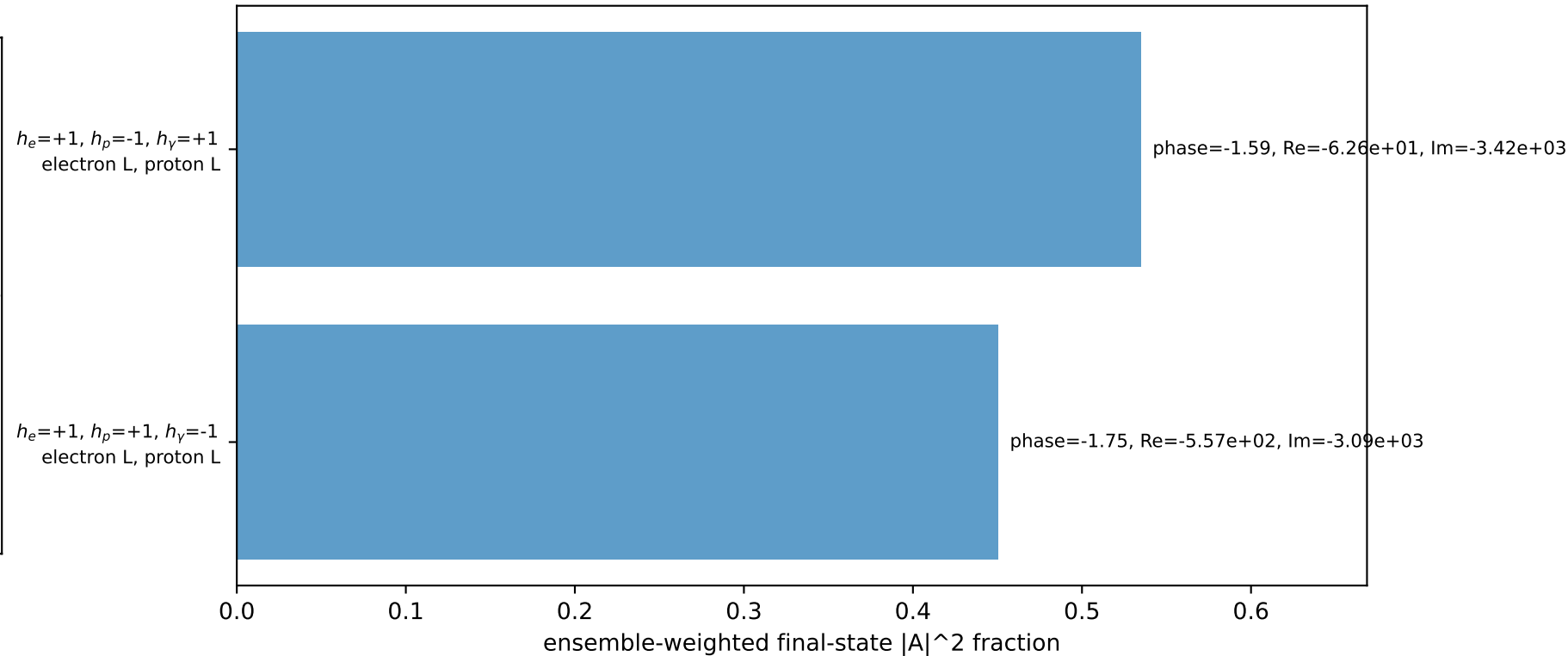
Leading initial-ensemble/final-state components (N=2, retained=98.5%)
