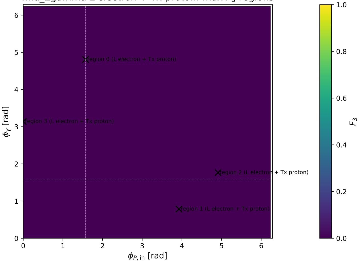
mid_Egamma L electron + Tx proton: max F_3 regions
