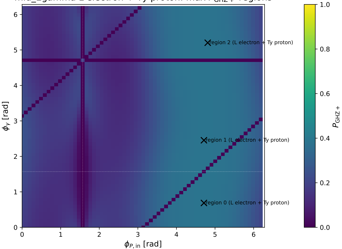
mid_Egamma L electron + Ty proton: max P_{\text{GHZ}} + regions
