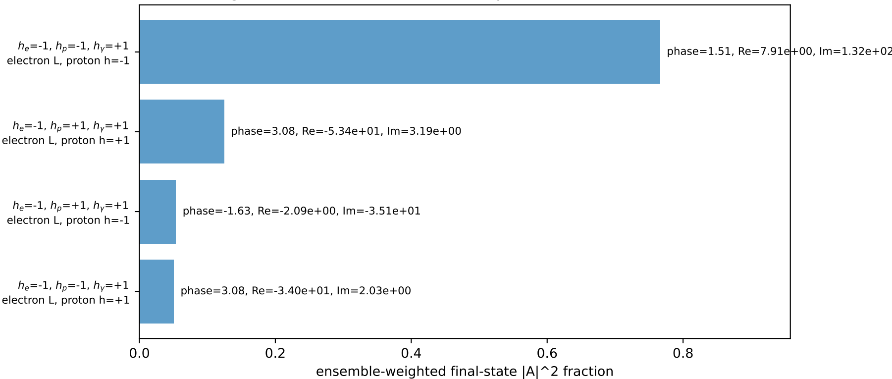
Leading initial-ensemble/final-state components (N=4, retained=99.5%)
