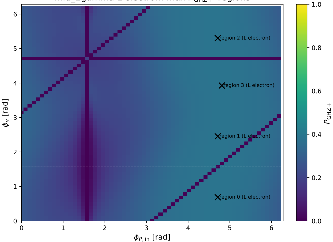
mid_Egamma L electron: max P_{\text{GHz}+} regions
