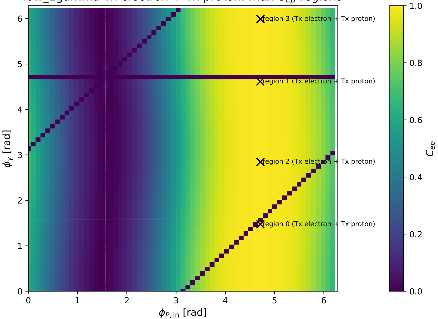
low_Egamma Tx electron + Tx proton: max C_{ep} regions
