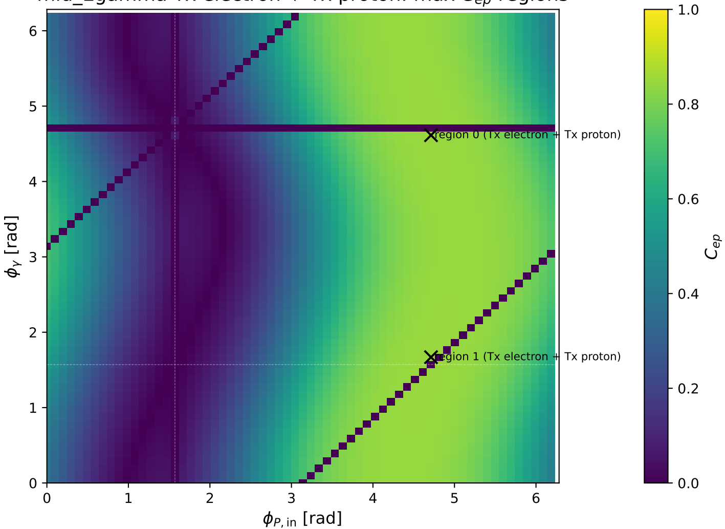
mid_Egamma Tx electron + Tx proton: max C_{ep} regions
