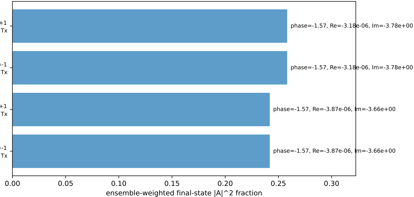
Leading initial-ensemble/final-state components (N=4, retained=100.0%)
