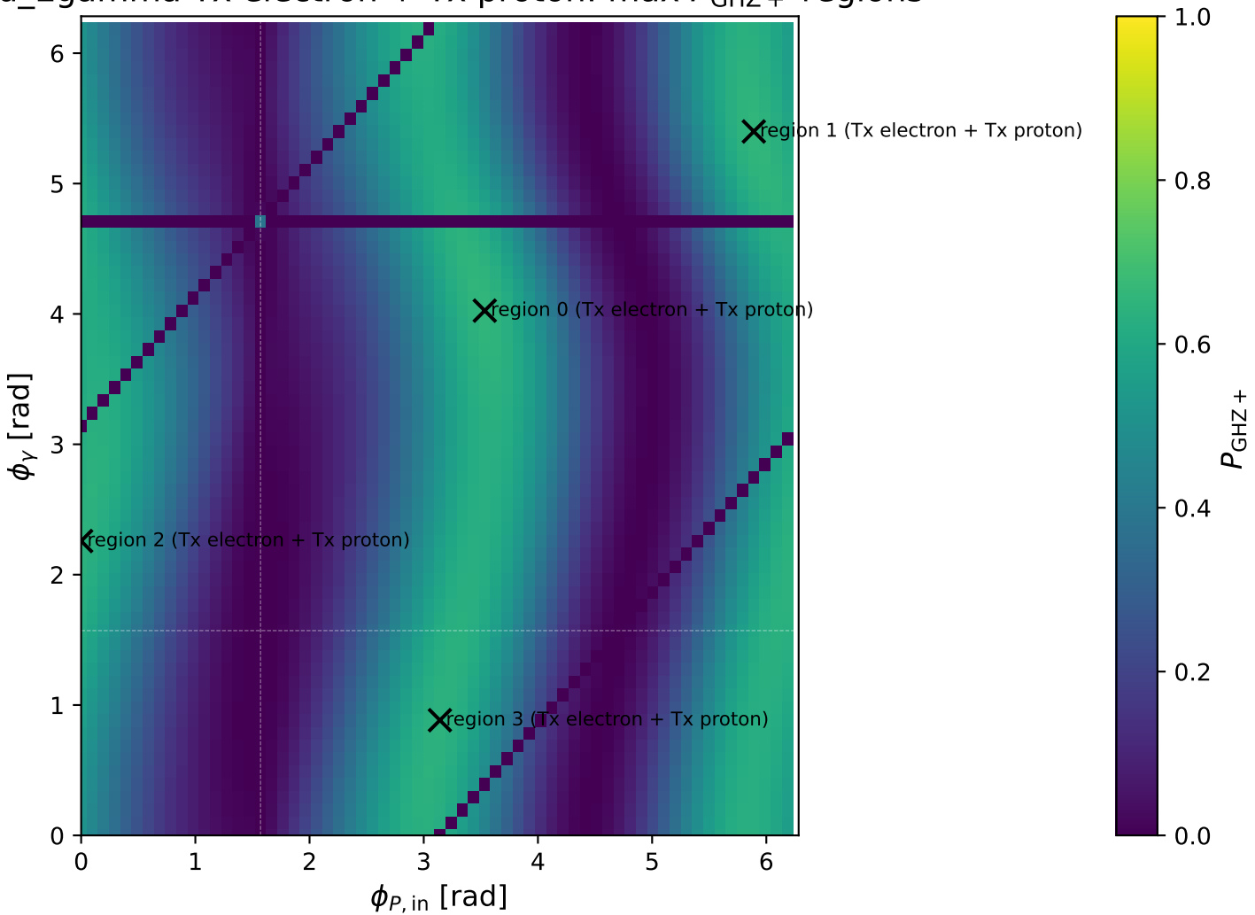
d_Egamma Tx electron + Tx proton: max P_{\text{GHz}} + regions
