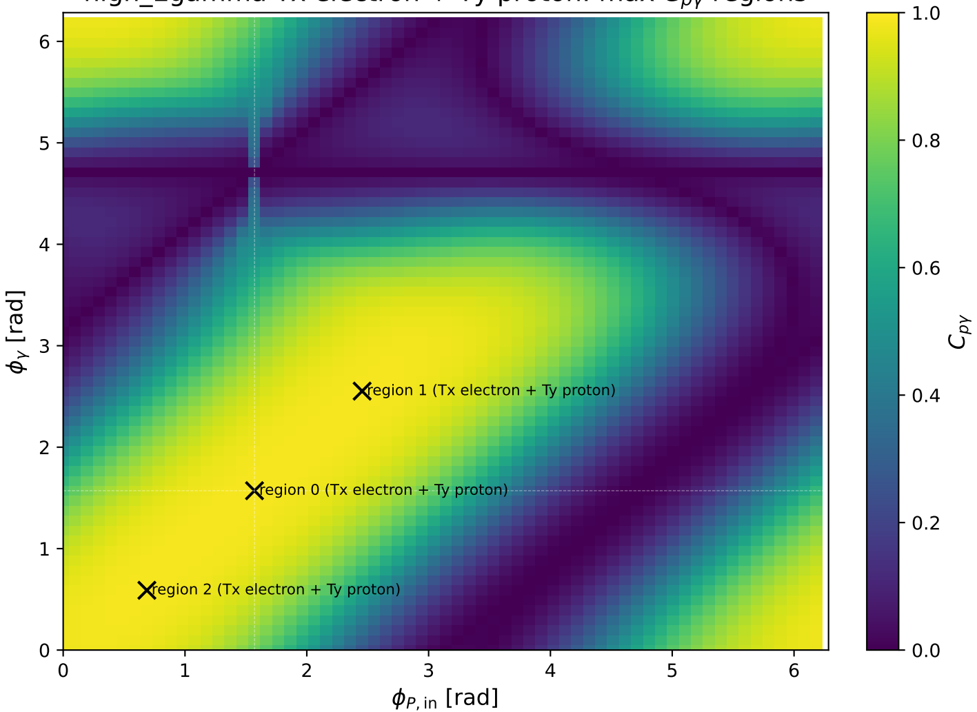
high_Egamma Tx electron + Ty proton: max C_{py} regions
