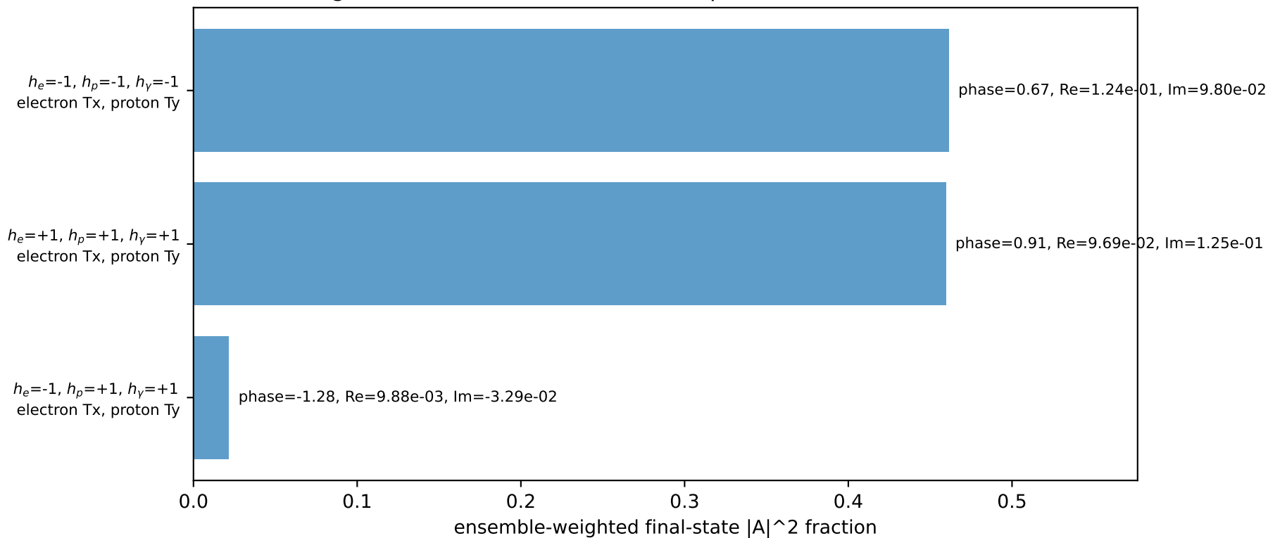
Leading initial-ensemble/final-state components (N=3, retained=94.3%)
