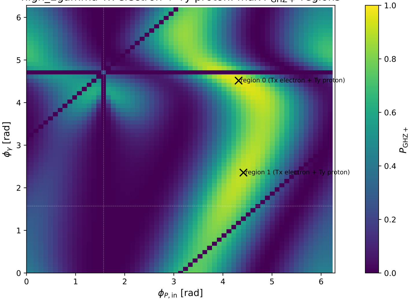
high_Egamma Tx electron + Ty proton: max P_{\text{GHZ}} + regions
