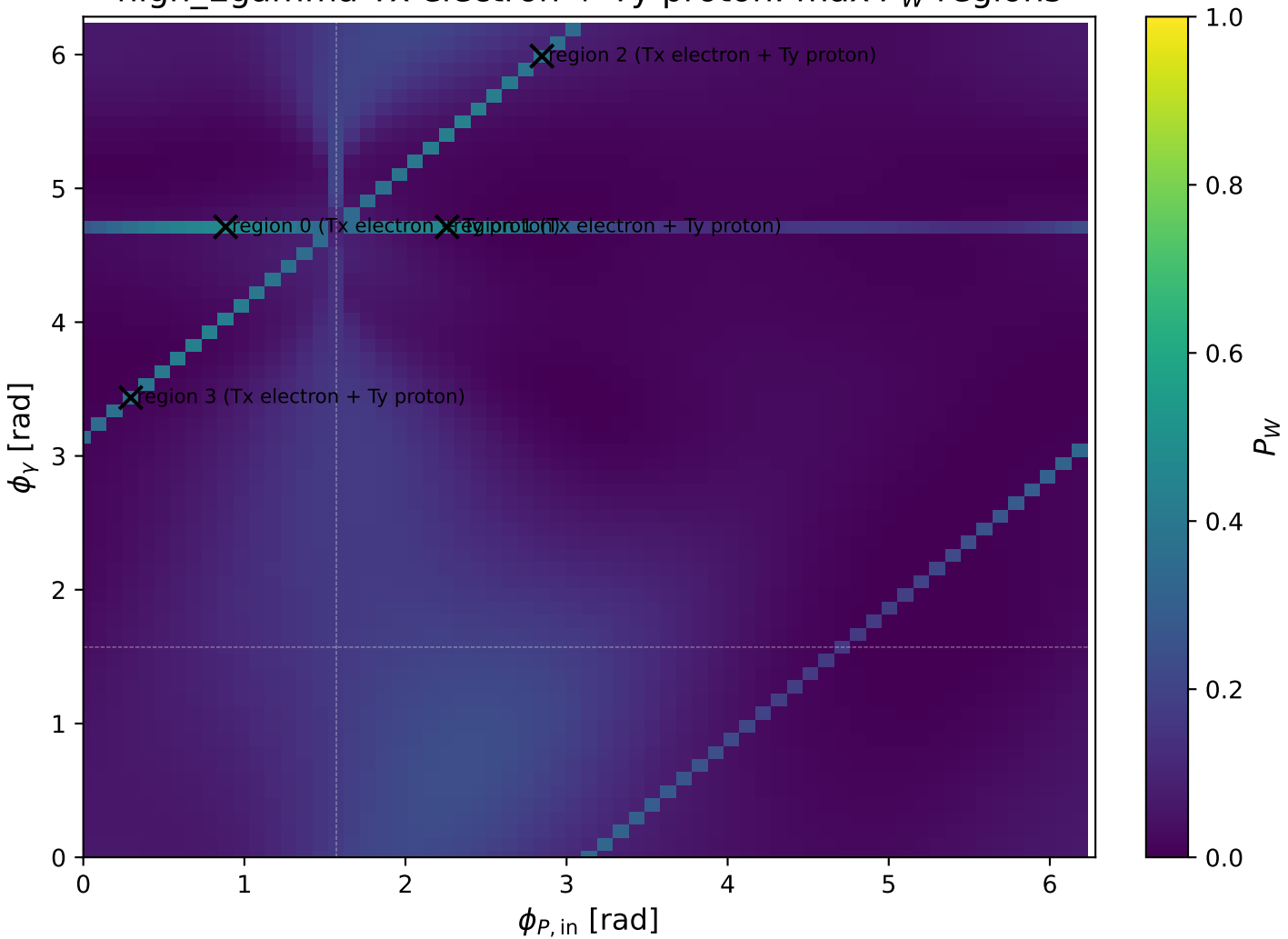
high_Egamma Tx electron + Ty proton: max P_W regions
