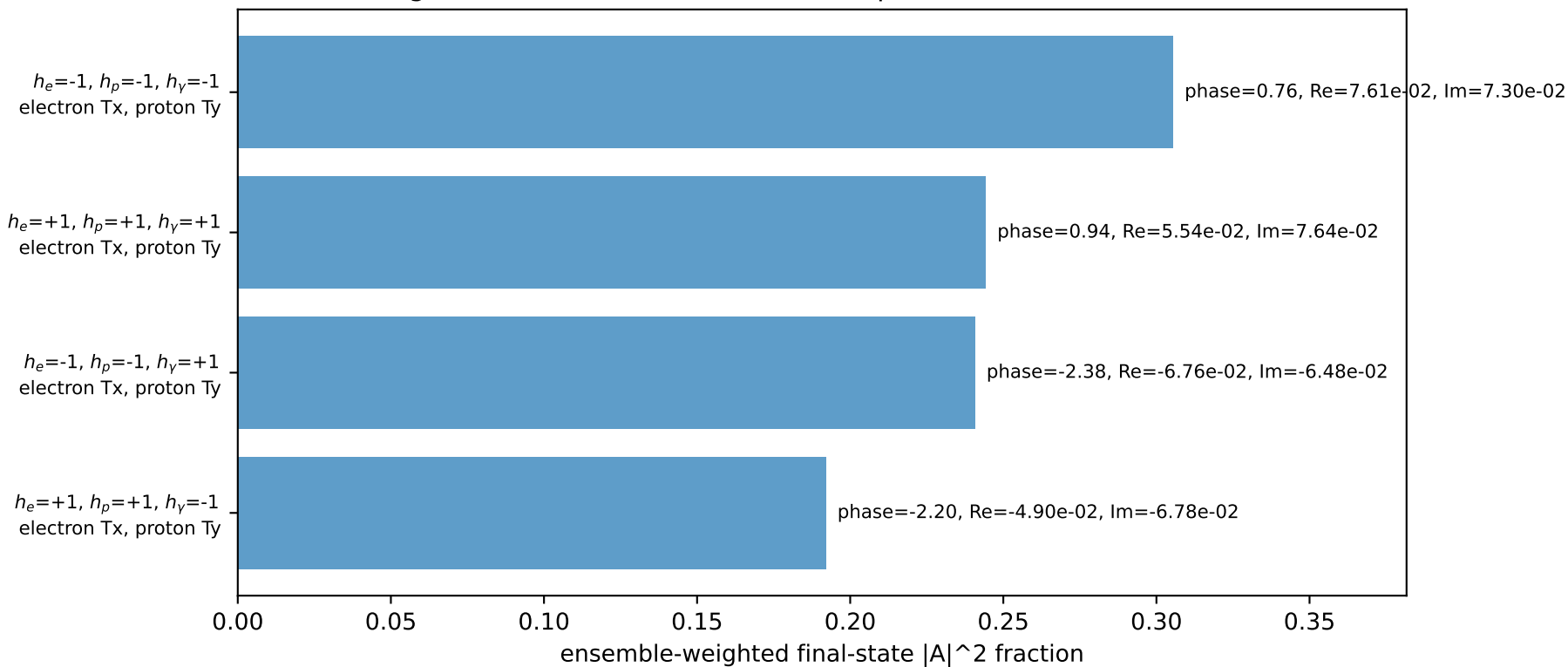
Leading initial-ensemble/final-state components (N=4, retained=98.2%)
