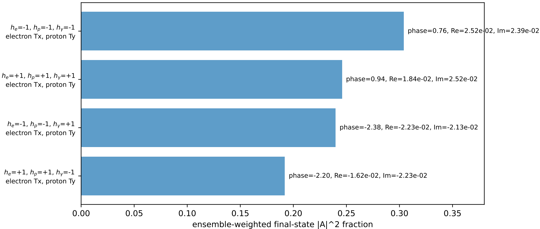
Leading initial-ensemble/final-state components (N=4, retained=98.1%)
