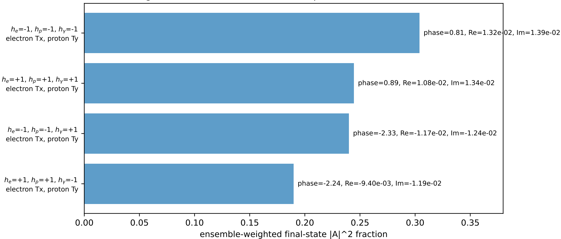
Leading initial-ensemble/final-state components (N=4, retained=97.8%)
