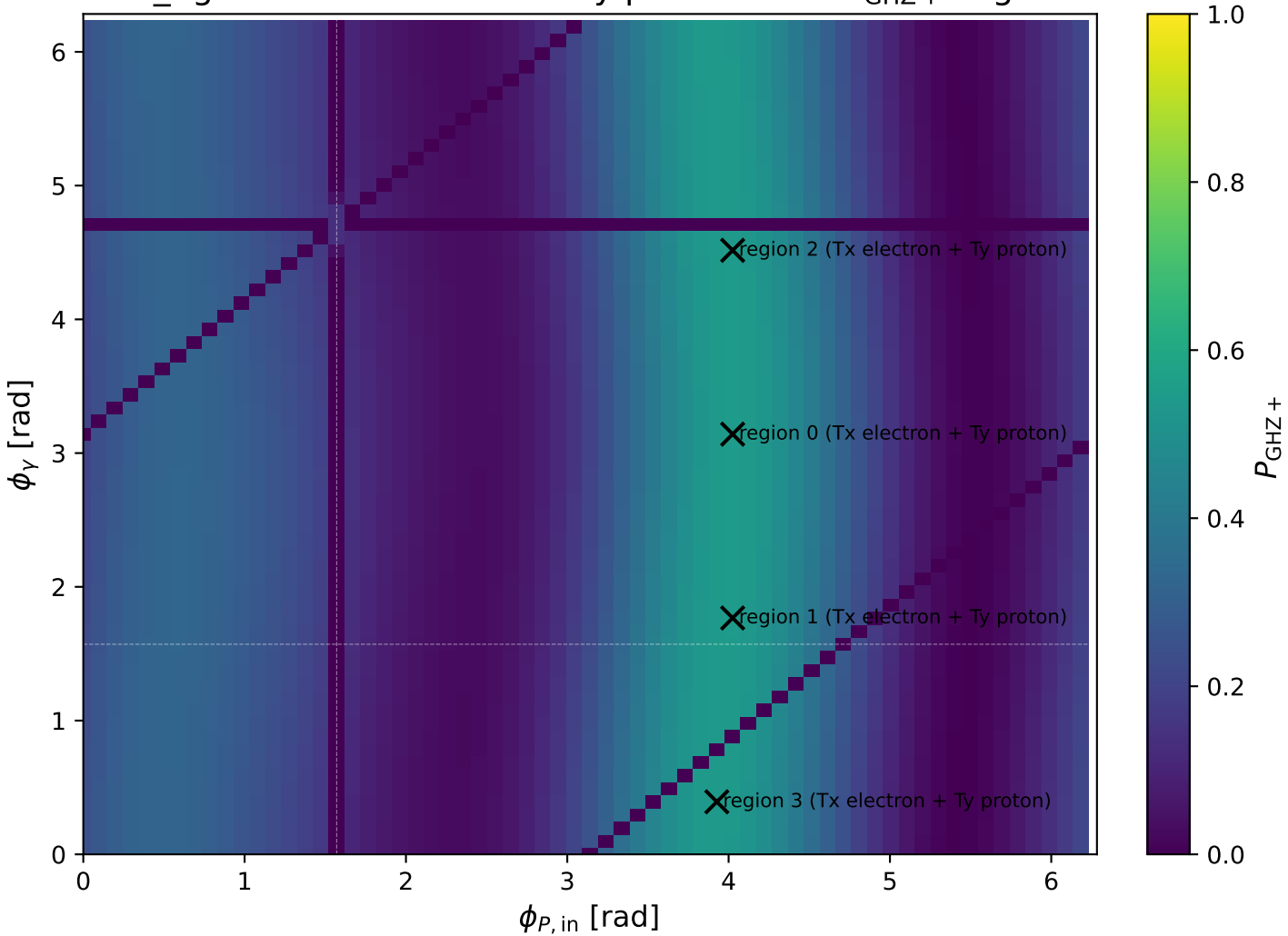
low_Egamma Tx electron + Ty proton: max P_{\text{GHZ}+} regions
