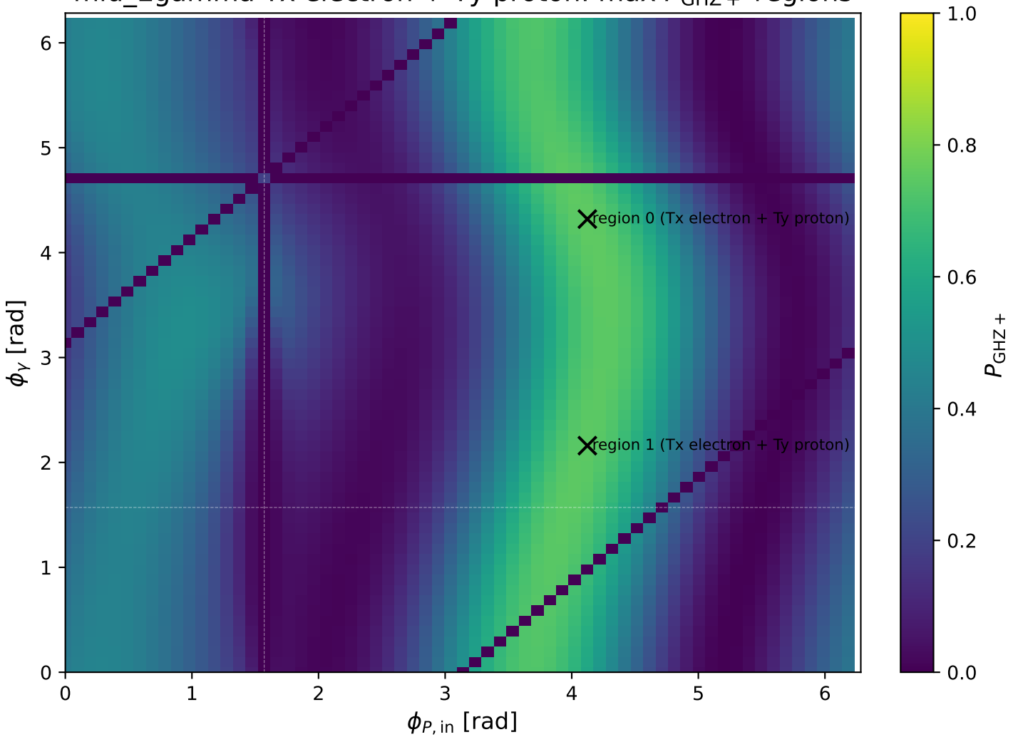
mid_Egamma Tx electron + Ty proton: max P_{\text{GHZ}+} regions
