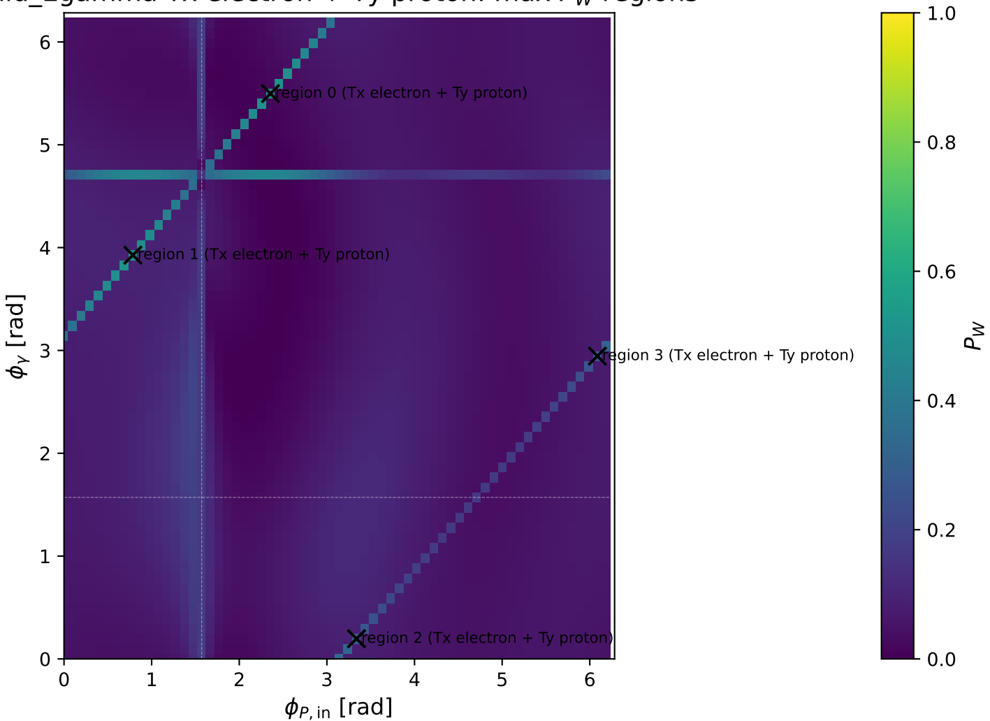
Mid_Egamma Tx electron + Ty proton: max P_W regions
