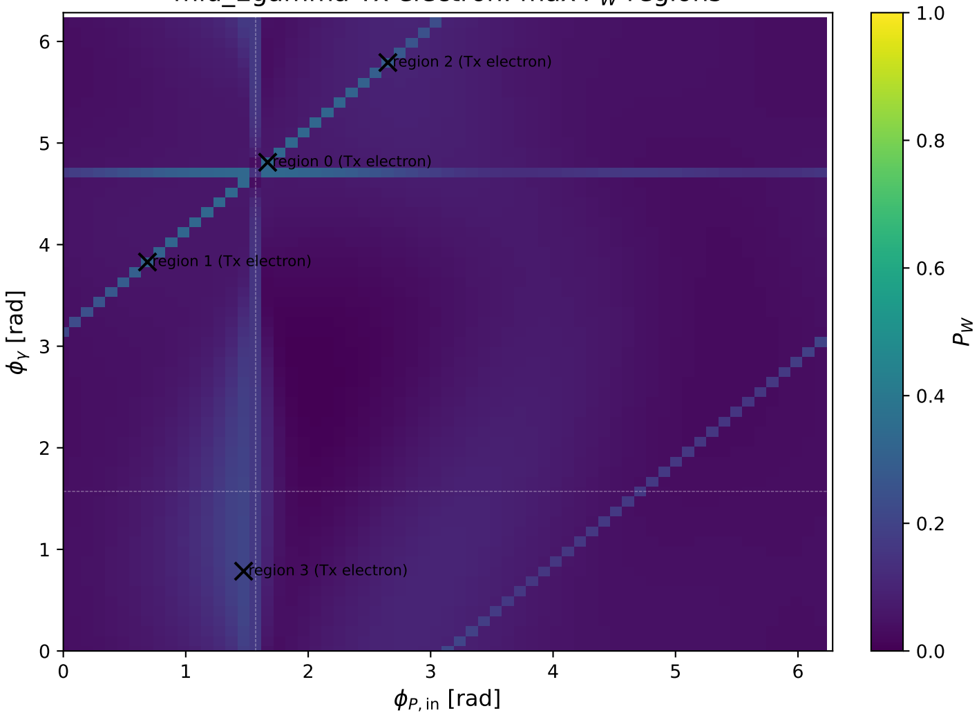
mid_Egamma Tx electron: max P_W regions
