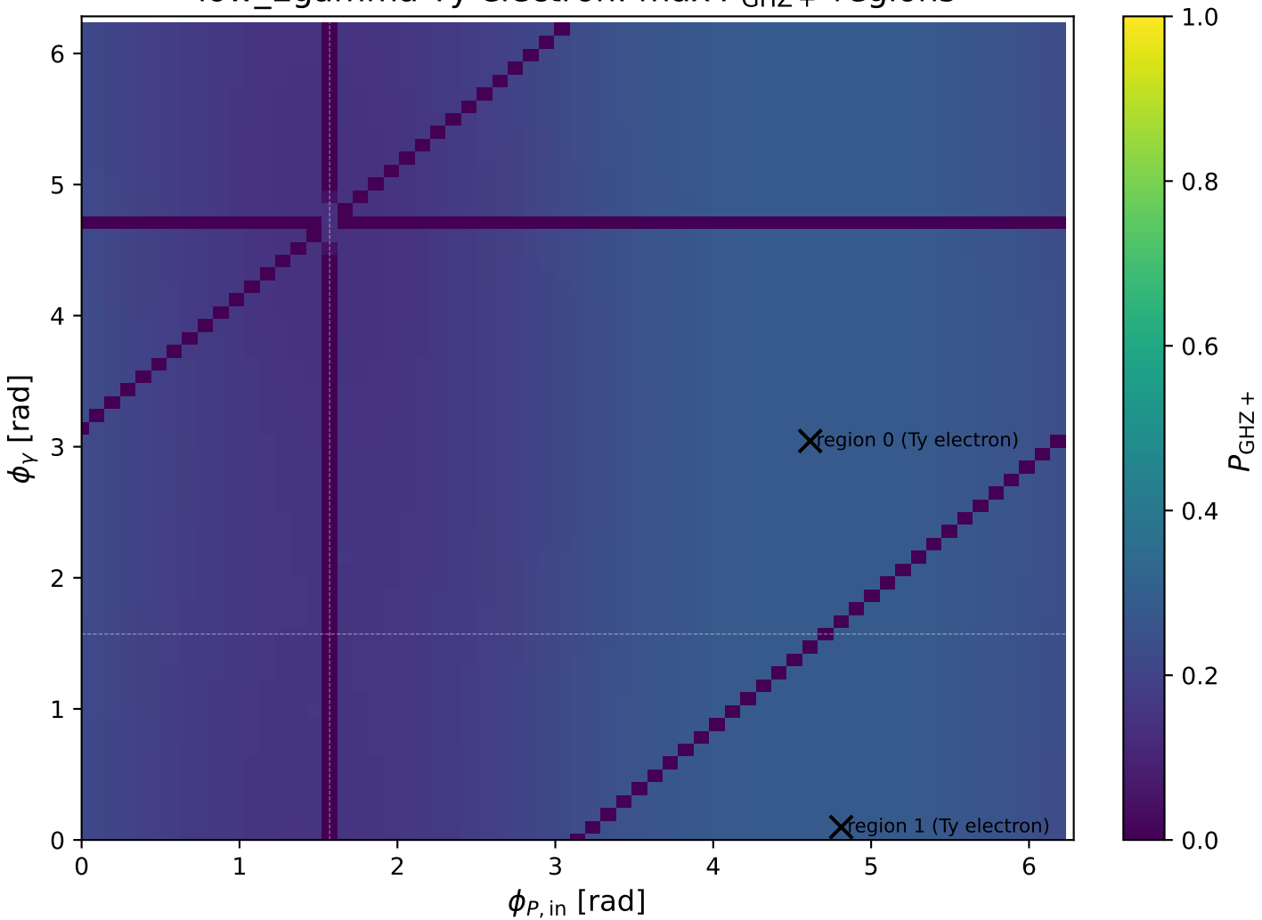
low_Egamma Ty electron: max P_{\text{GHz}+} regions
