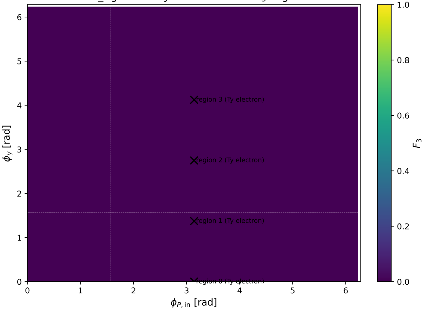
mid_Egamma Ty electron: max F_3 regions
