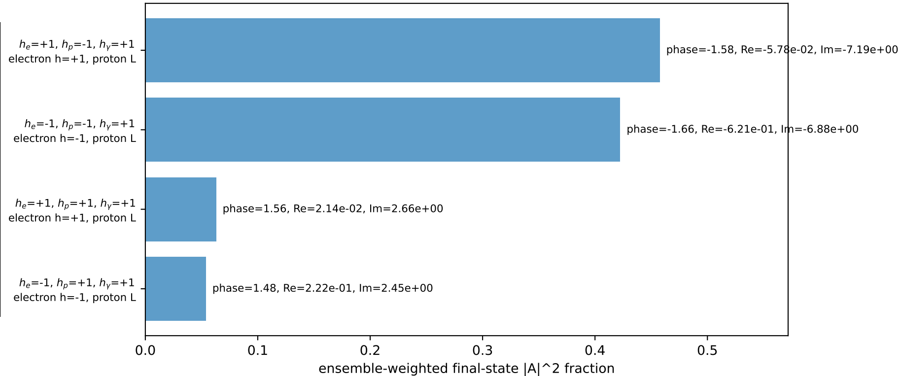
Leading initial-ensemble/final-state components (N=4, retained=99.6%)
