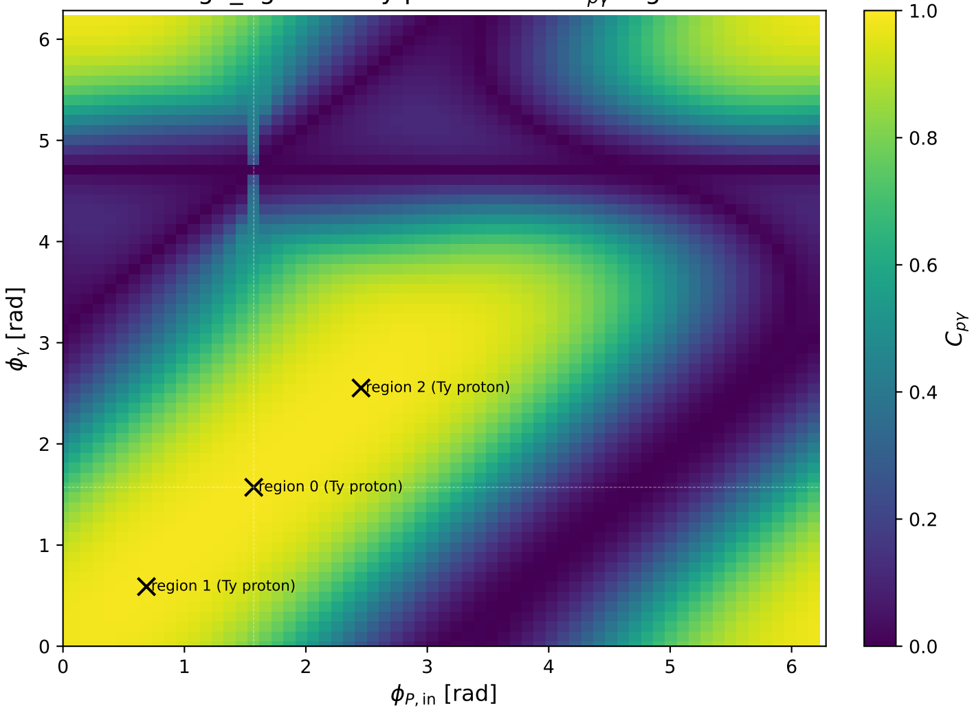
high_Egamma Ty proton: max C_{p\gamma} regions
