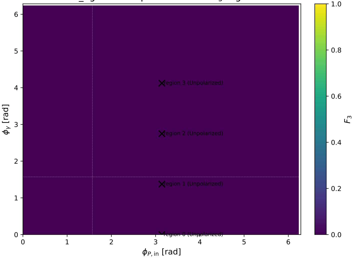
low_Egamma Unpolarized: max F_3 regions
