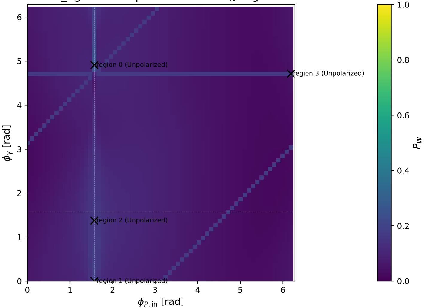
mid_Egamma Unpolarized: max P_W regions
