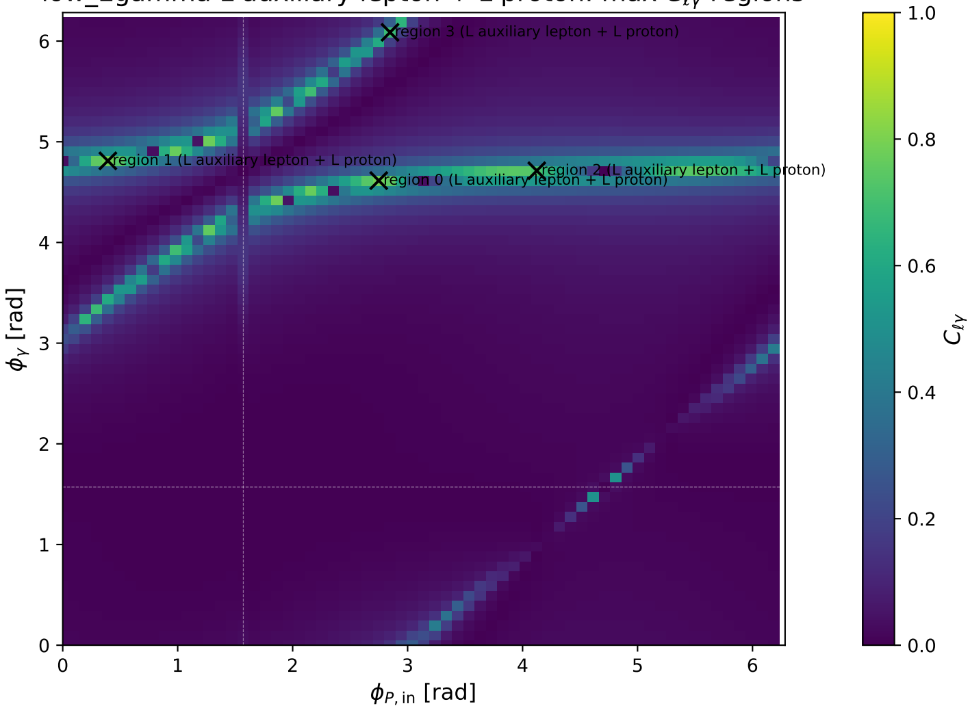
low_Egamma L auxiliary lepton + L proton: max C_{\ell\gamma} regions
