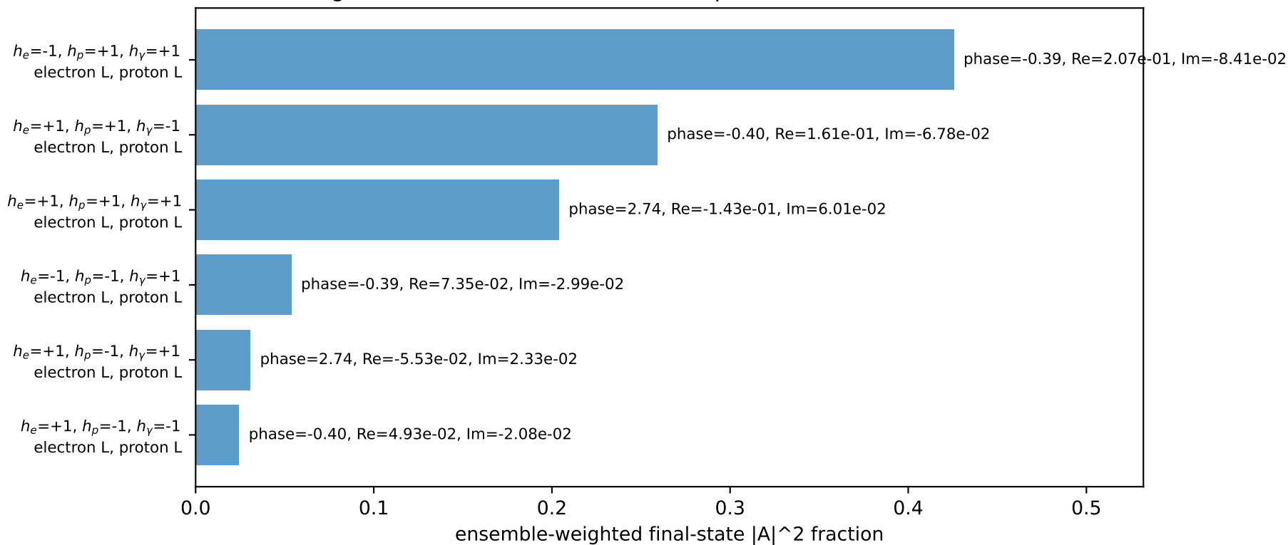
Leading initial-ensemble/final-state components (N=6, retained=99.8%)
