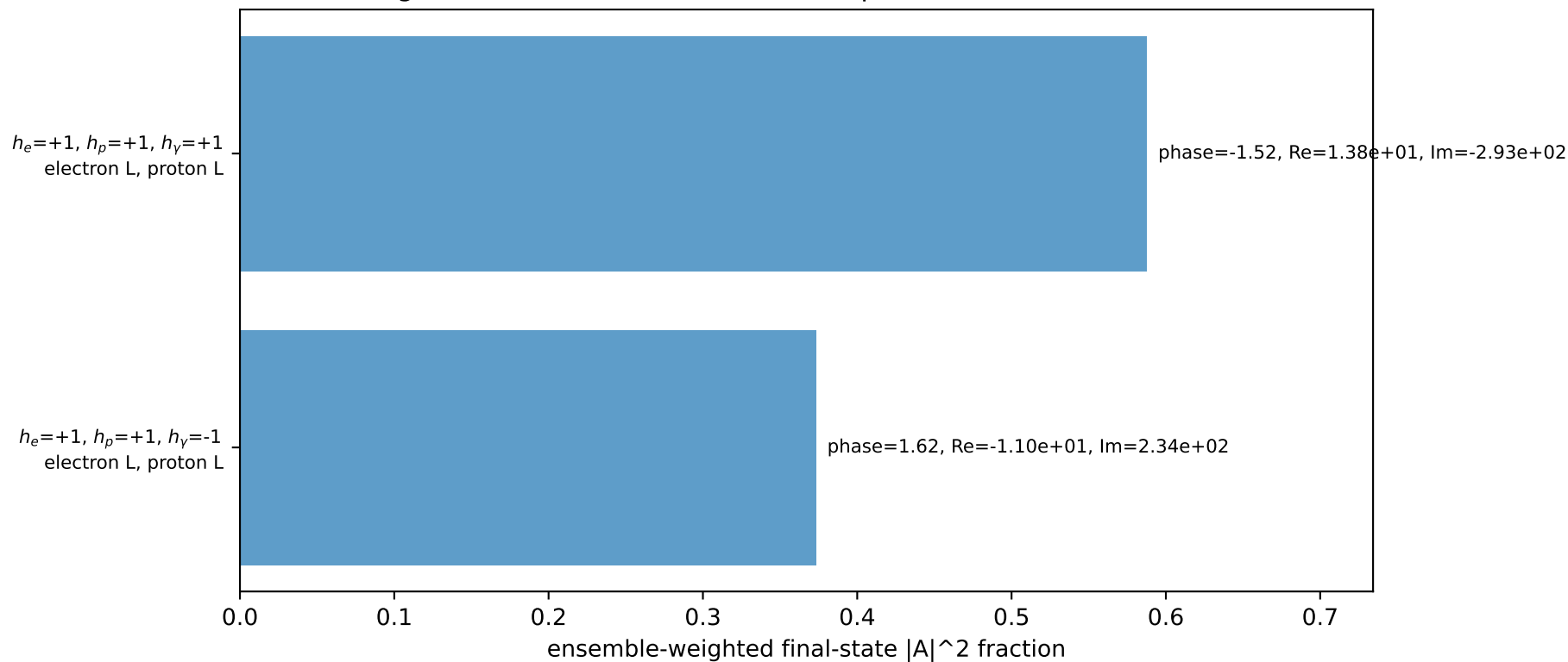
Leading initial-ensemble/final-state components (N=2, retained=96.0%)
