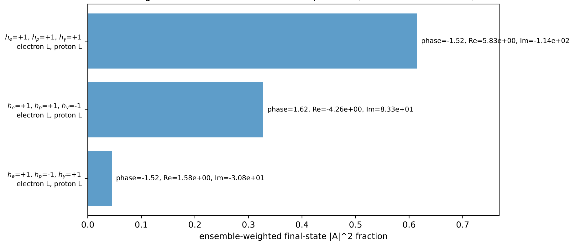
Leading initial-ensemble/final-state components (N=3, retained=98.7%)
