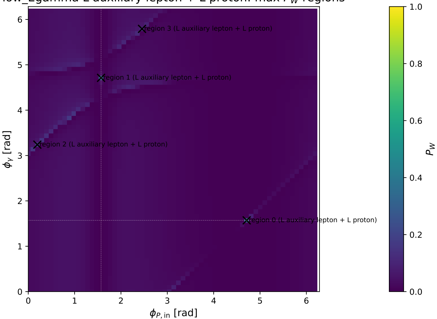
low_Egamma L auxiliary lepton + L proton: max P_W regions
