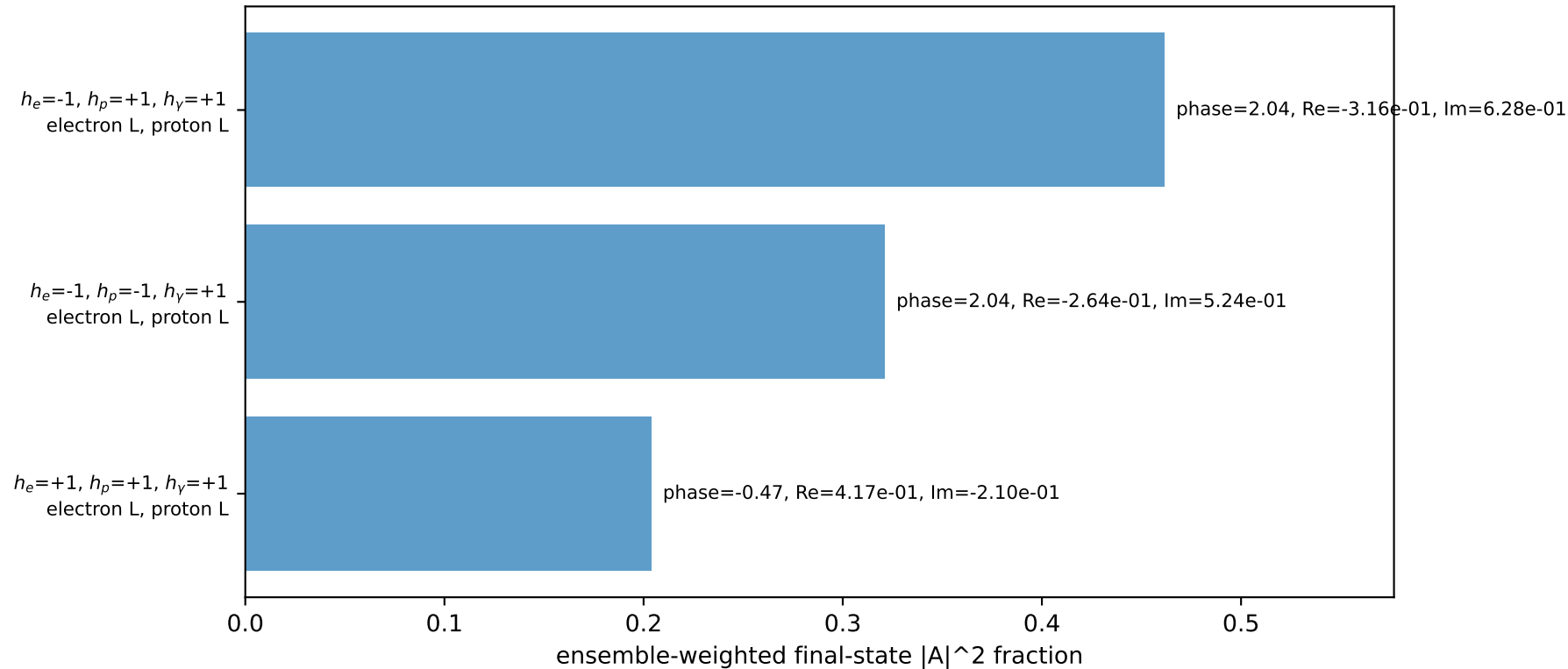
Leading initial-ensemble/final-state components (N=3, retained=98.6%)
