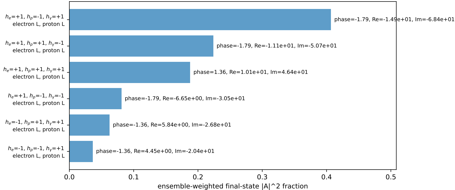
Leading initial-ensemble/final-state components (N=6, retained=99.8%)
