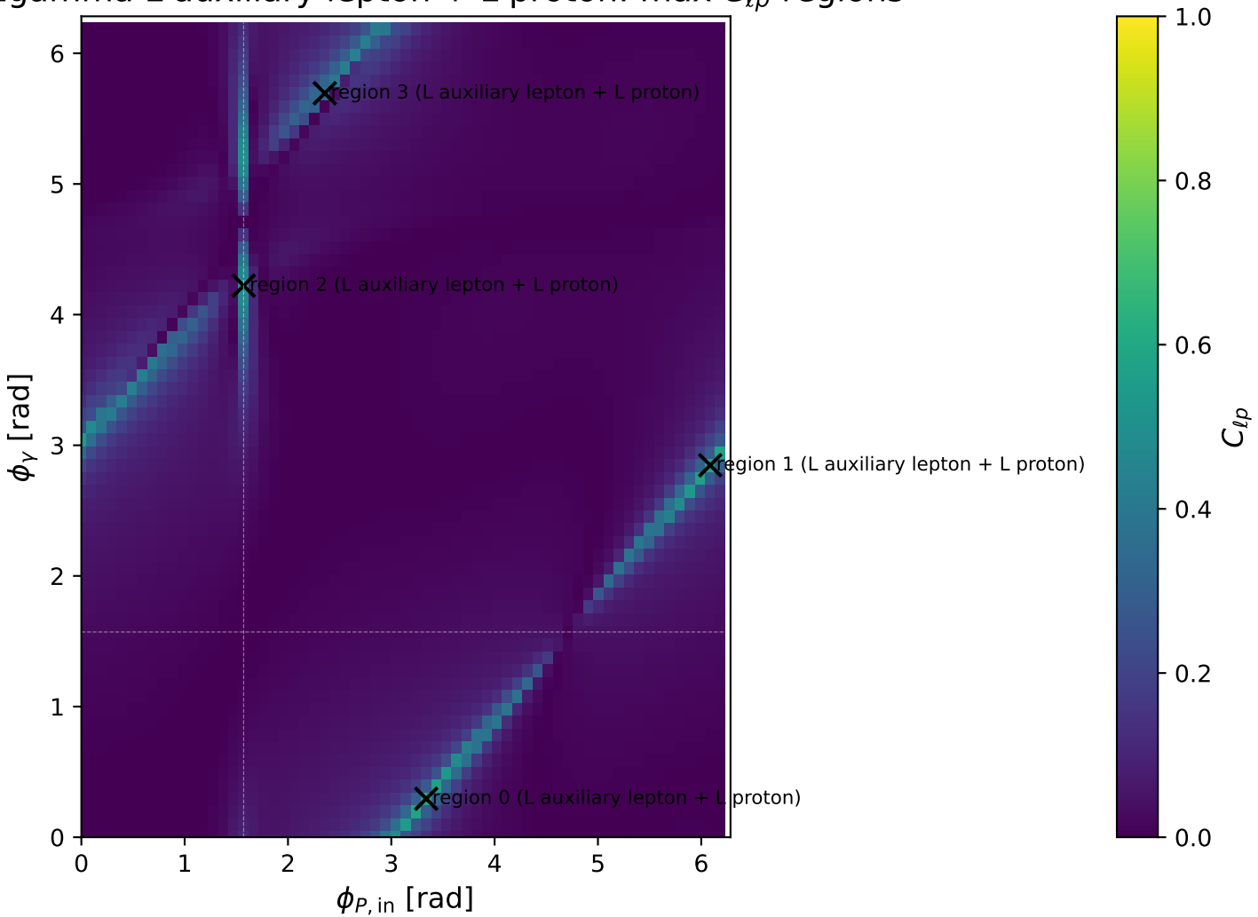
egamma L auxiliary lepton + L proton: max C_{lp} regions
