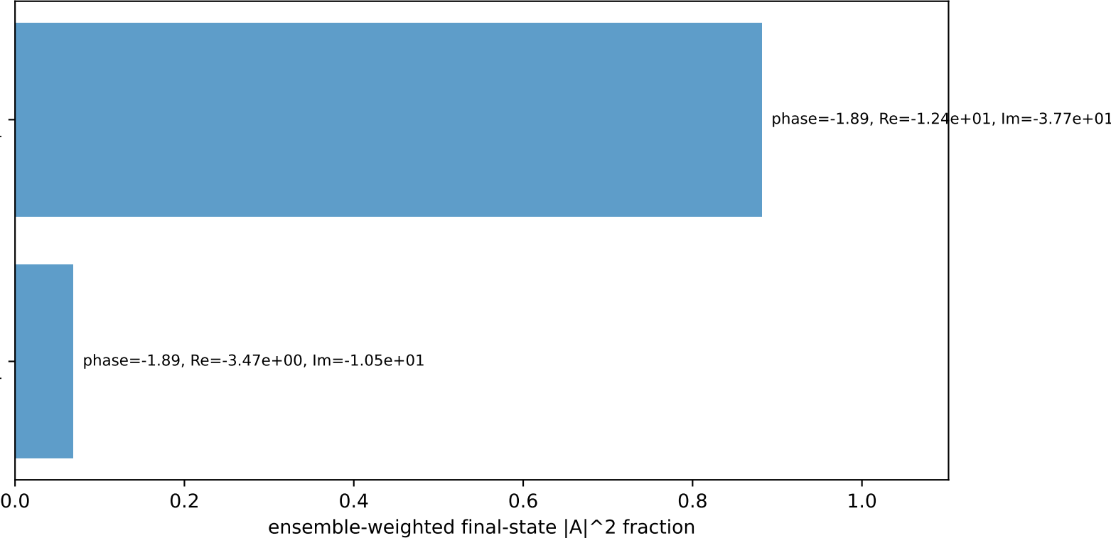
Leading initial-ensemble/final-state components (N=2, retained=95.0%)
