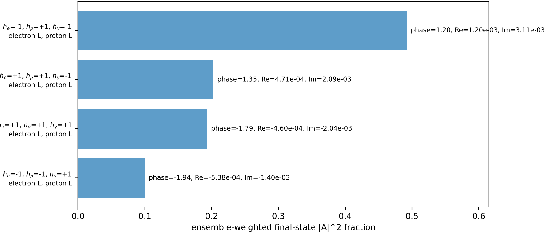
Leading initial-ensemble/final-state components (N=4, retained=98.7%)
