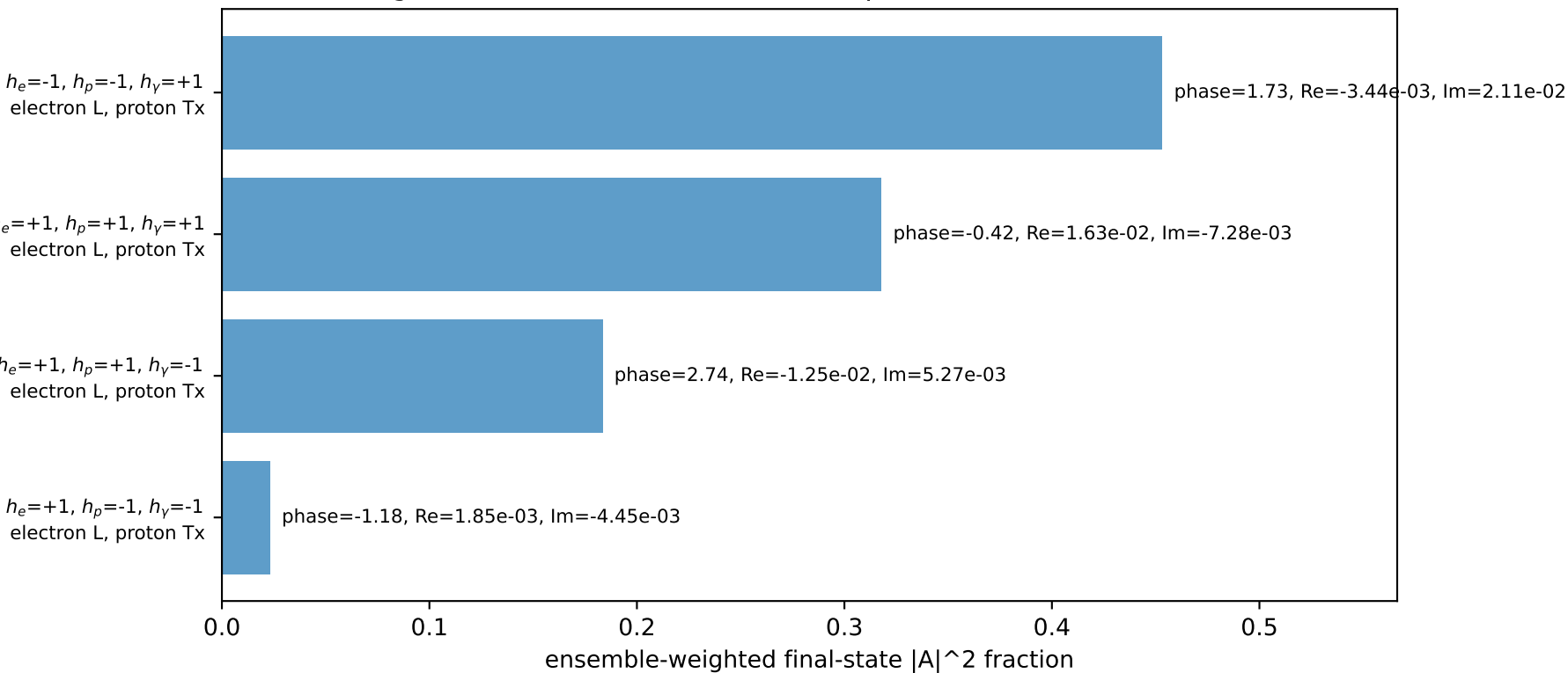
Leading initial-ensemble/final-state components (N=4, retained=97.7%)
