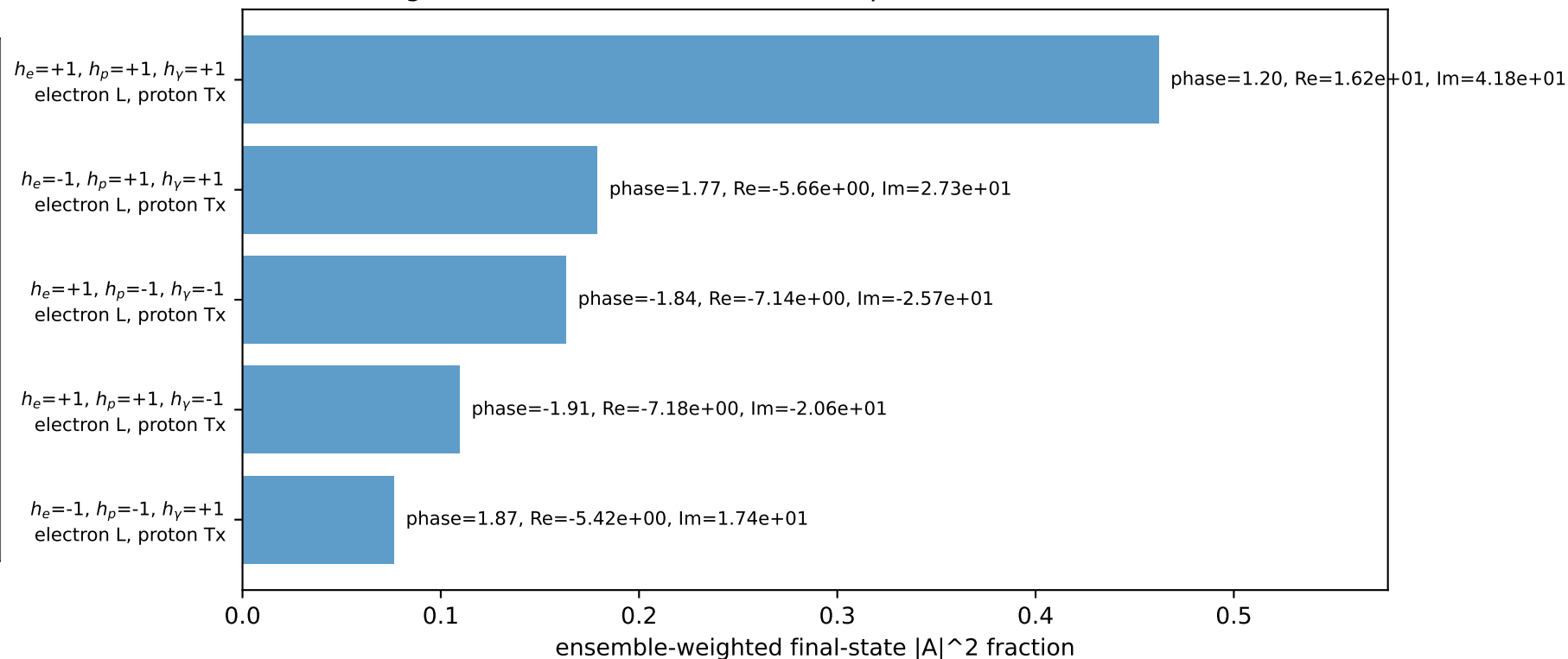
Leading initial-ensemble/final-state components (N=5, retained=99.1%)
