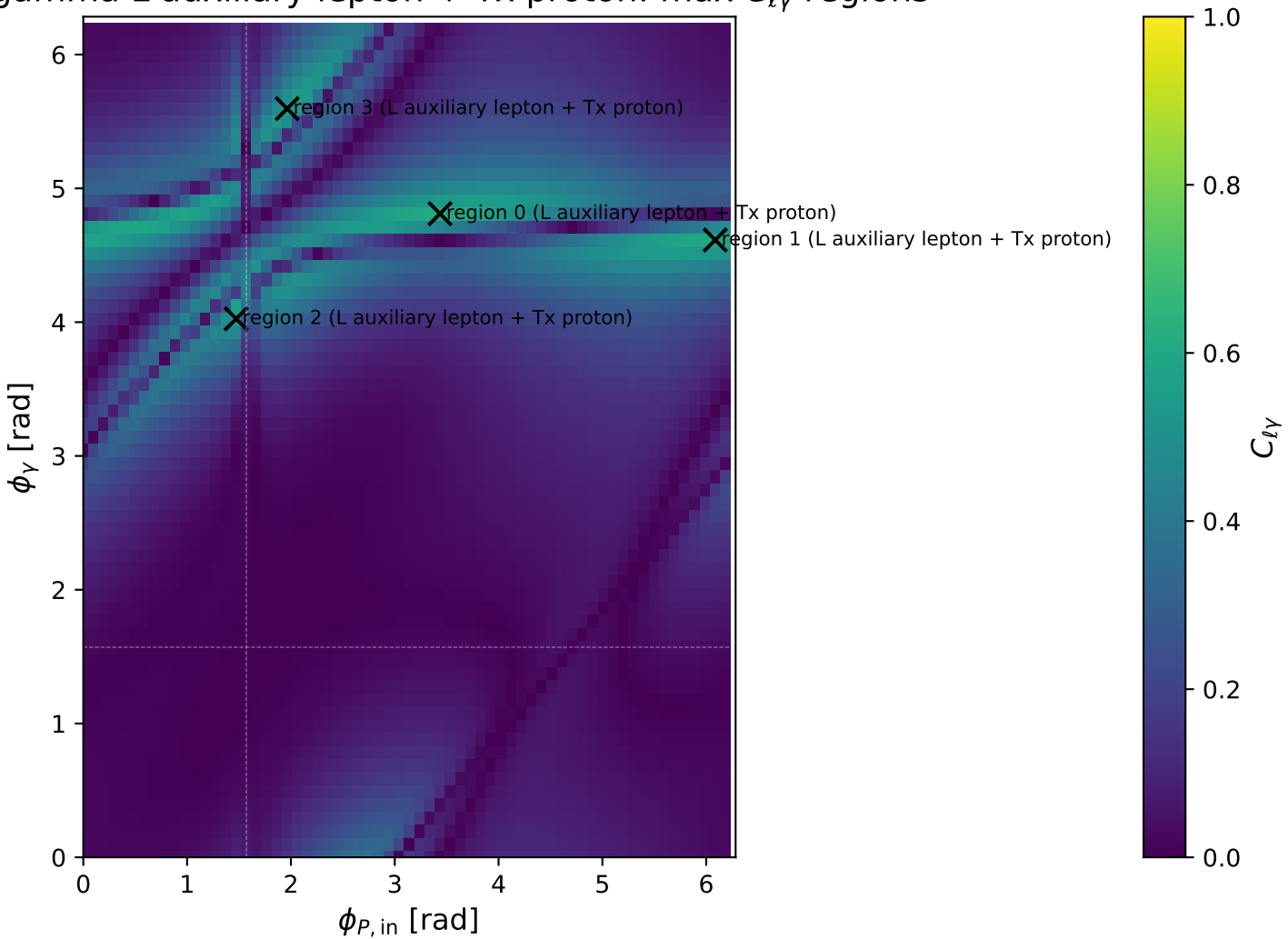
gamma L auxiliary lepton + Tx proton: max C_{\ell\gamma} regions
