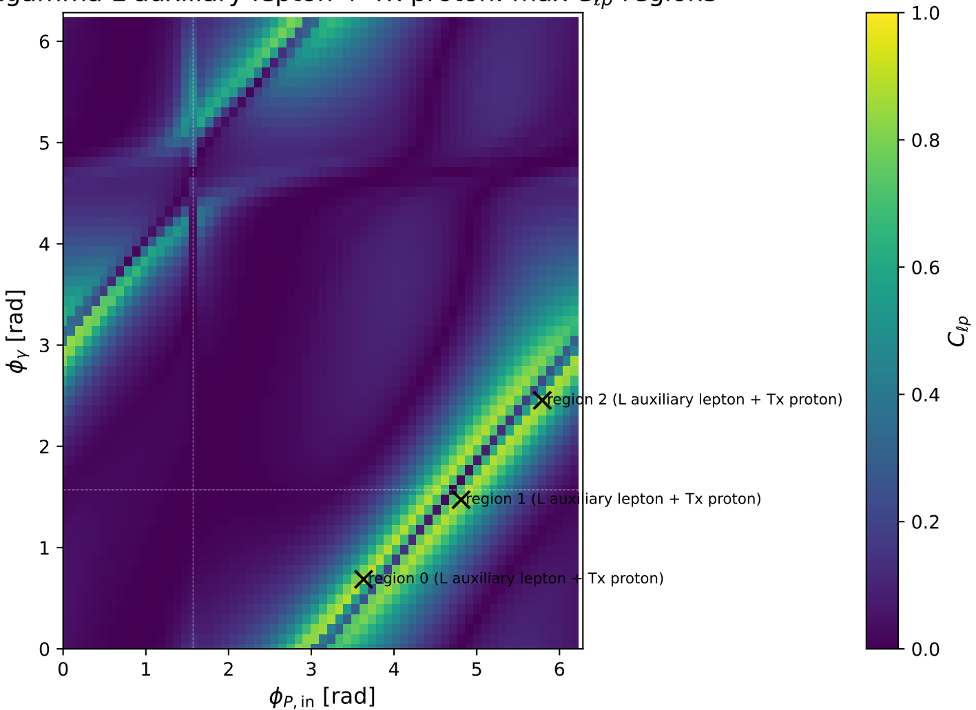
gamma L auxiliary lepton + Tx proton: max C_{lp} regions
