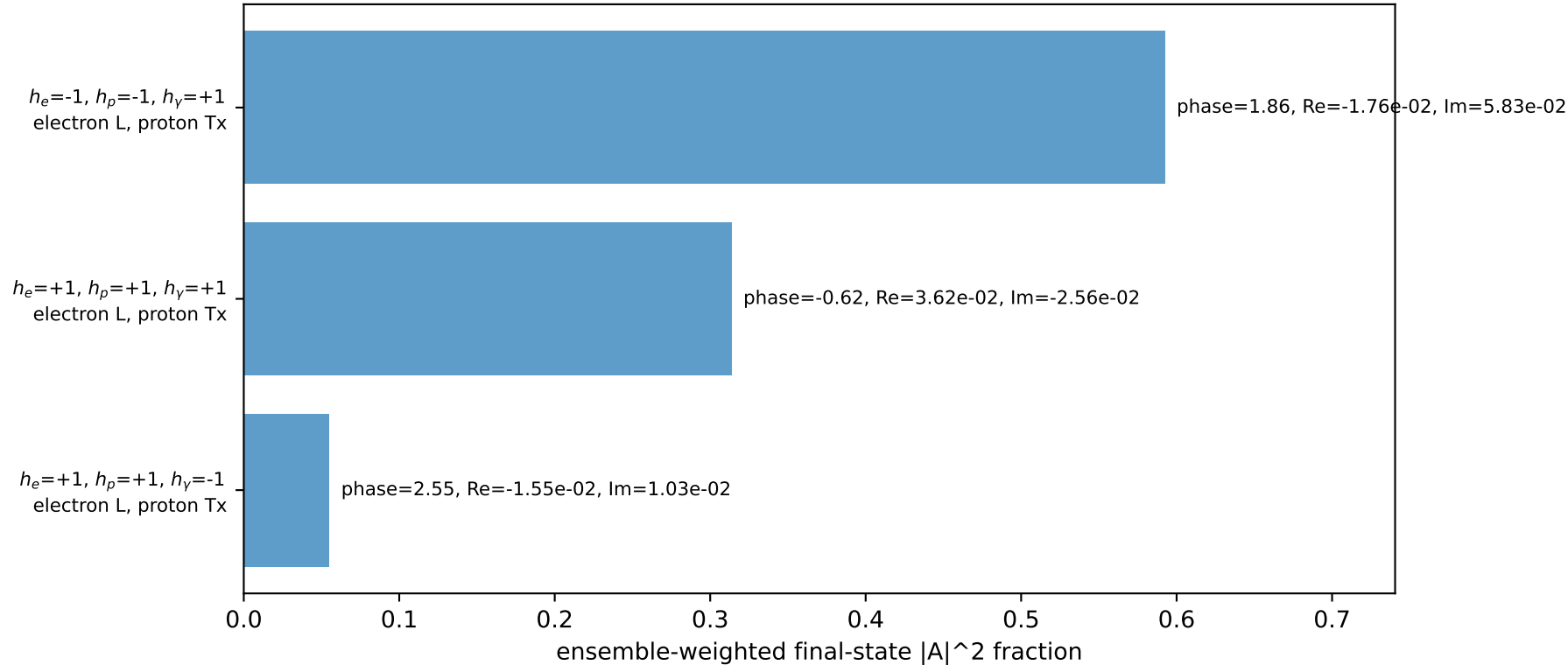
Leading initial-ensemble/final-state components (N=3, retained=96.1%)
